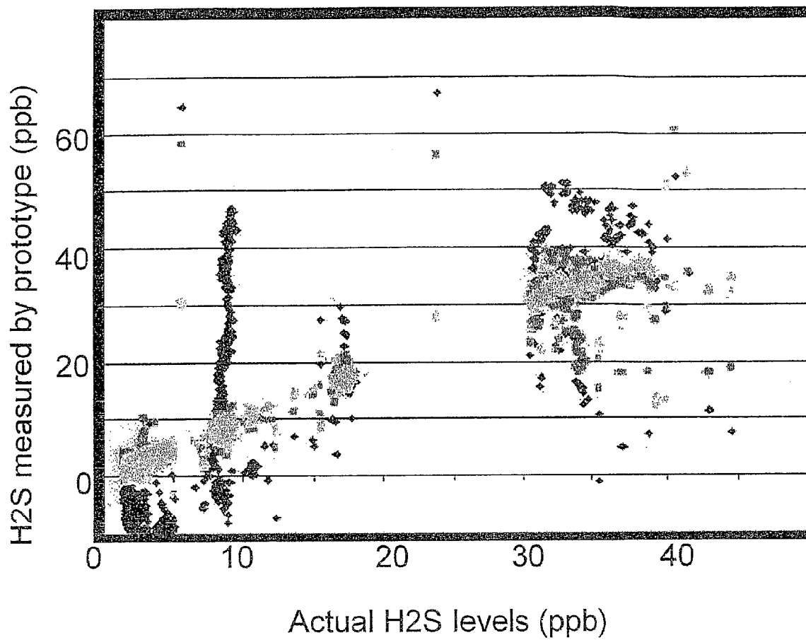
Figure 4: Multiple sensors
