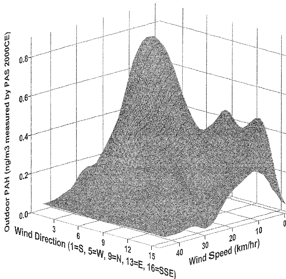
Figure 16: Surface representing mean real-time measures of PAH levels outdoors compared to wind speed and direction for temperatures less than -15 C.
