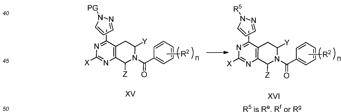
Scheme 6
