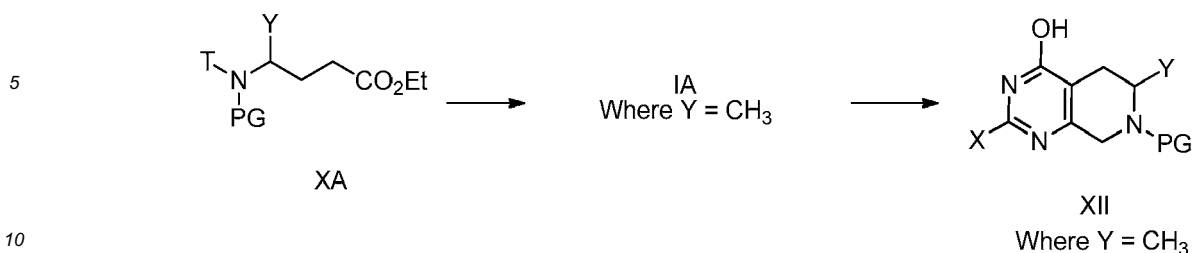
Scheme 4
