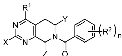
Formula (Ia)
