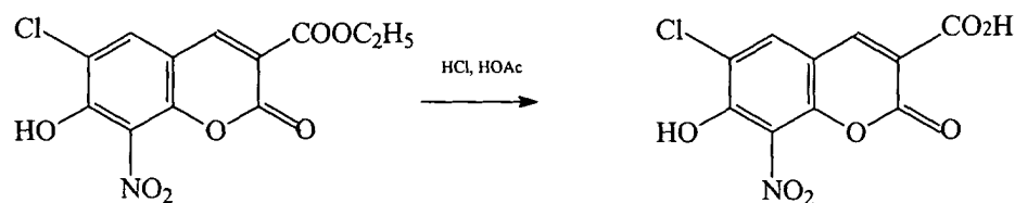
(16) 6-carboxycoumarin
