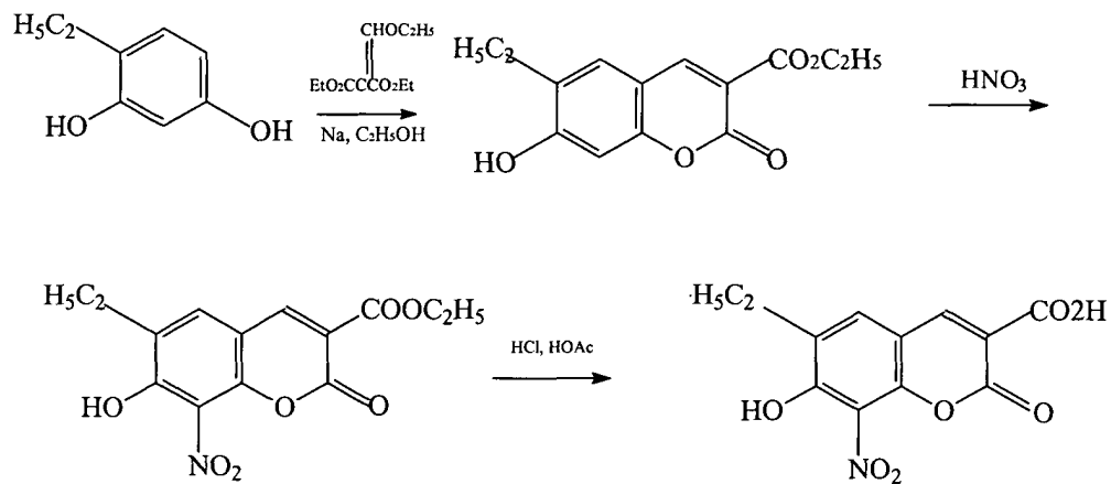
(14) 3-ethoxycarbonyl-6-ethyl-7-hydroxy-8-nitrocoumarin and 3-carboxy-6-ethyl-7-hydroxy-8-nitrocoumarin
