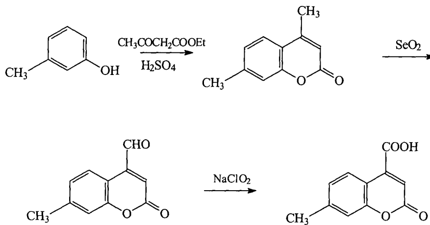
(17) 4-carboxy-7-methylcoumarin
