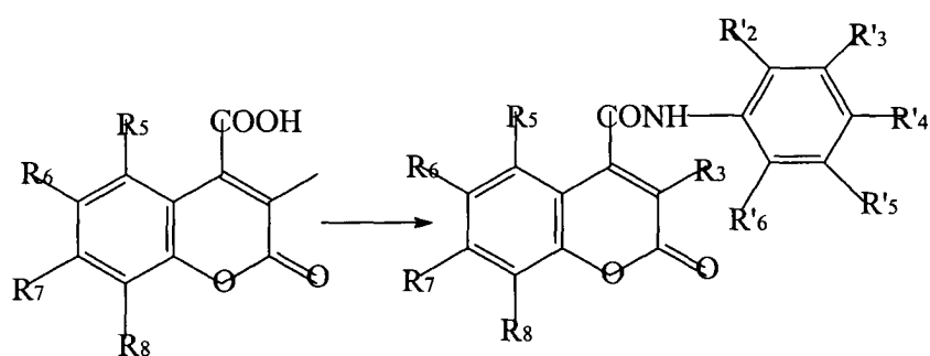
(IIc)
