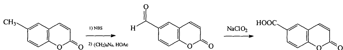
(16) 6-carboxycoumarin
