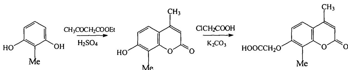
(19) 4, 8-dimethyl-7-carboxymethoxycoumarin
