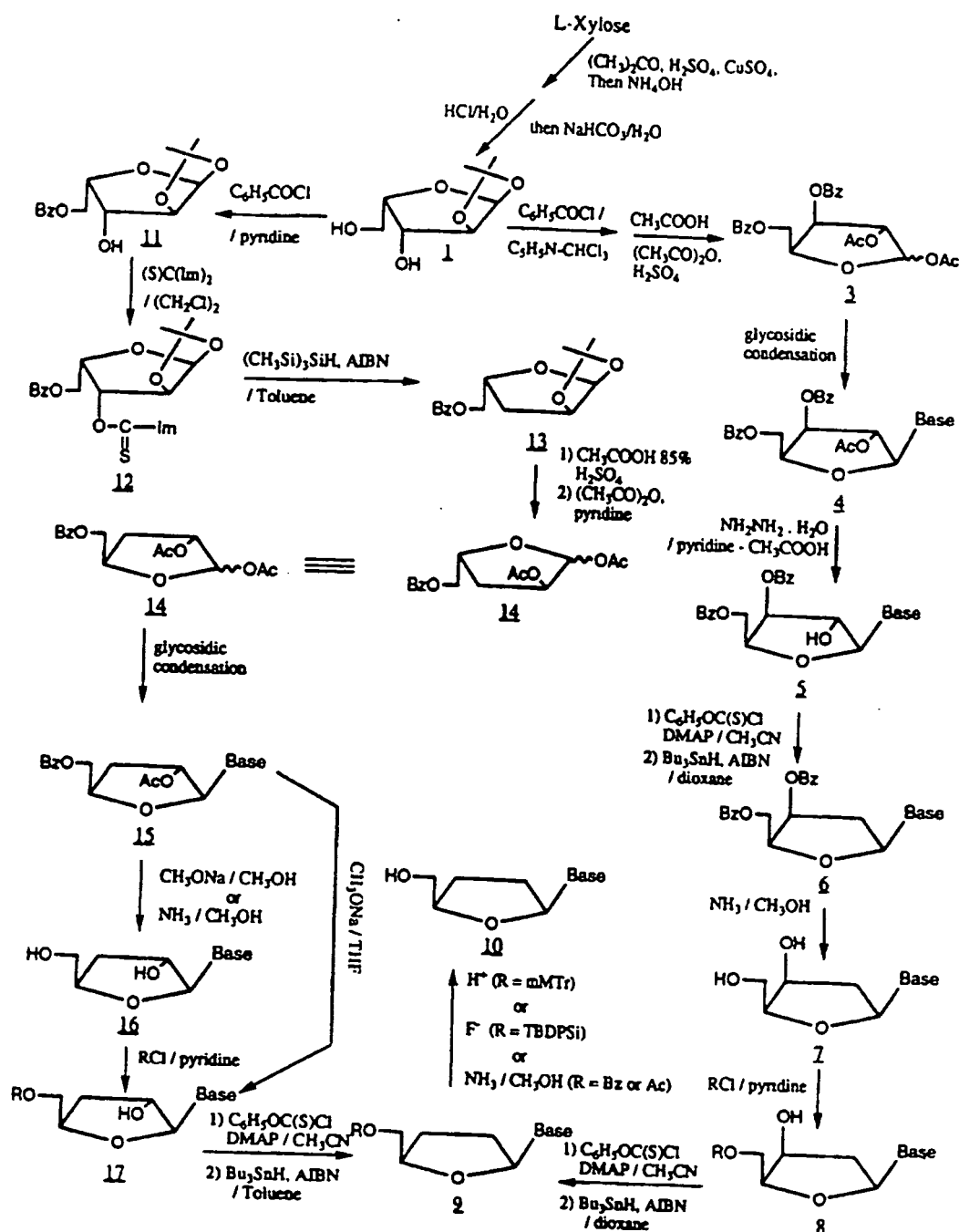
Scheme I: Bases = purines or pyrimidines, éventuellement convenablement protégées; R = Benzoyl (Bz) Acetyl (Ac), monomethoxytrityl (mMTr) or tertiarybutyldiphenylsilyl (TBDPSi)
