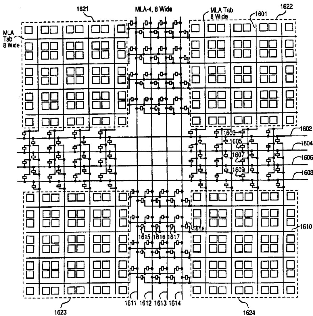
MLA-4 Routing Network - Access and Routing
