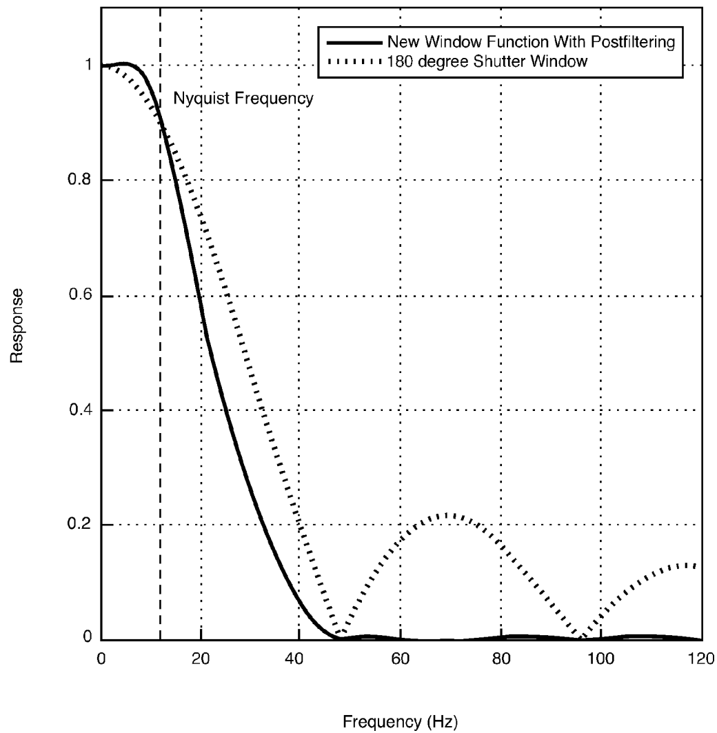
Modulation Transfer Function for Exposure Window With Postfiltering
