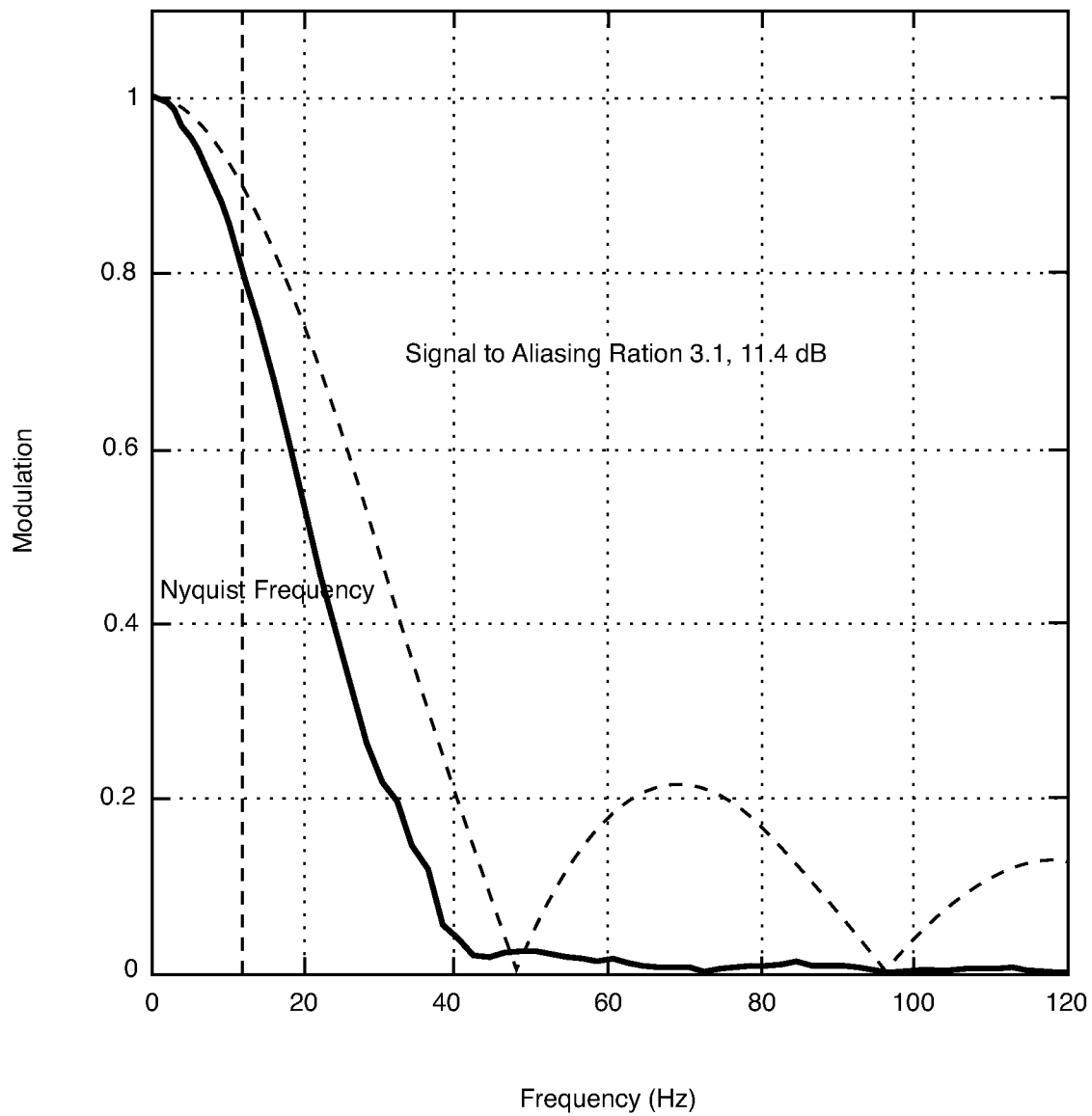
Temporal Modulation Transfer Functions (24 fps, Hamming Window)
