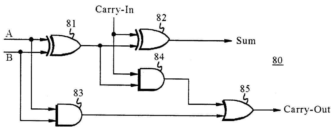
FIG. 5 PRIOR ART
