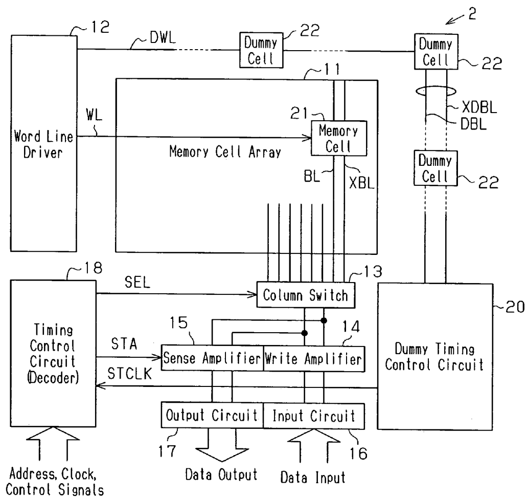
Fig.3(Prior Art)
