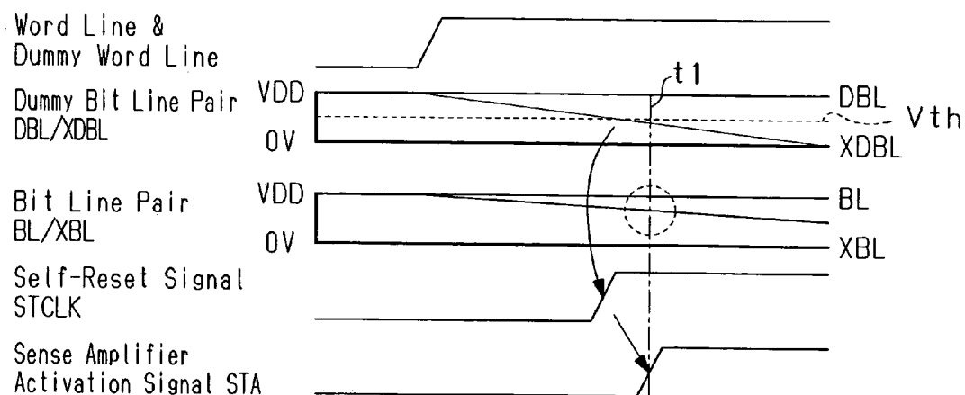
Fig.4B(Prior Art)
