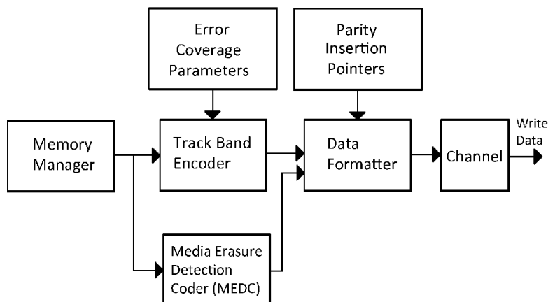
Track Band ECC System – Write flow
