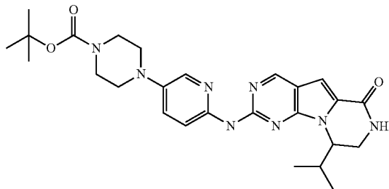
Compound 6
