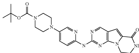
Compound 2
