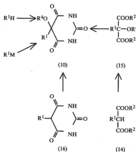
Flowsheet II
