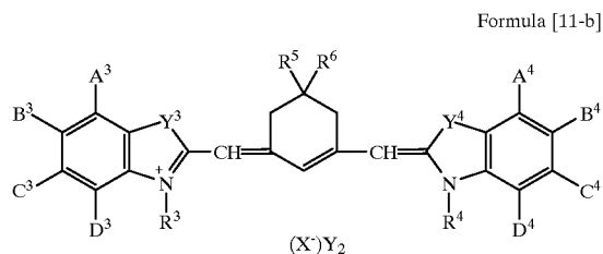
Formula [11-b]
