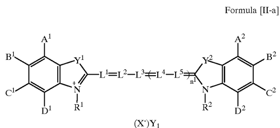
Formula [II-a]
