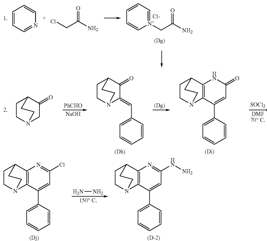
REACTION SCHEME 4
