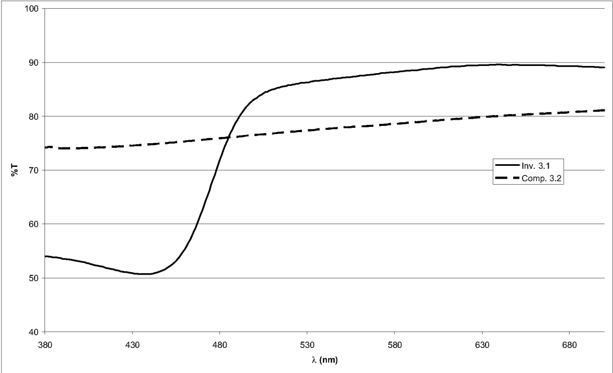
Fig. 4: spectra of samples of Example 3
