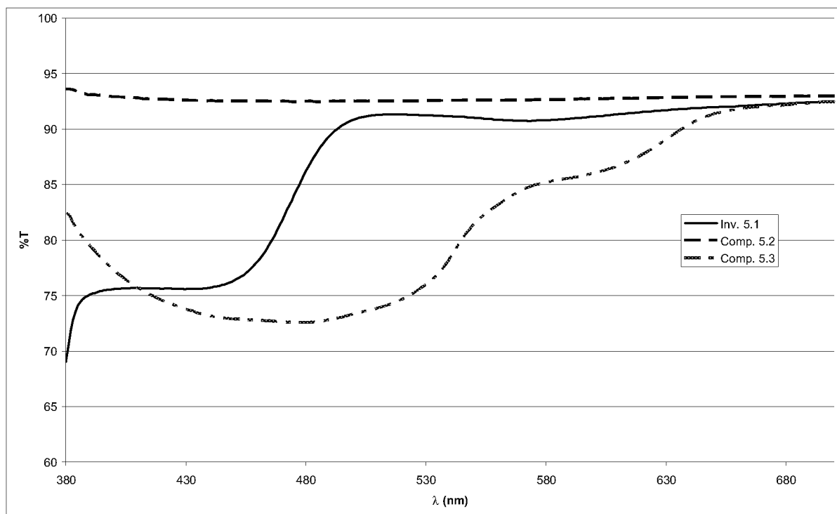
Fig. 6: spectra of samples of Example 5
