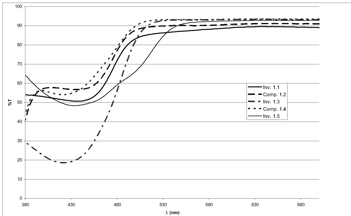
Fig. 1: spectra of samples of Example 1
