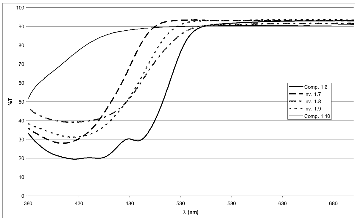
Fig. 2: spectra of samples of Example 1
