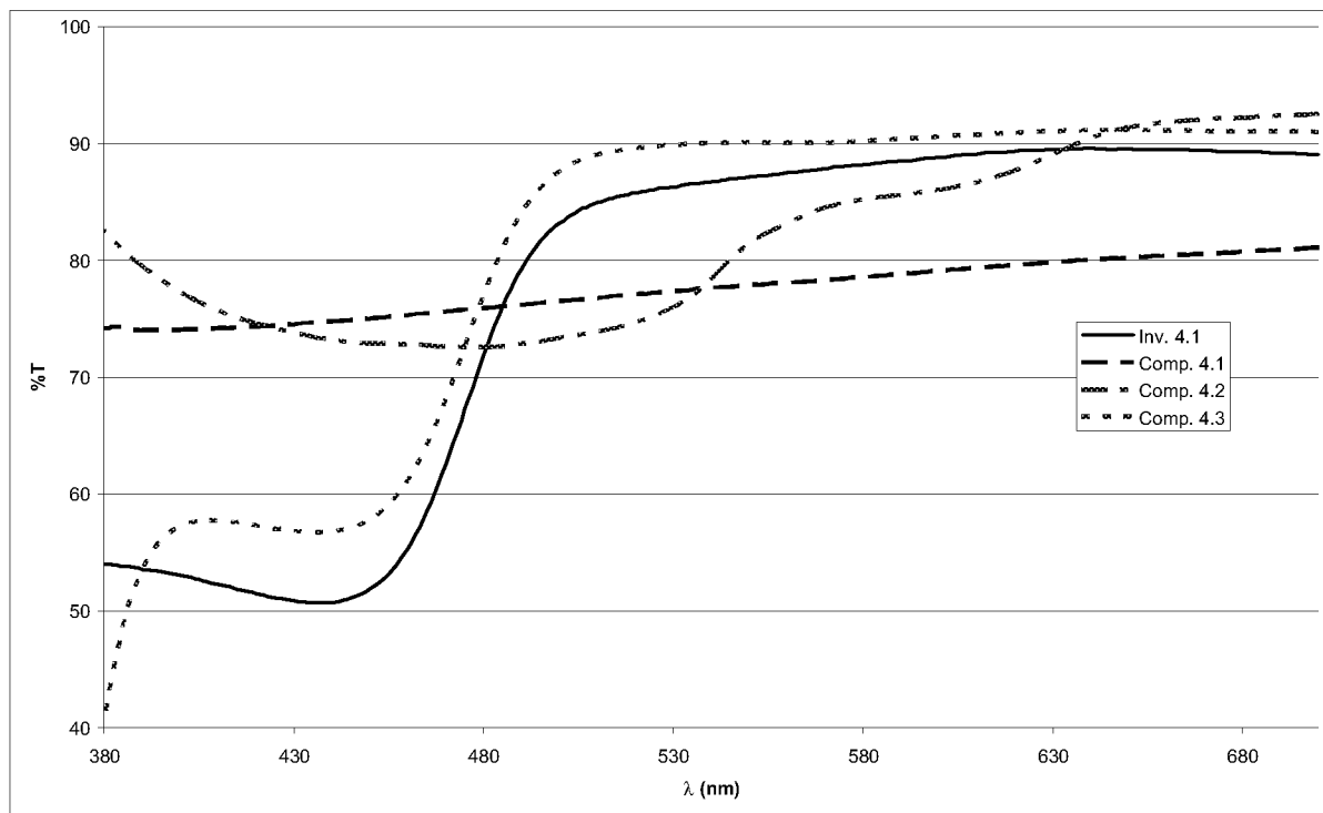
Fig. 5: spectra of samples of Example 4
