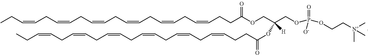
(Compound 438)
