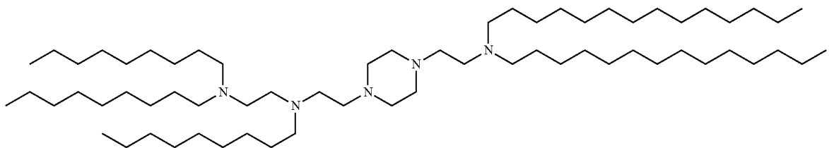
(Compound 253)
