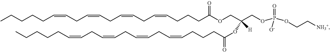
(Compound 443)
