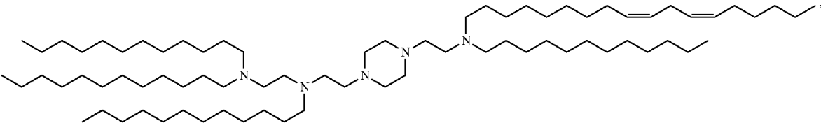
(Compound 259)
