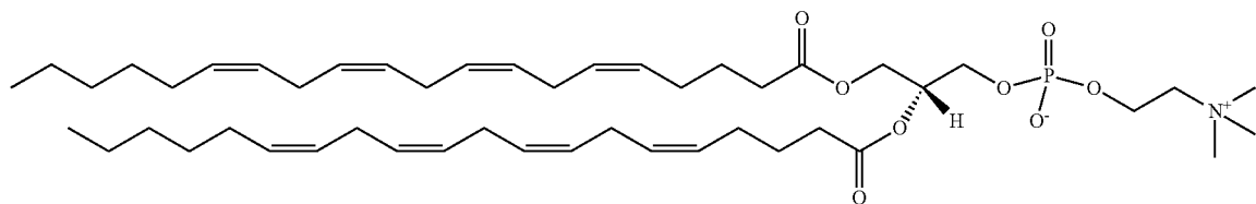
(Compound 436)
