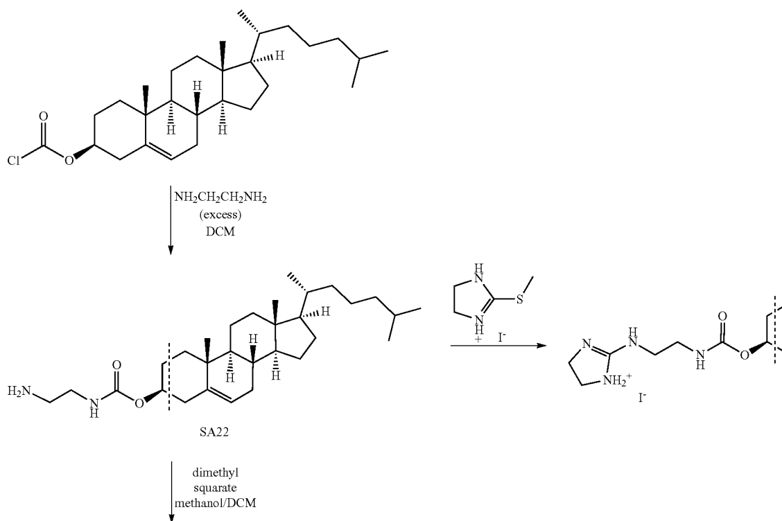
Scheme 5
