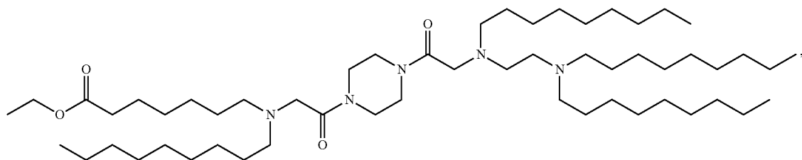
(Compound 285)
