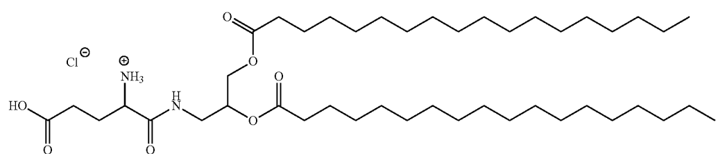
Compound 461a
