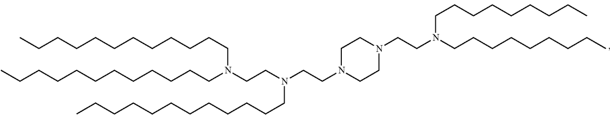
(Compound 255)
