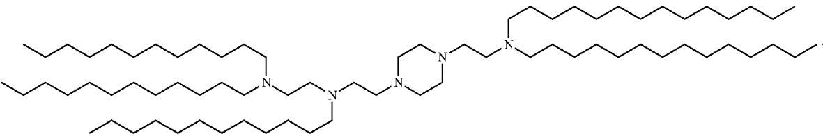
(Compound 259)
