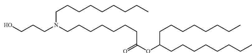
(Compound 7)
