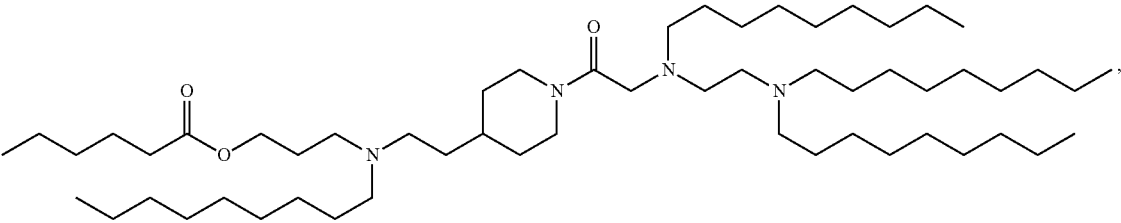
(Compound 294)
