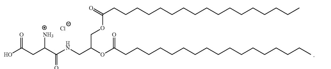
Compound 463b
