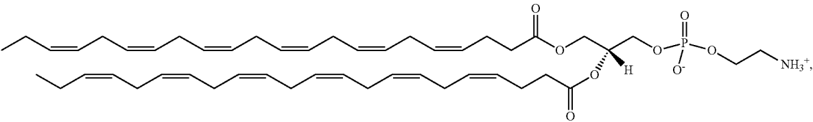
(Compound 443)
