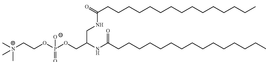
(Compound 453)
