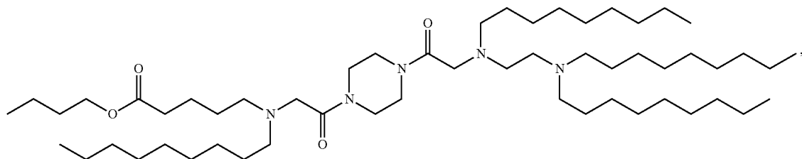
(Compound 288)
