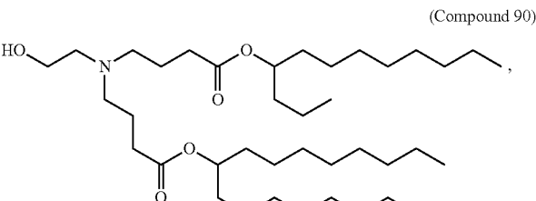
(Compound 92)
