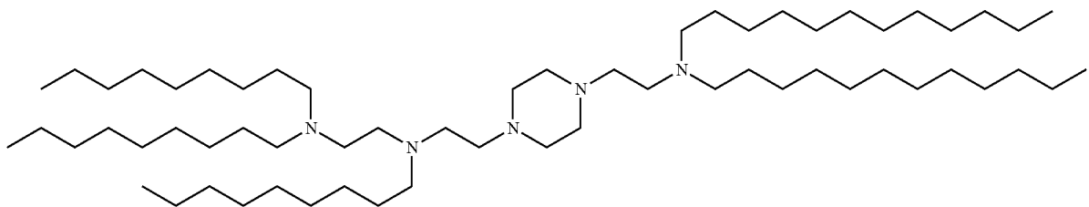
(Compound 252)
