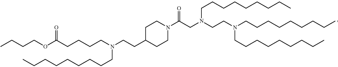
(Compound 293)
