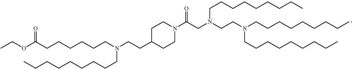
(Compound 290)
