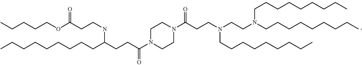
(Compound 294)
