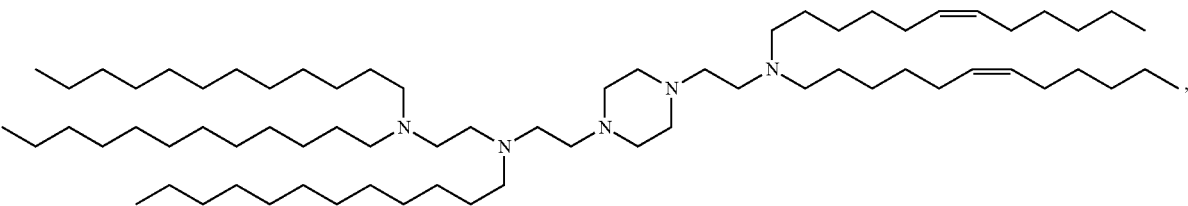
(Compound 258)
