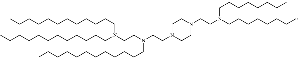
(Compound 254)
