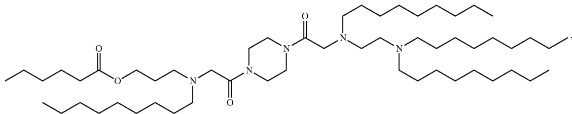
(Compound 289)
