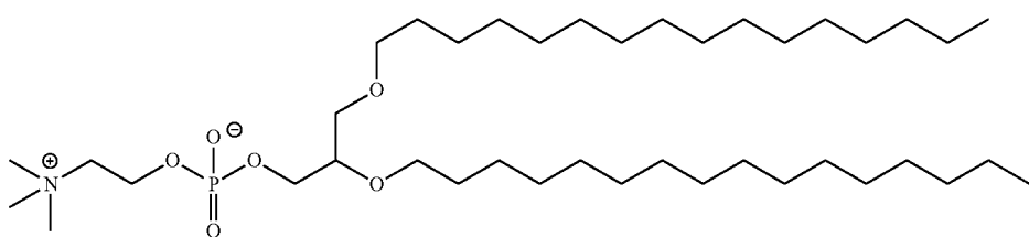
(Compound 449)
