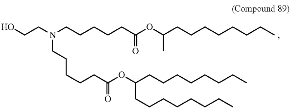
(Compound 91)
