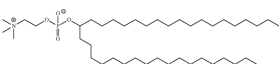
(Compound 452)
