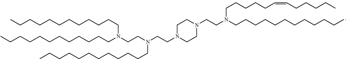
(Compound 257)
