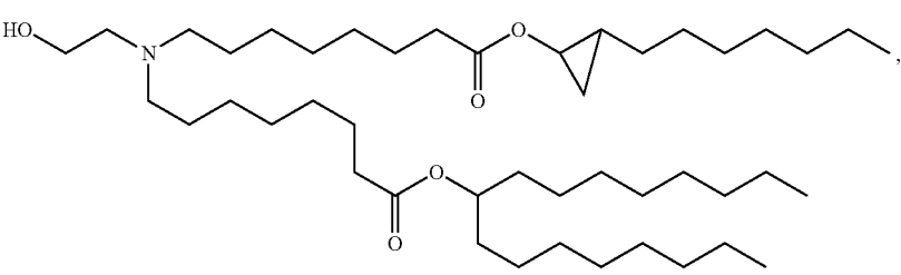
(Compound 89)
