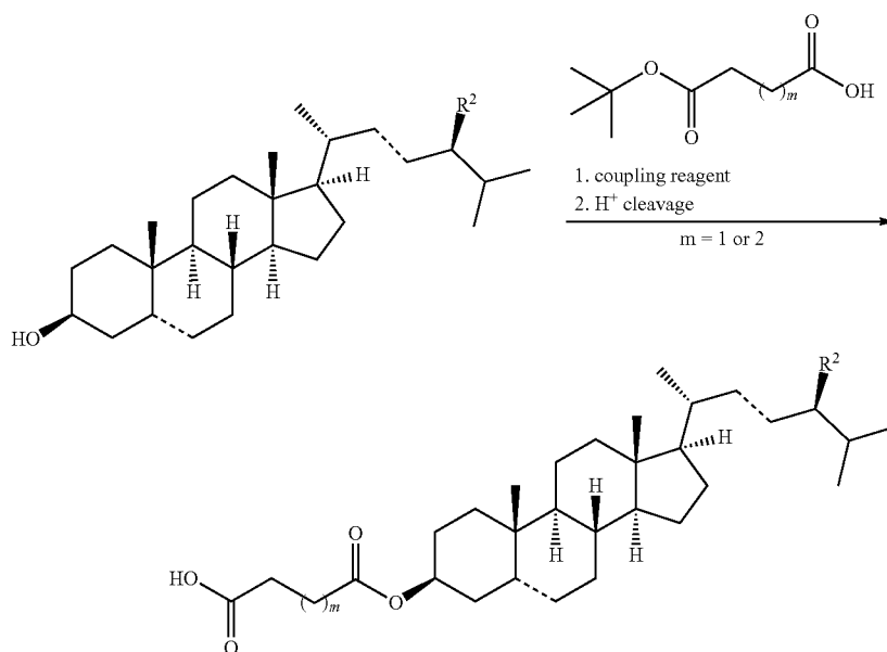
Scheme 8
