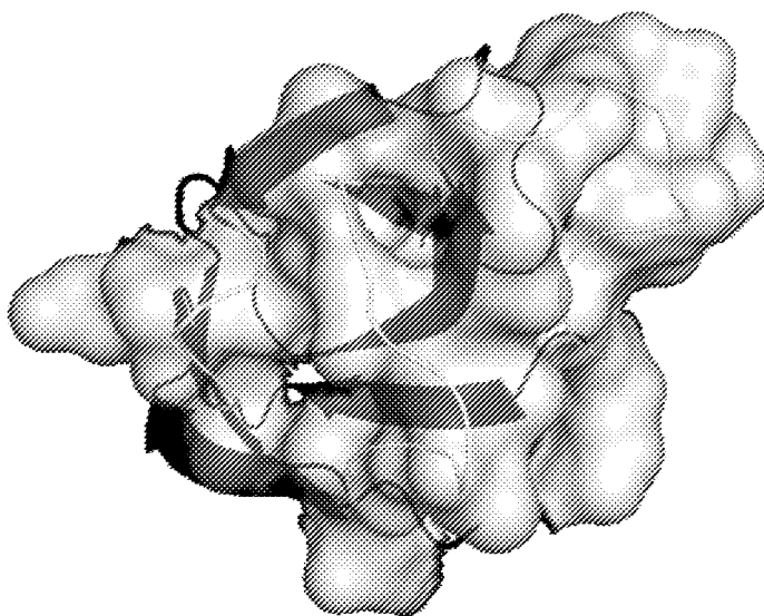
FnIII 10 Top Side Surface = 1834 Å 2
