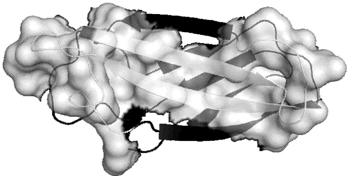
FnIII 10 Cradle Surface = 2457 Å 2
