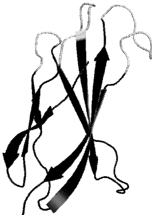
FnIII 10 Top Side
