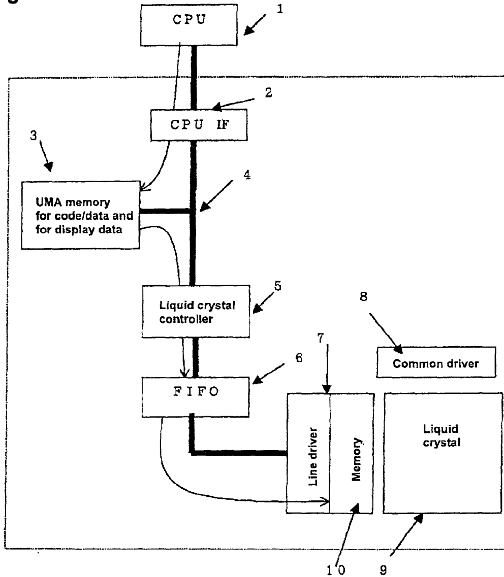
Liquid crystal display apparatus
