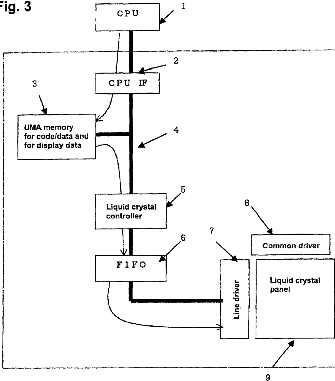
Liquid crystal display apparatus
