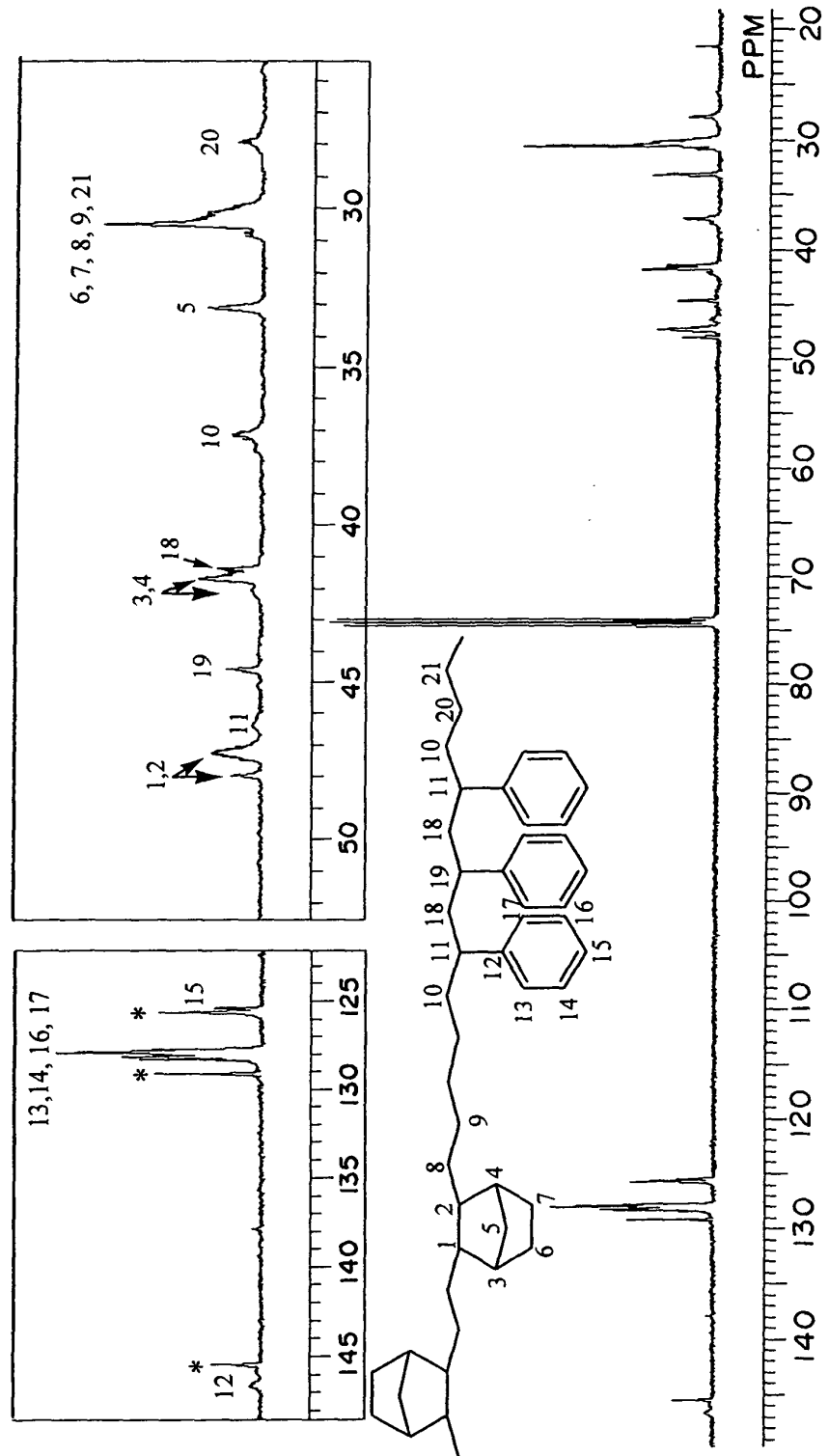
^{13}\text{C} -NMR spectrum chart of the terpolymer of ethylene, norbornene, and styrene obtained in Example 99
