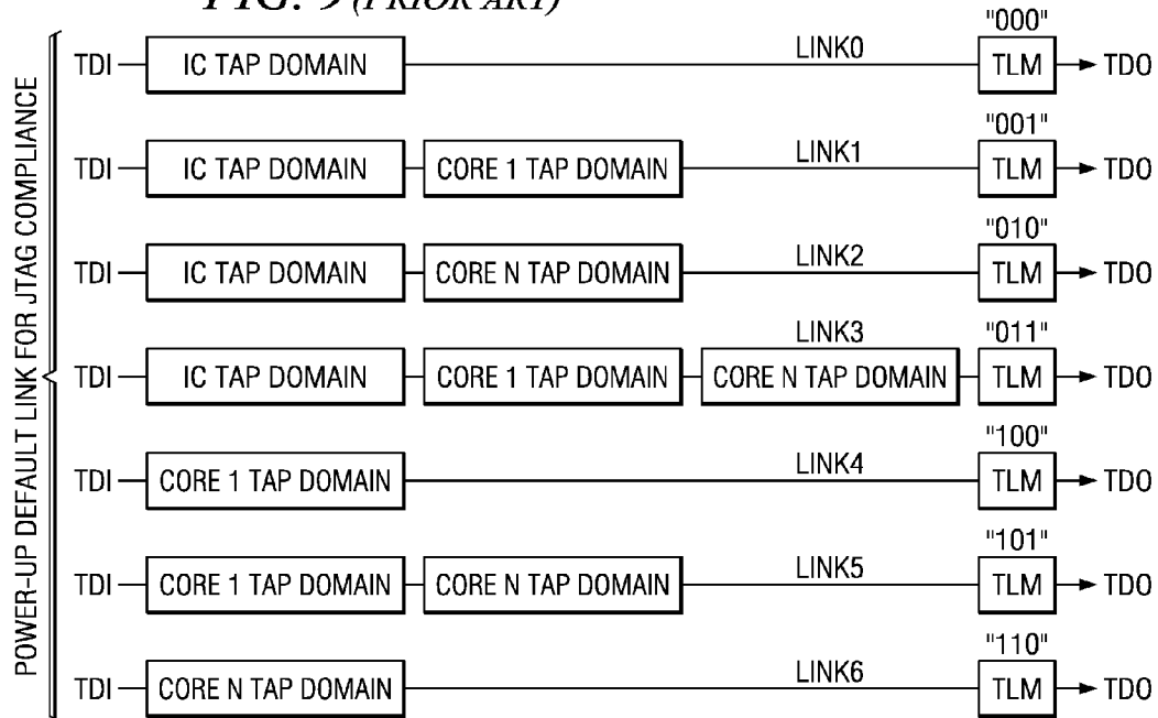
FIG. 9 (PRIOR ART)
