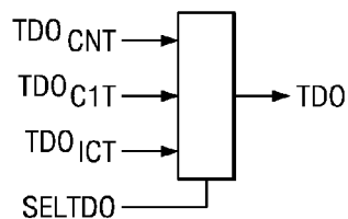
FIG. 7 (PRIOR ART)
