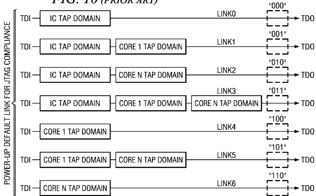
FIG. 10 (PRIOR ART)
