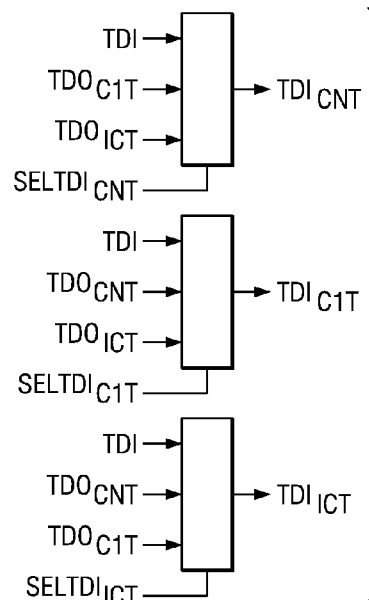
FIG. 6 (PRIOR ART)
