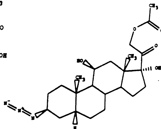
3 \beta -AZIDO-5 \beta -PREGNAN-11 \beta , 17 \alpha ,21-TRIOL-20-ONE-21-ACETATE
