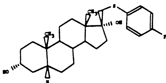
20-(4-FLUOROPHENYL)THIO-21-NOR- PREGNAN-3 \alpha , 17 \alpha -DIOL
