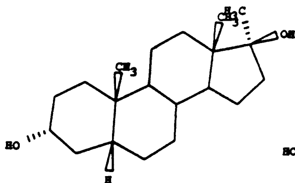
17 \alpha -METHYL-5 \beta -ANDROSTAN- 3 \alpha ,17 \beta -DIOL
