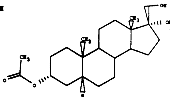
21-NOR-5β-PREGNAN-3α,17α,20-TRIOL-3-ACETATE
