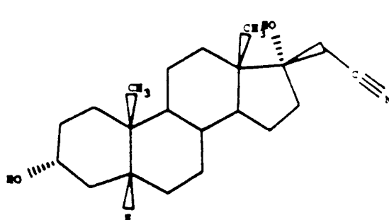
20-CYANO-21-NOR-5 \beta -PREGNAN-3 \alpha ,17 \alpha - DIOL
