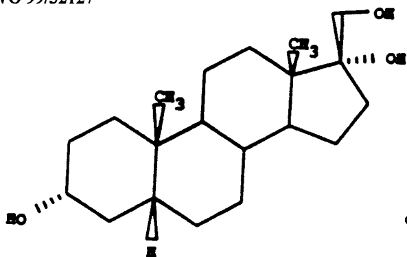
21-NOR-5β-PREGNAN-3α,17α,20-TRIOL
