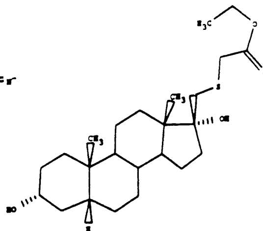
20-(CARBETHOXYMETHYL)THIO-21-NOR-5 \beta - PREGNAN-3 \alpha , 17 \alpha -DIOL
