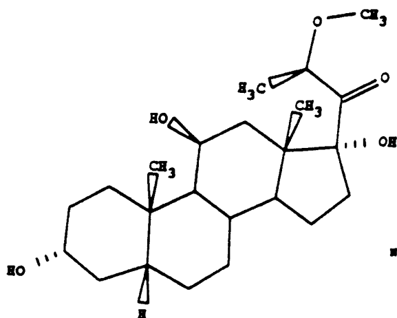
21-METHYL-5 \beta -PREGNAN-3 \alpha ,11 \beta ,17 \alpha , 21-TETROL-20-ONE 21-METHYL ETHER
