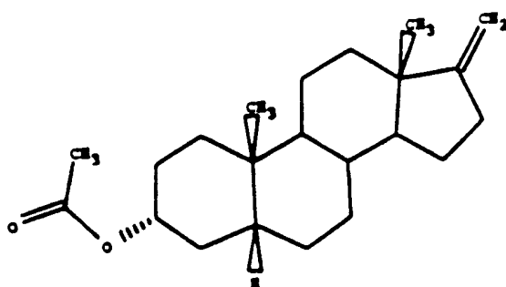
21-NOR-5 \beta -PREGN-17(20)-EN- 3 \alpha -OL-3-ACETATE
