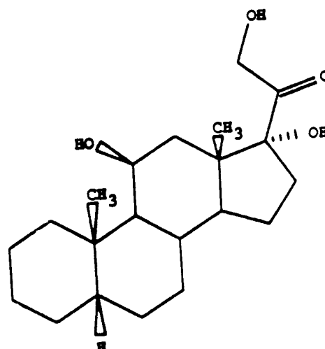
5 \beta -PREGNAN-11 \beta ,17 \alpha ,21-TRIOL-20-ONE
