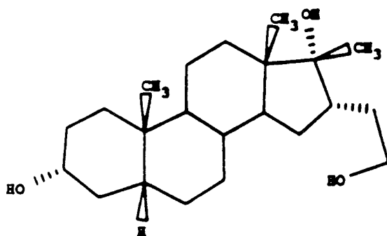
16 \alpha -(2-HYDROXYETHYL)-17 \beta -METHYL- 5 \beta -ANDROSTAN-3 \alpha ,17 \alpha -DIOL
