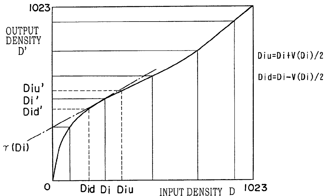
FIG. 6C EVALUATION-VALUE CORRECTION DATA AFTER CORRECTION
