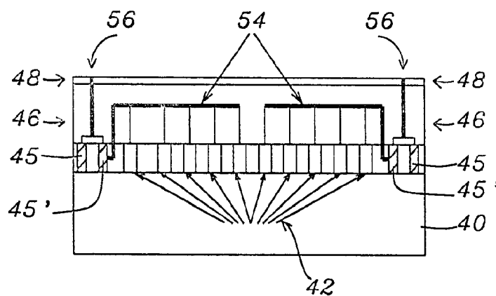
FIG. 2 - Prior Art
