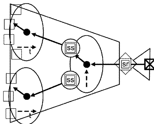
Figure 11: Example single Processing Resource Instance scheduling hierarchy
