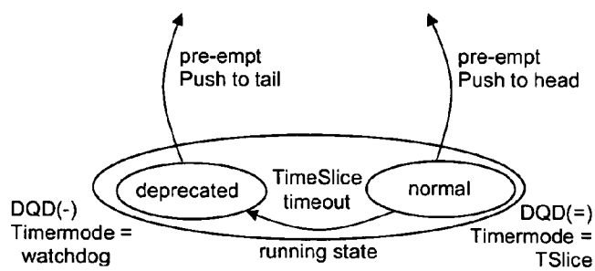
Figure 24: Task priority delta diagram
