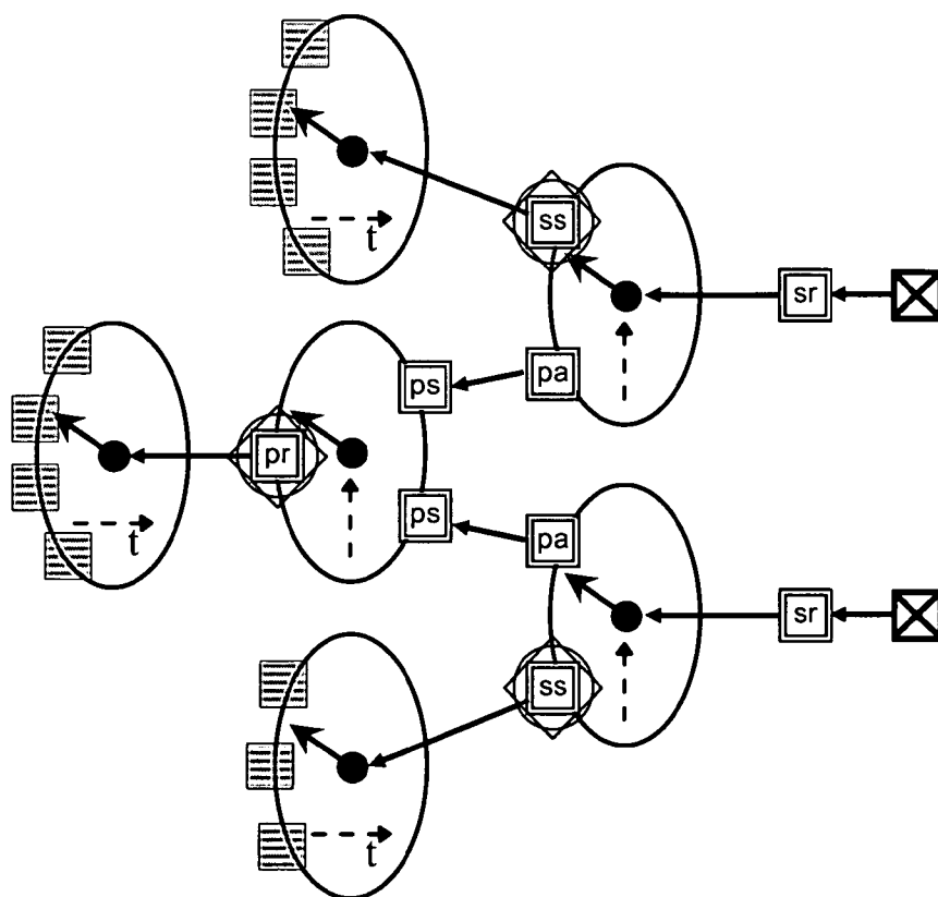
Figure 8: A typical processing resource pool
