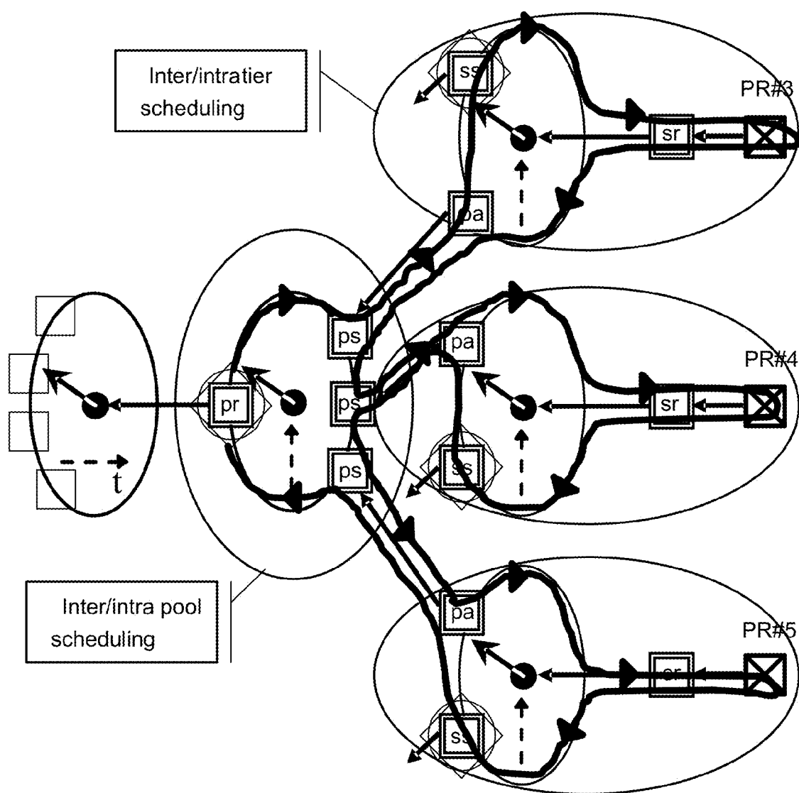
Figure 65: Iterating pool distribution tiers in inter-pool scheduling
