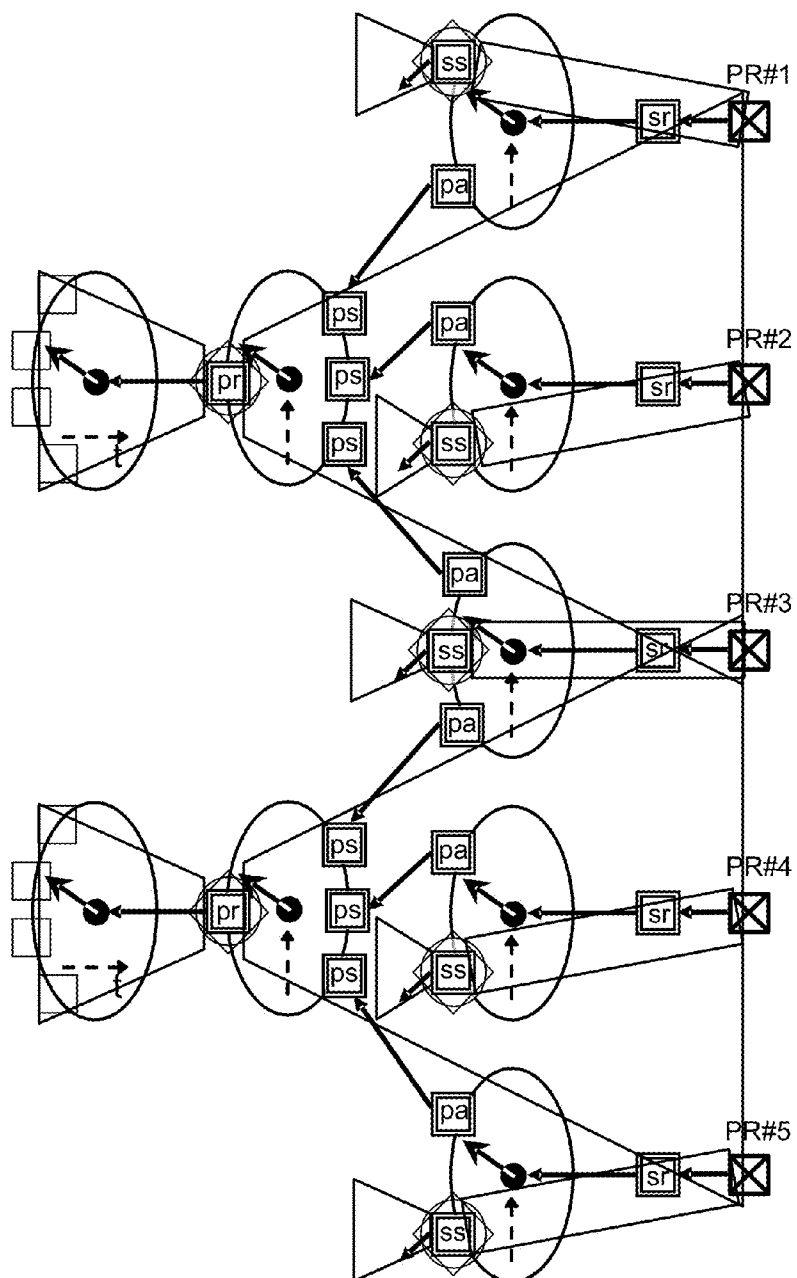
Figure 15 : A 5 processor configuration with two distribution pools
