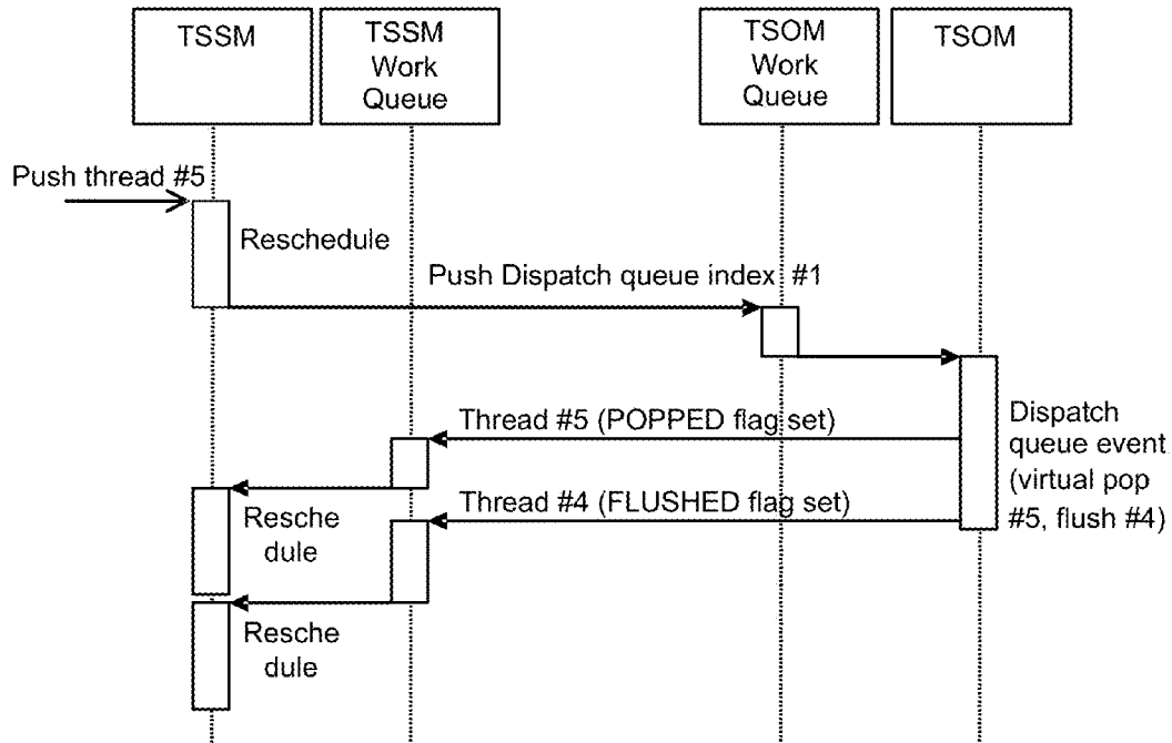
Figure 72: Push event TSOM, TSSM interaction
