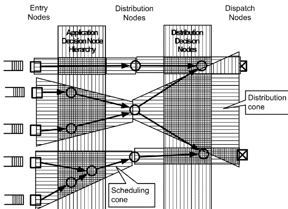
Figure 5: Conceptual scheduling structure
