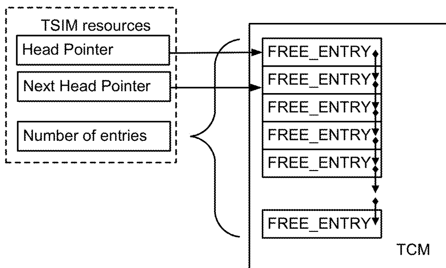
Figure 48: TSIM internal architecture
