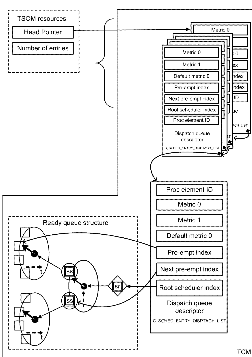
Figure 58: TSOM internal architecture
