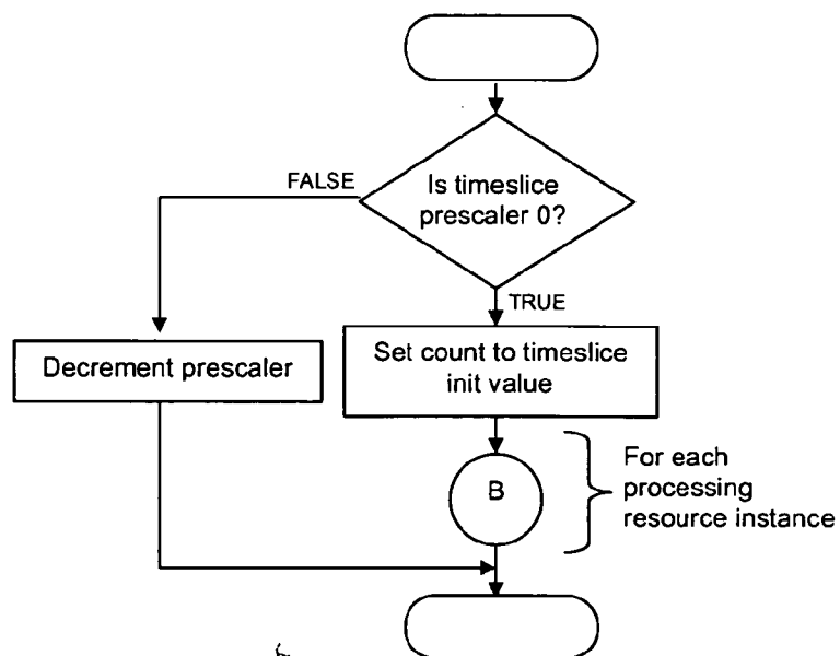
Figure 45: Timeslice control
