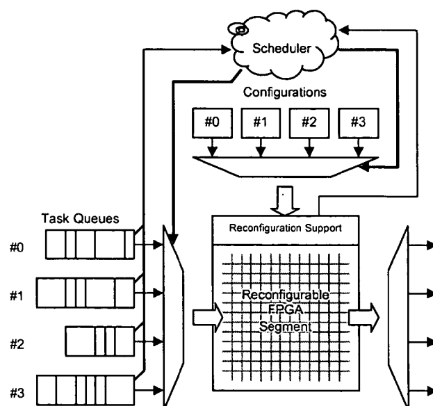
Figure 30: Reconfiguration Management Architecture
