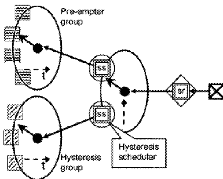
Figure 33: Example hysteresis scheduling configuration
