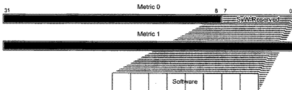
Figure 9: Task descriptor metrics
