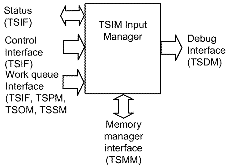
Figure 47: TSIM primary IO
