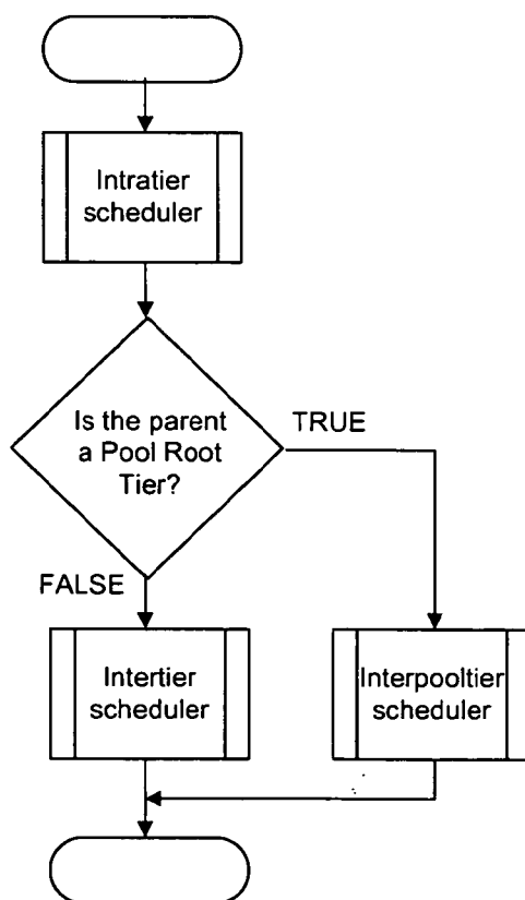
Figure 60: Reschedule flow
