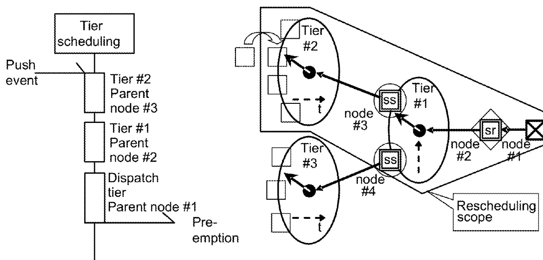
Figure 19: Rescheduling scope for a simple push operation
