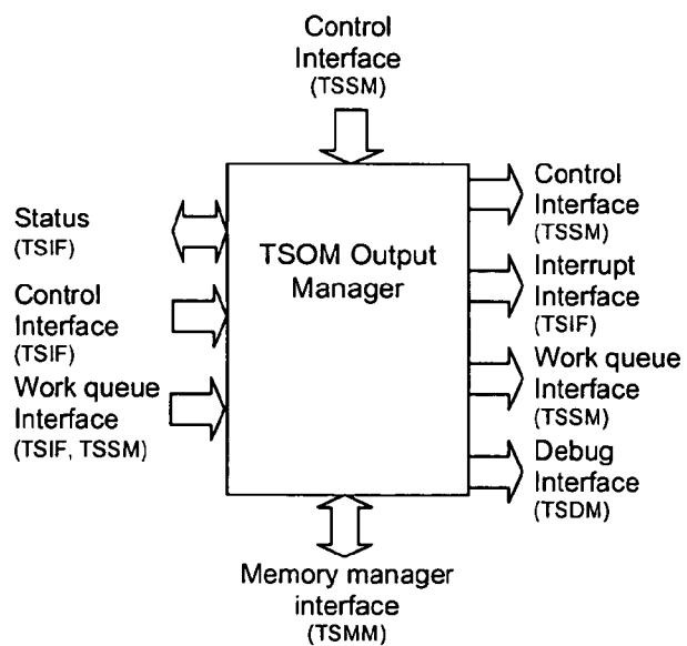
Figure 57: TSOM primary IO
