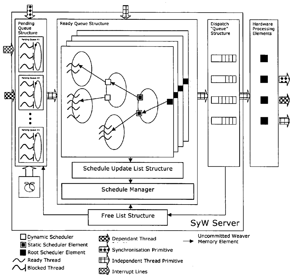
Figure 39: SystemWeaver server conceptual diagram
