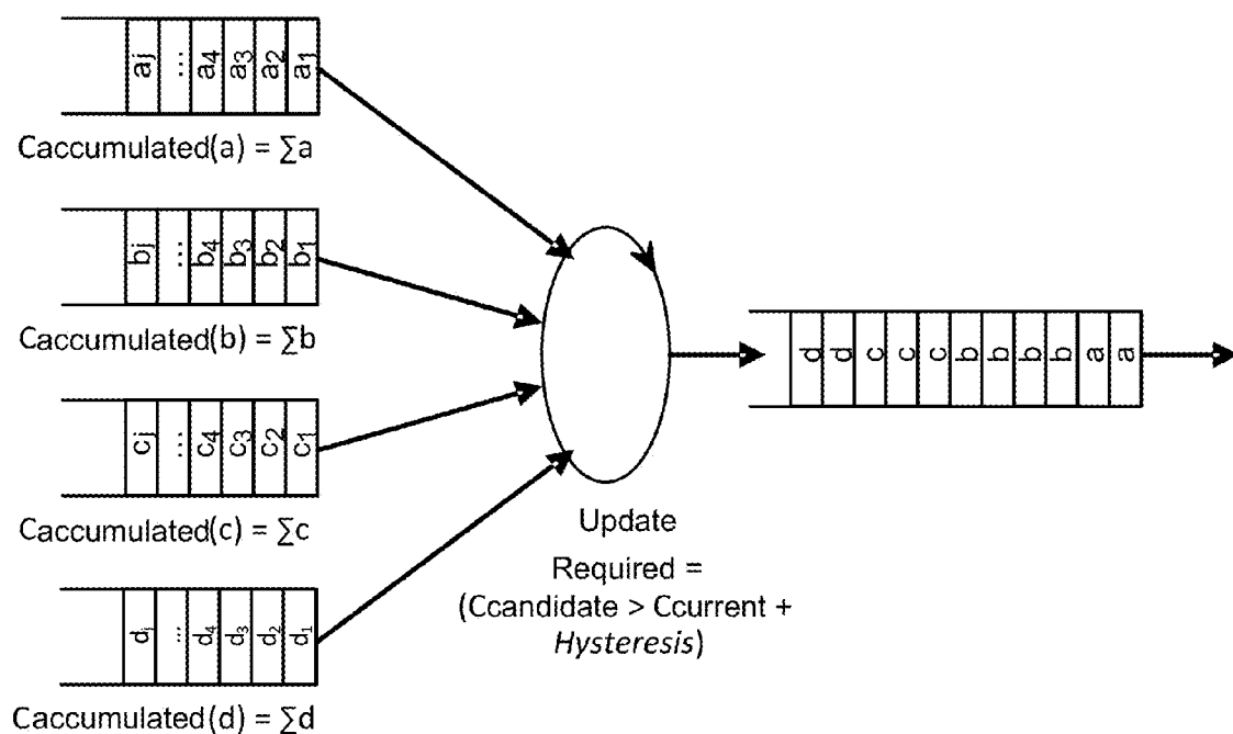
Figure 32: Scheduler grouping for minimal context thrashing
