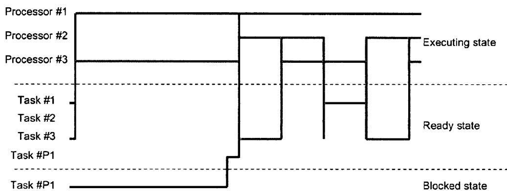
Figure 27: Three processor 3 timeslice tasks, 1 pre-emption task
