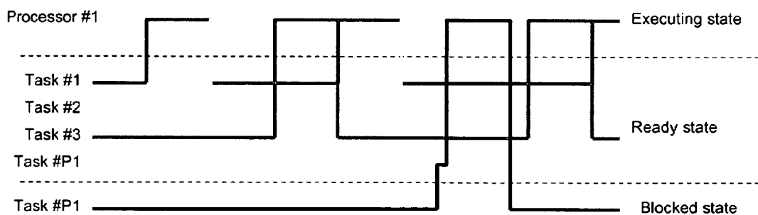
Figure 25: Single processor 3 timeslice, 1 pre-emption
