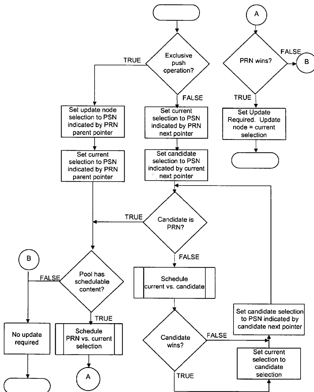
Figure 67: Intra-pool tier scheduler processing
