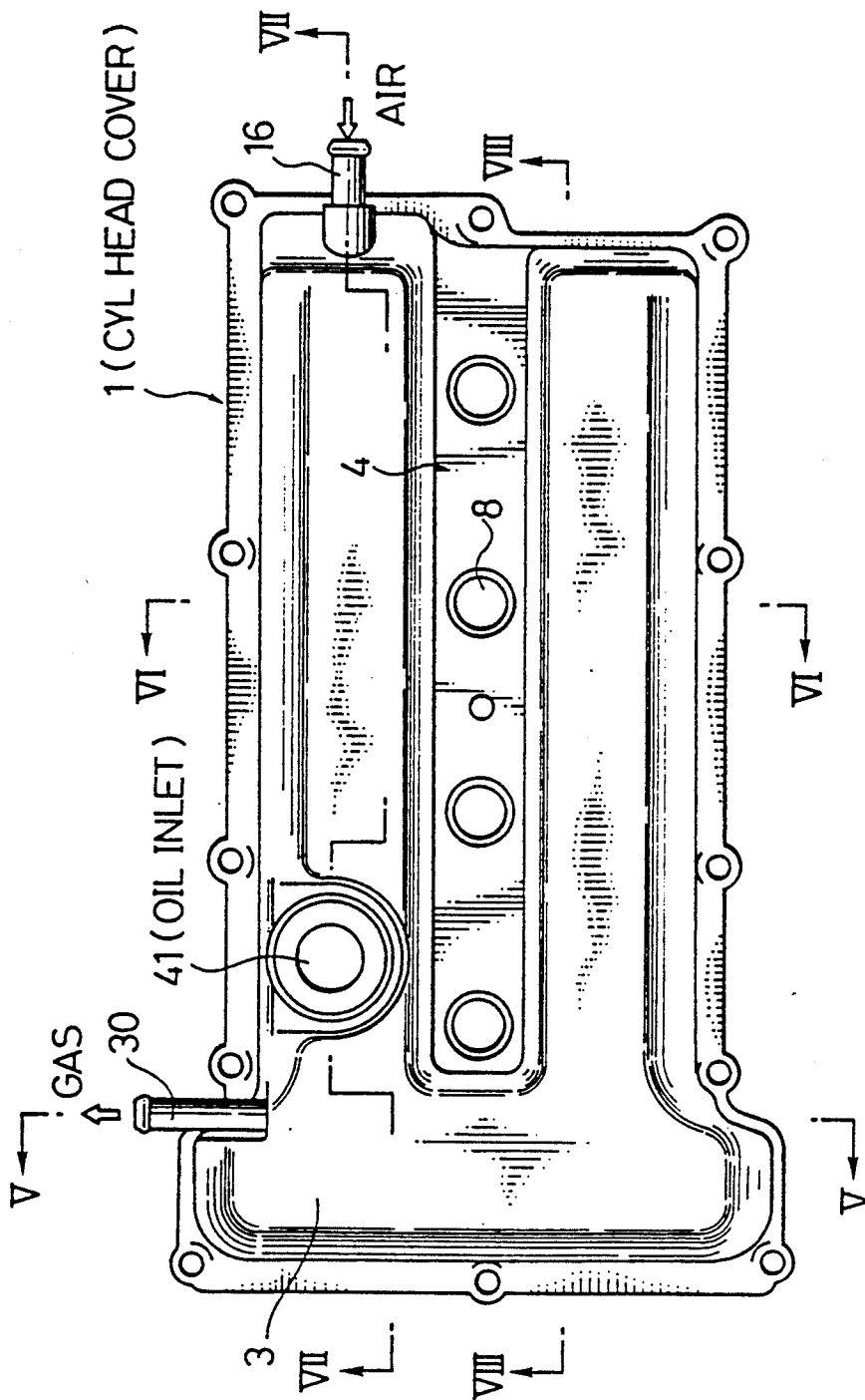
FIG. 2 (TOP VIEW)
