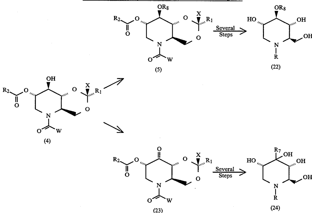
Scheme I: Generic Synthesis of 3-substituted 1,5-iminosugars
