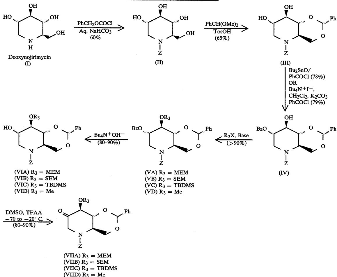
Scheme D: A Synthesis of 2-Ketone
