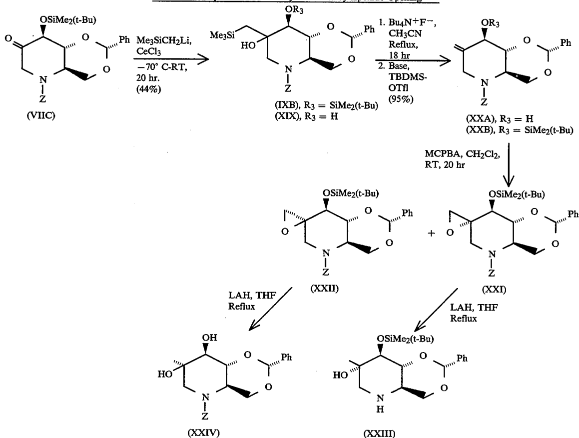
Scheme H: Synthesis of 2-Methyl Carbinol by Epoxide Opening
