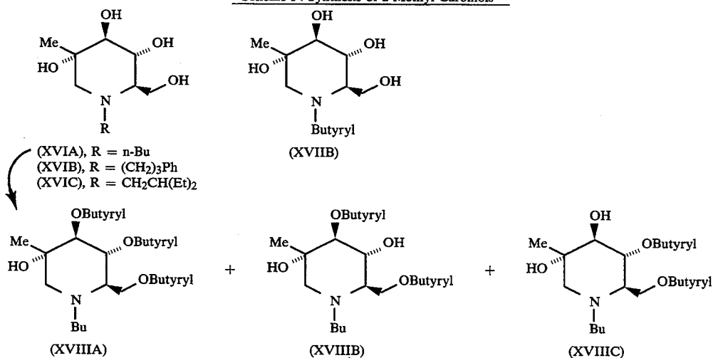
Scheme F: Synthesis of 2-Methyl Carbinols
