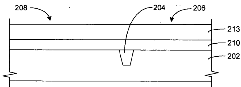
Fig. 2C (prior art)
