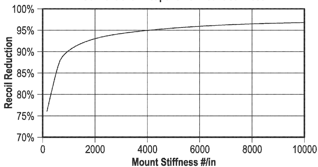
Recoil Load Reduction over Conventional Weapons Vs. Mount Stiffness
