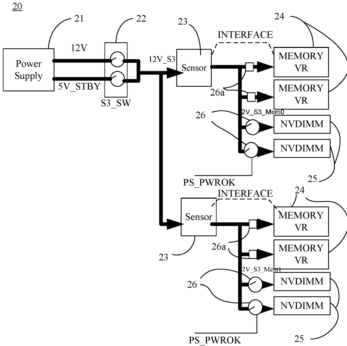
FIG. 1 RELATED ART
