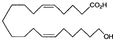
20-Hydroxyeicosa-5(Z),14(Z)-dienoic Acid (50)
