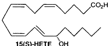
15(S)-HETE
