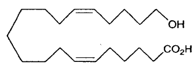
20-Hydroxyeicosa-6(Z),15(Z)-dienoic Acid (54)
