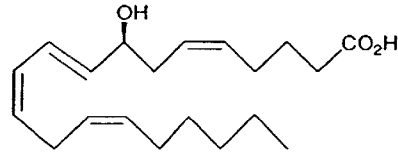
8(S)-HETE
