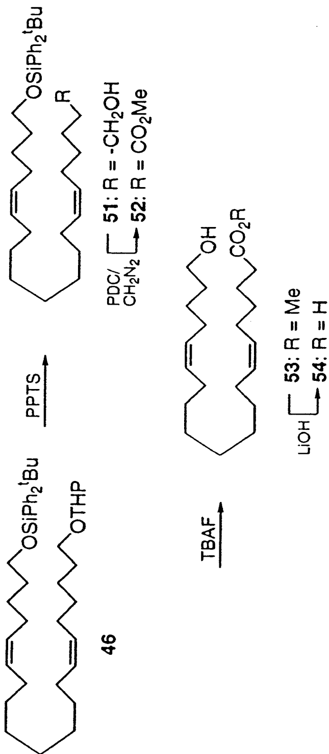
Scheme 6
