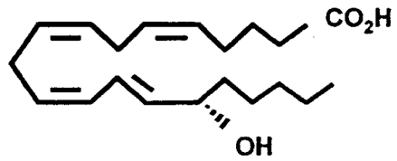
15(S)-HETE
