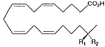
19(S)-HETE (34: R 1 = H, R 2 = OH)
