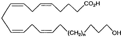
19-Hydroxynonadeca-5(Z),8(Z),11(Z),14(Z)-tetraenoic Acid (9a: n = 0)
