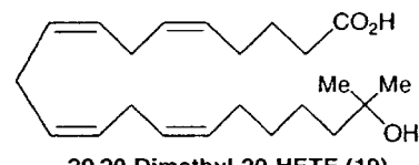
20,20-Dimethyl-20-HETE (19)
