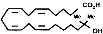
Dimethyl 20-HETE
