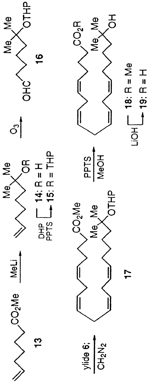
Scheme 2
