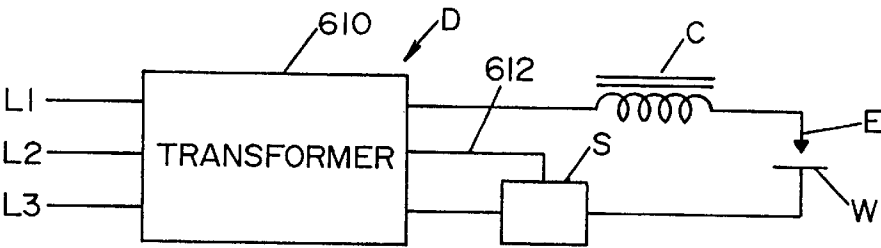
FIG. II (PRIOR ART)
