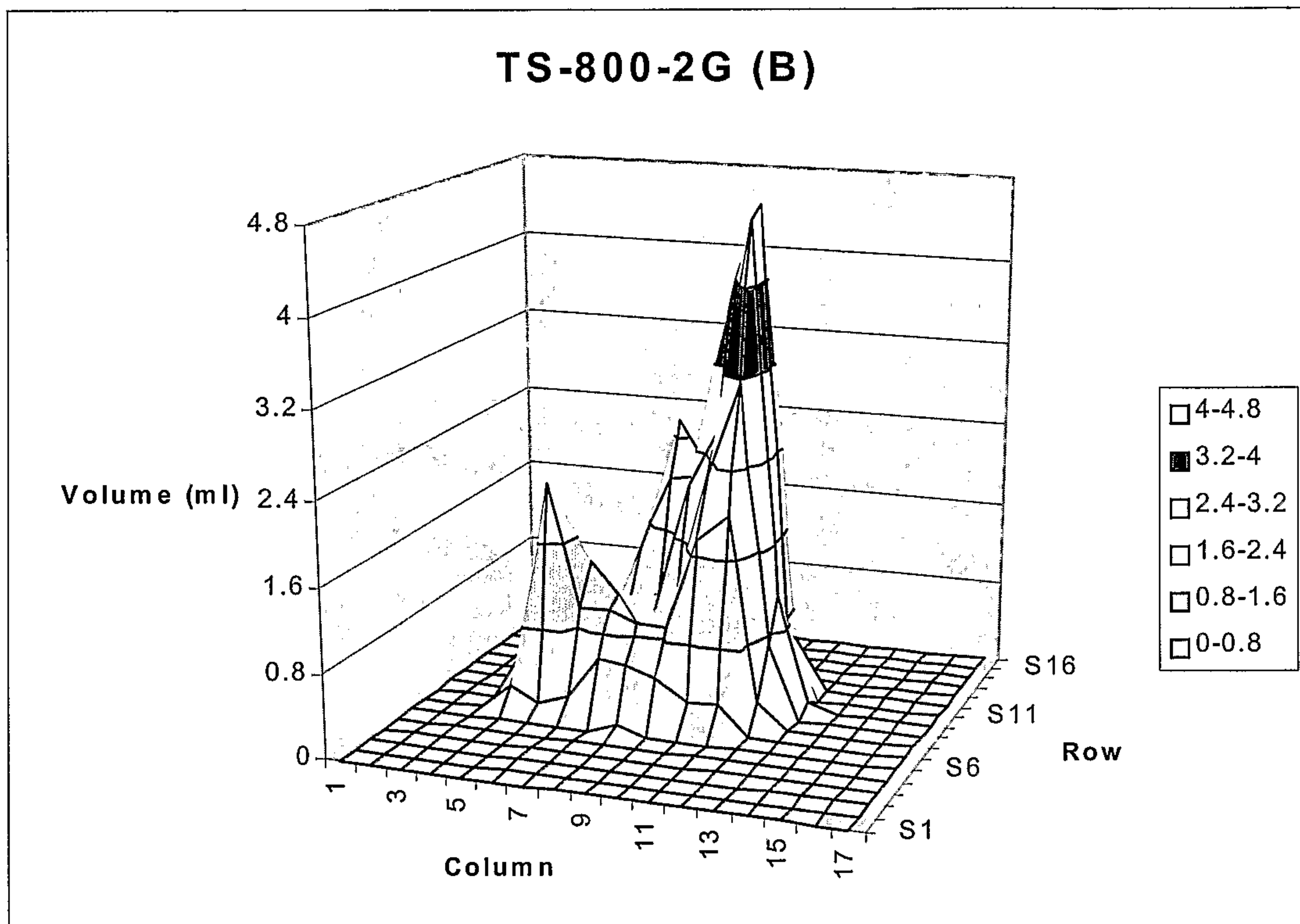
Plot 3. Graph of the spray pattern for the Calmar TS-800-2G sprayer.
