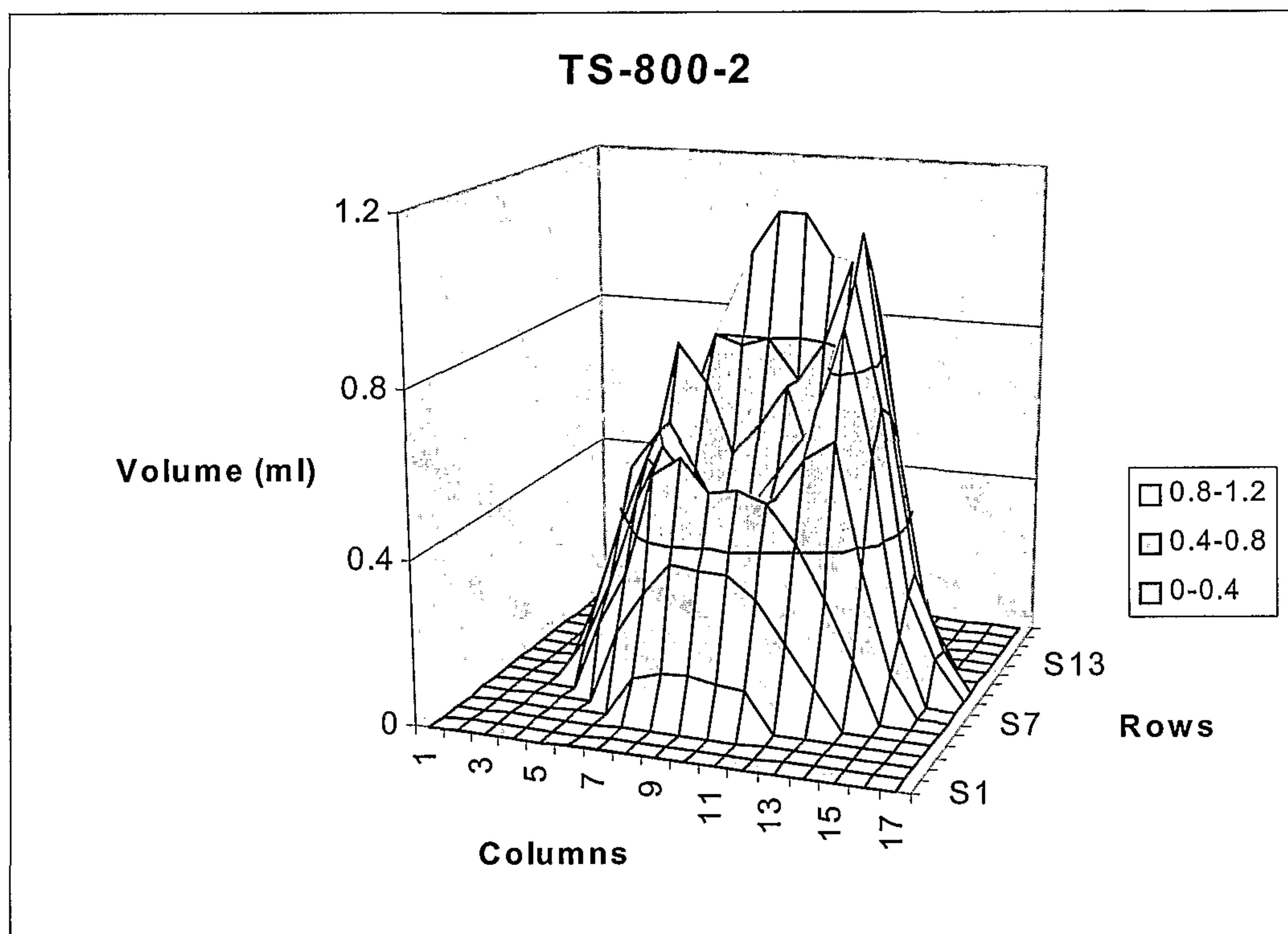
Plot 6. Graph of the spray pattern for the Calmar TS-800-2 sprayer.
