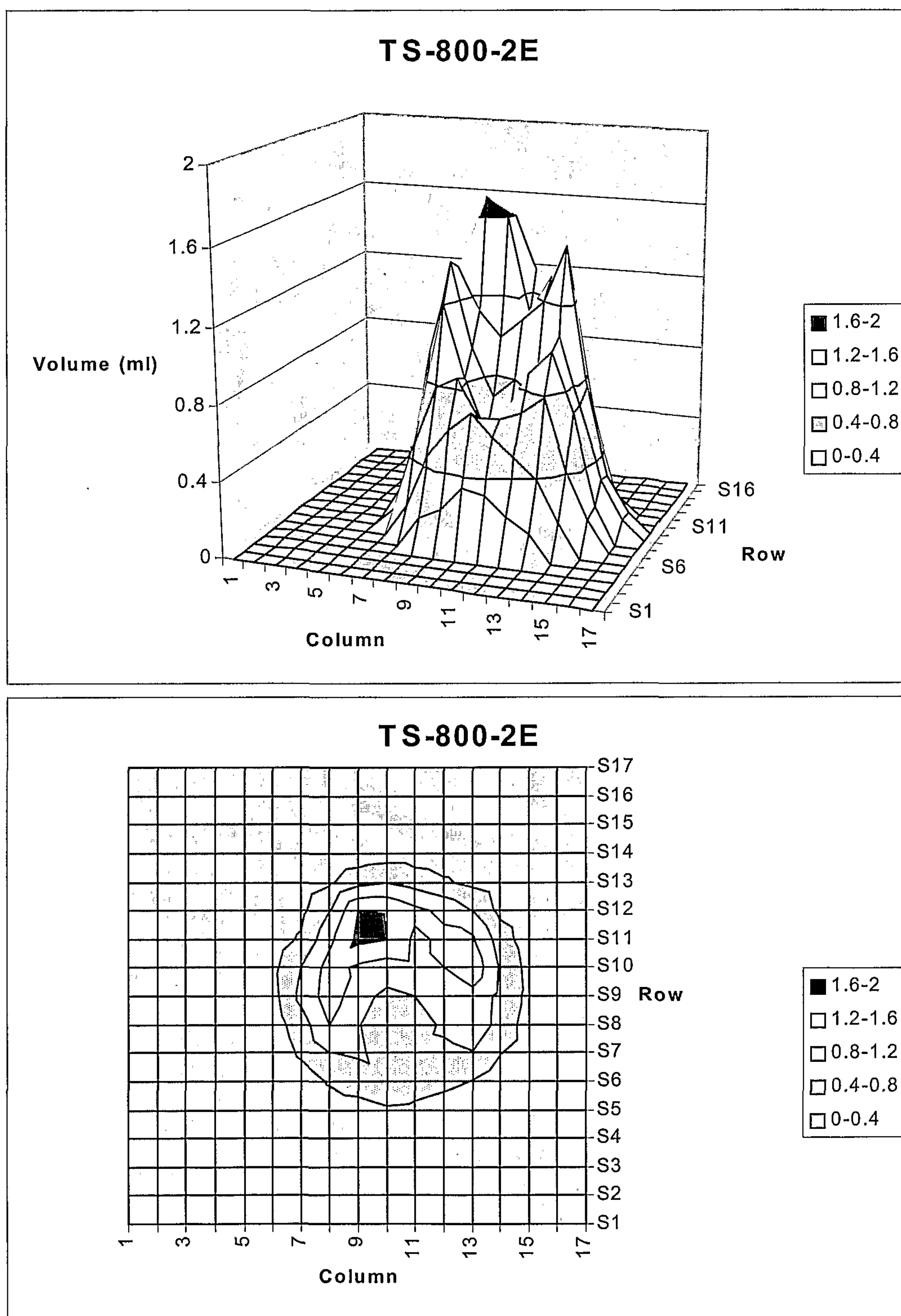
Plot 5. Graph of the spray pattern for the Calmar TS-800-2E sprayer
