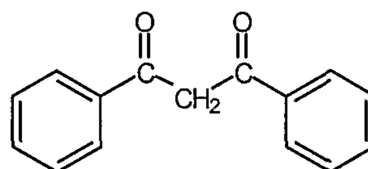
Dibenzoylmethane
