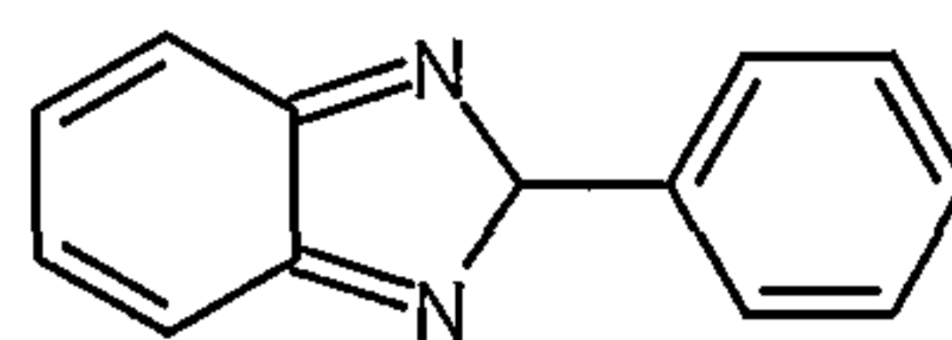
Phenylbenzimidazole
