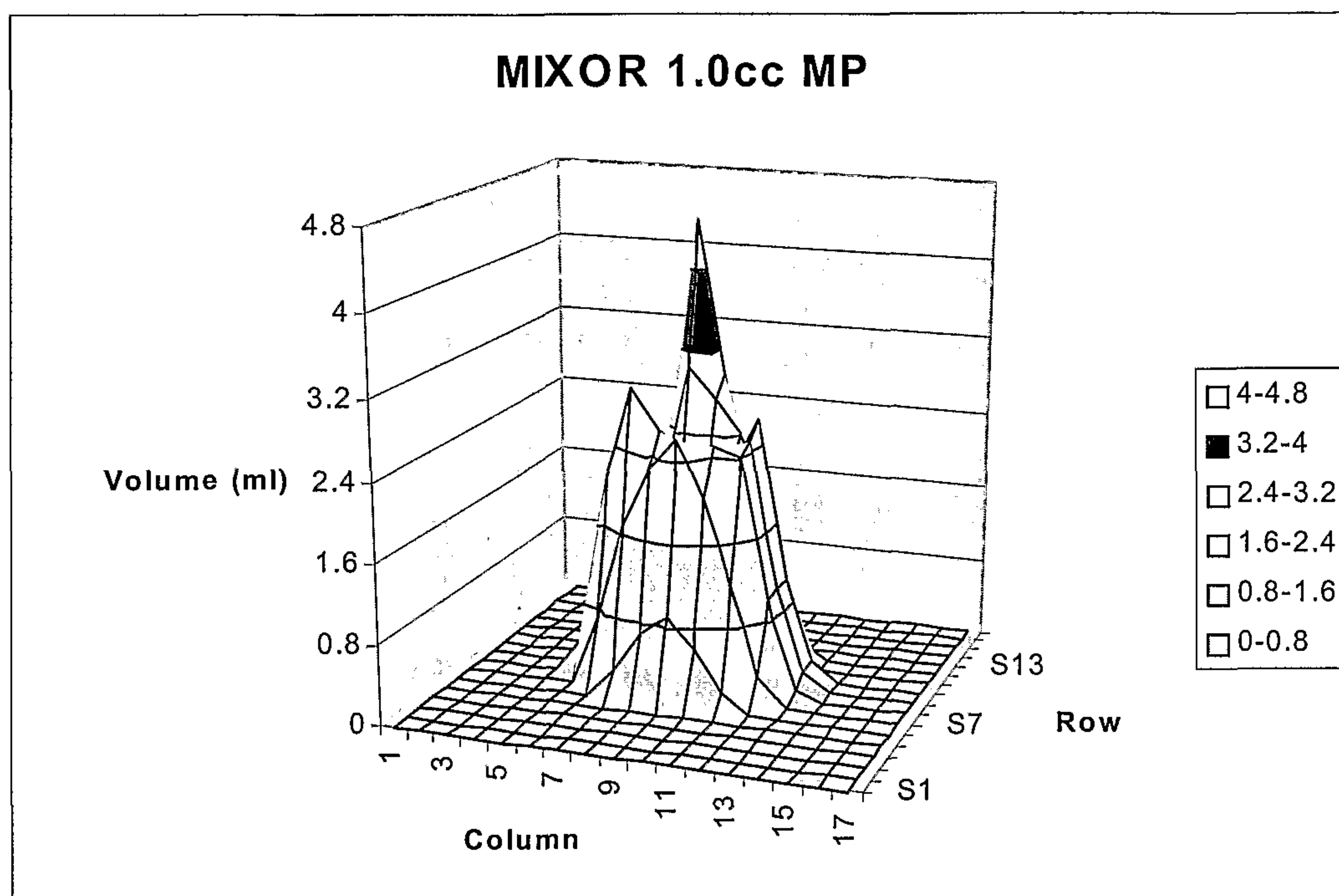
Plot 2. Graph of the spray pattern for the Mixor 1.0cc MP sprayer.
