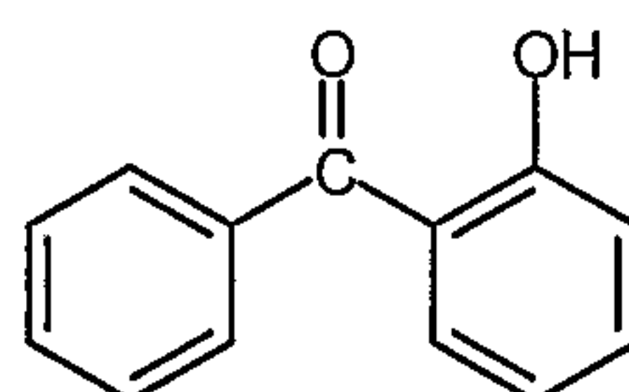
2-Hydroxybenzophenone
