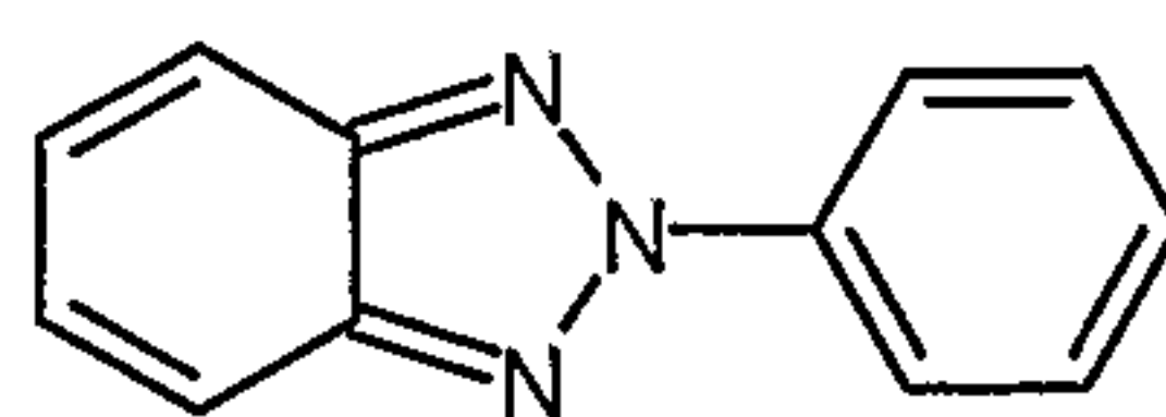
Phenylbenzotriazole
