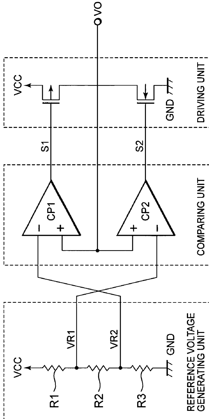
CONVENTIONAL REFERENCE VOLTAGE GENERATING CIRCUIT
