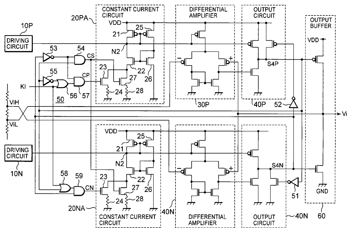
DRIVER POWER SUPPLY CIRCUIT ACCORDING TO SECOND EMBODIMENT
