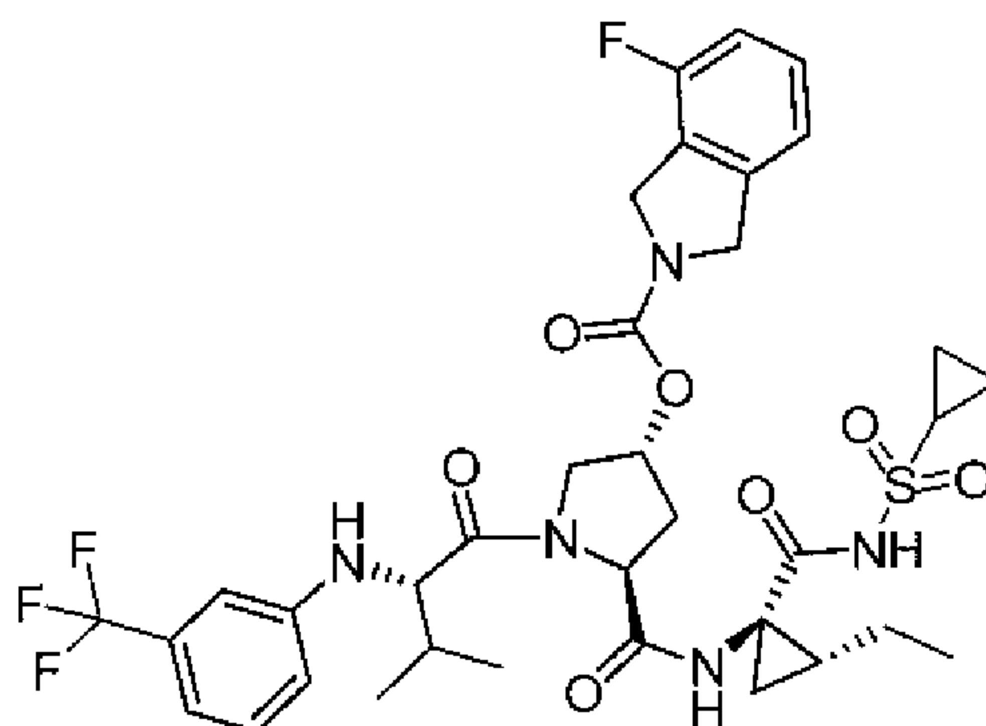
Compound 47
