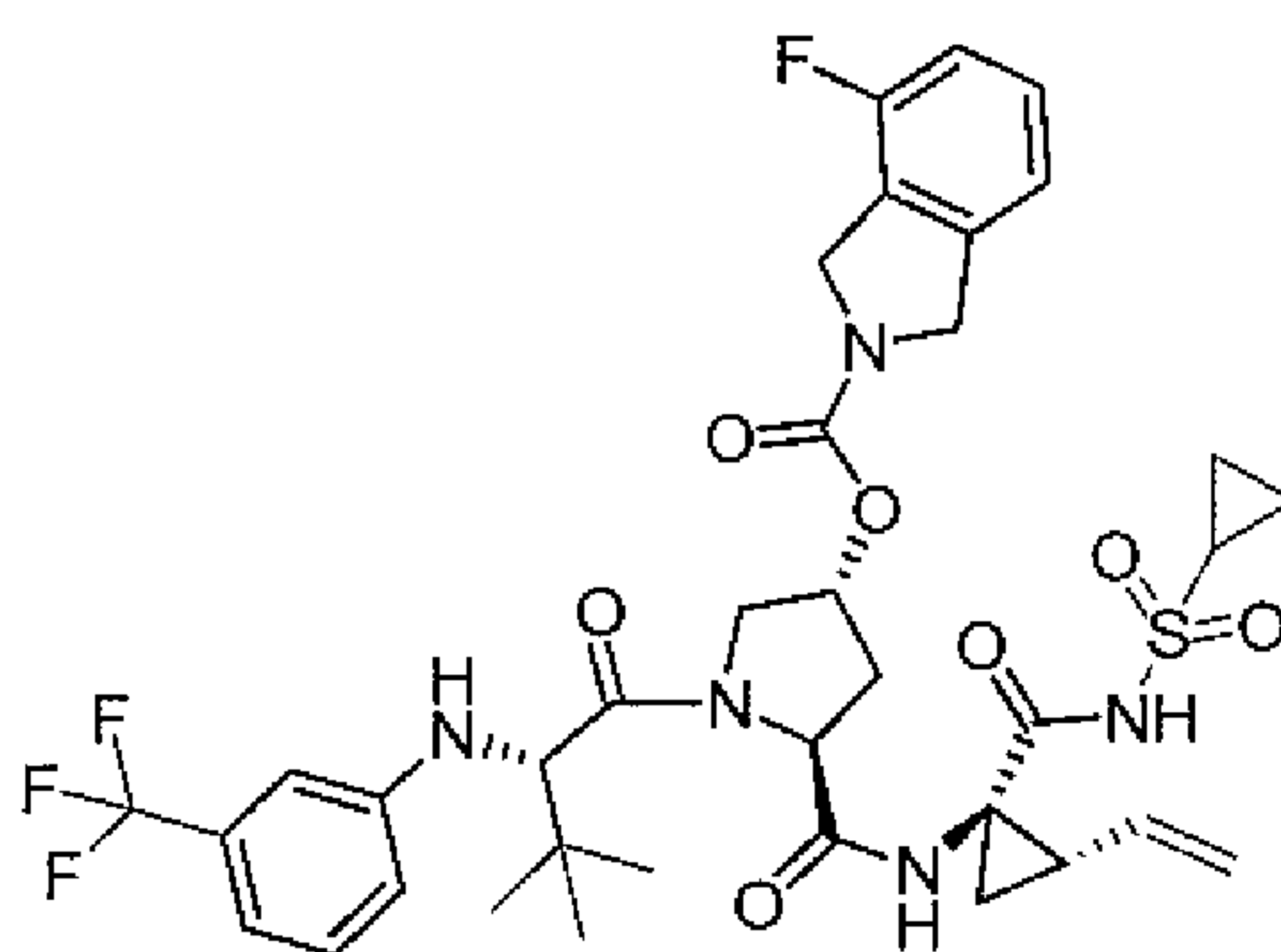
Compound 43
