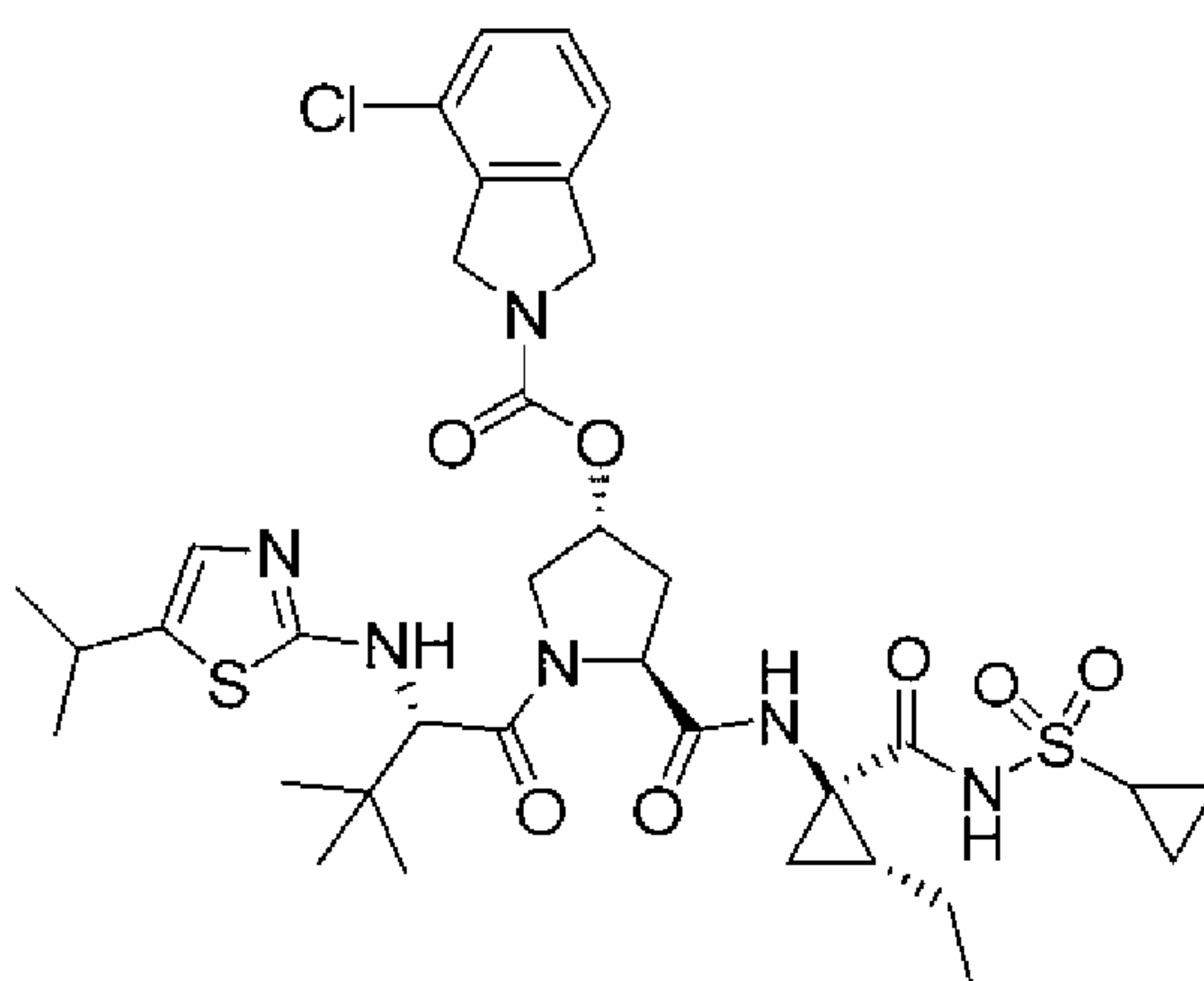
Compound 65
