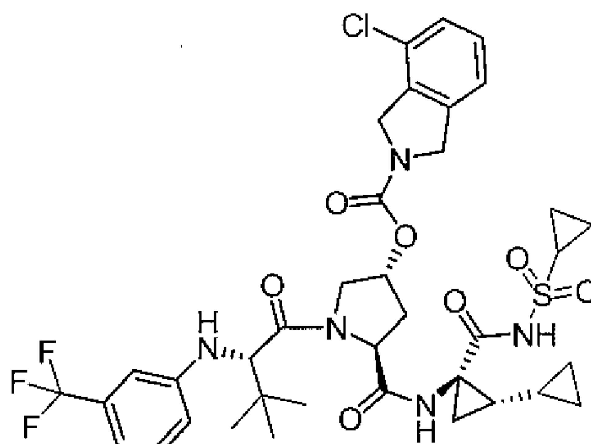
Compound 60
