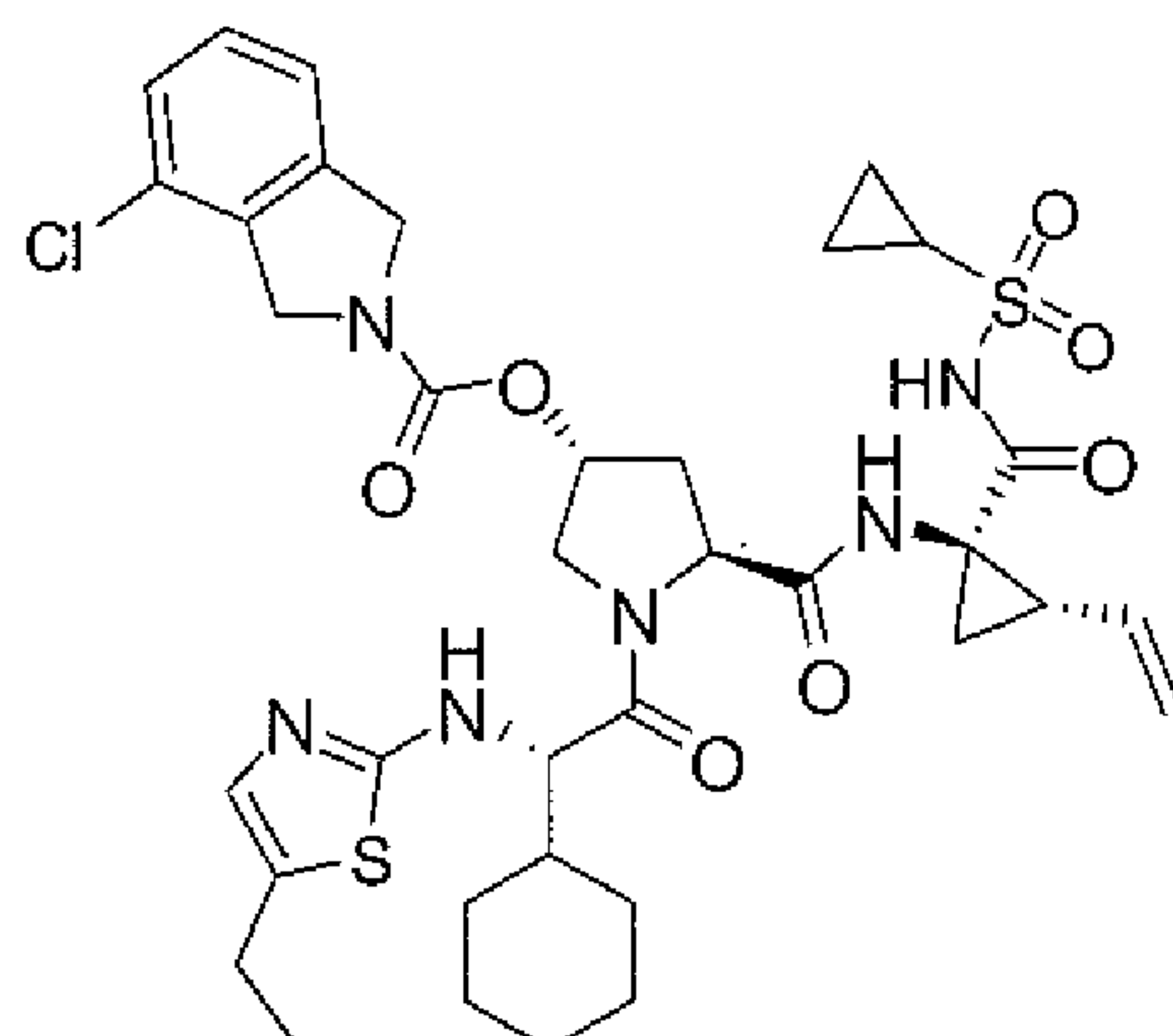
Compound 62
