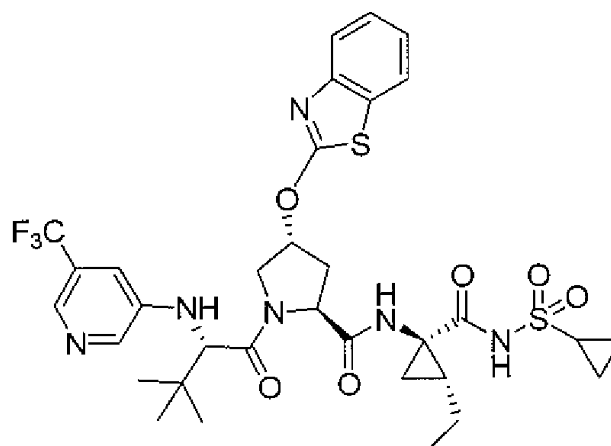
Compound 70
