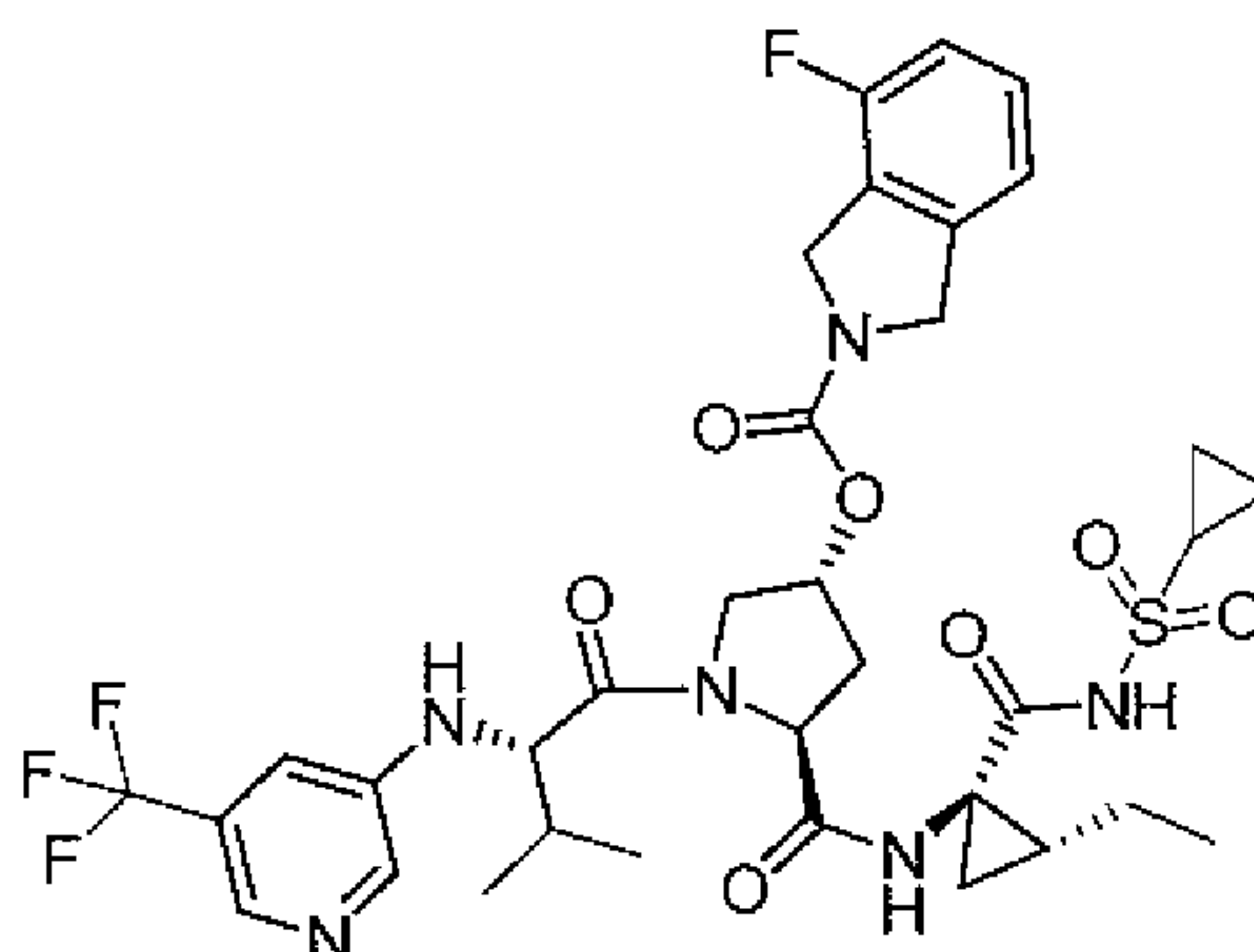
Compound 48
