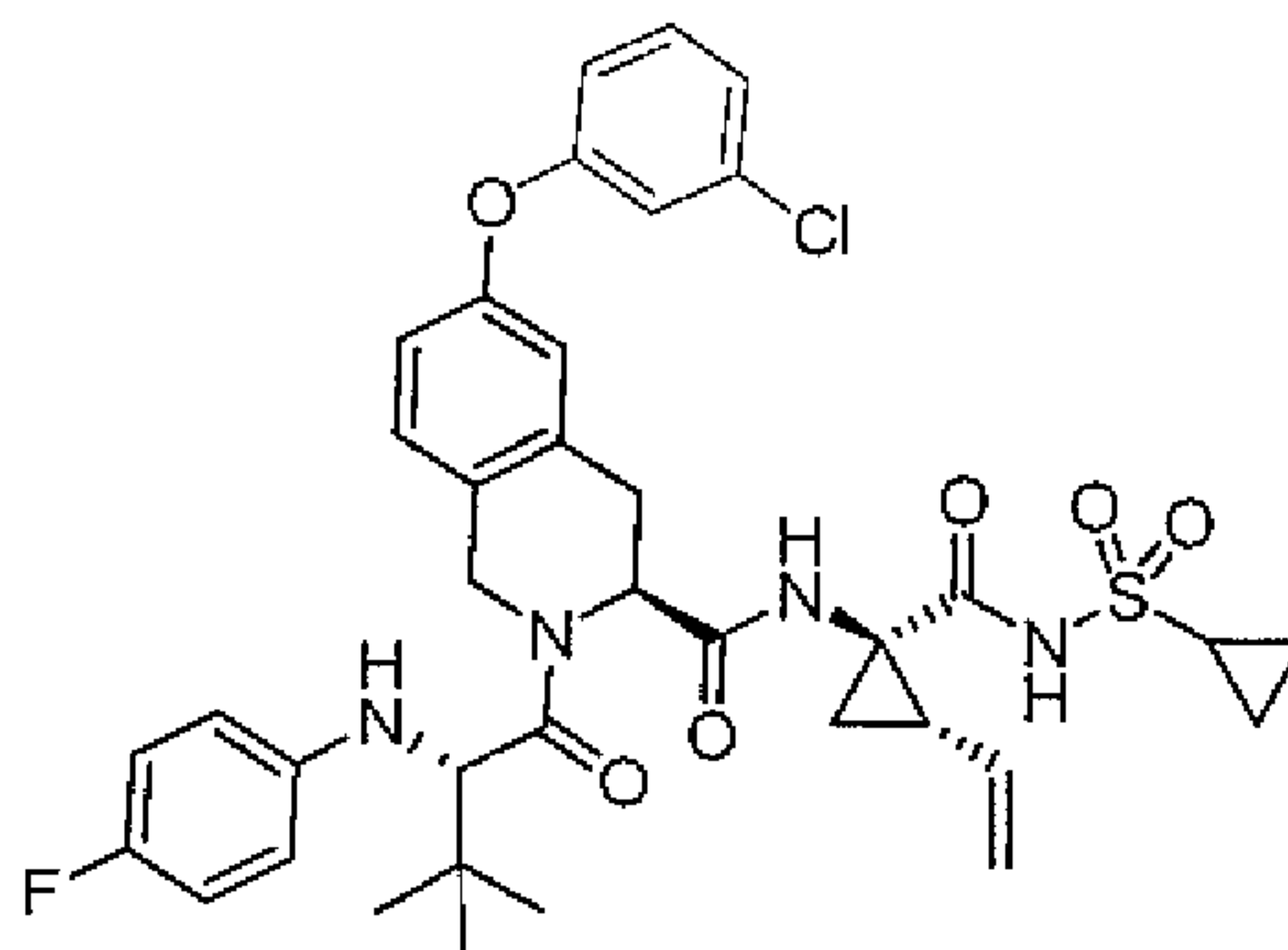
Compound 11
