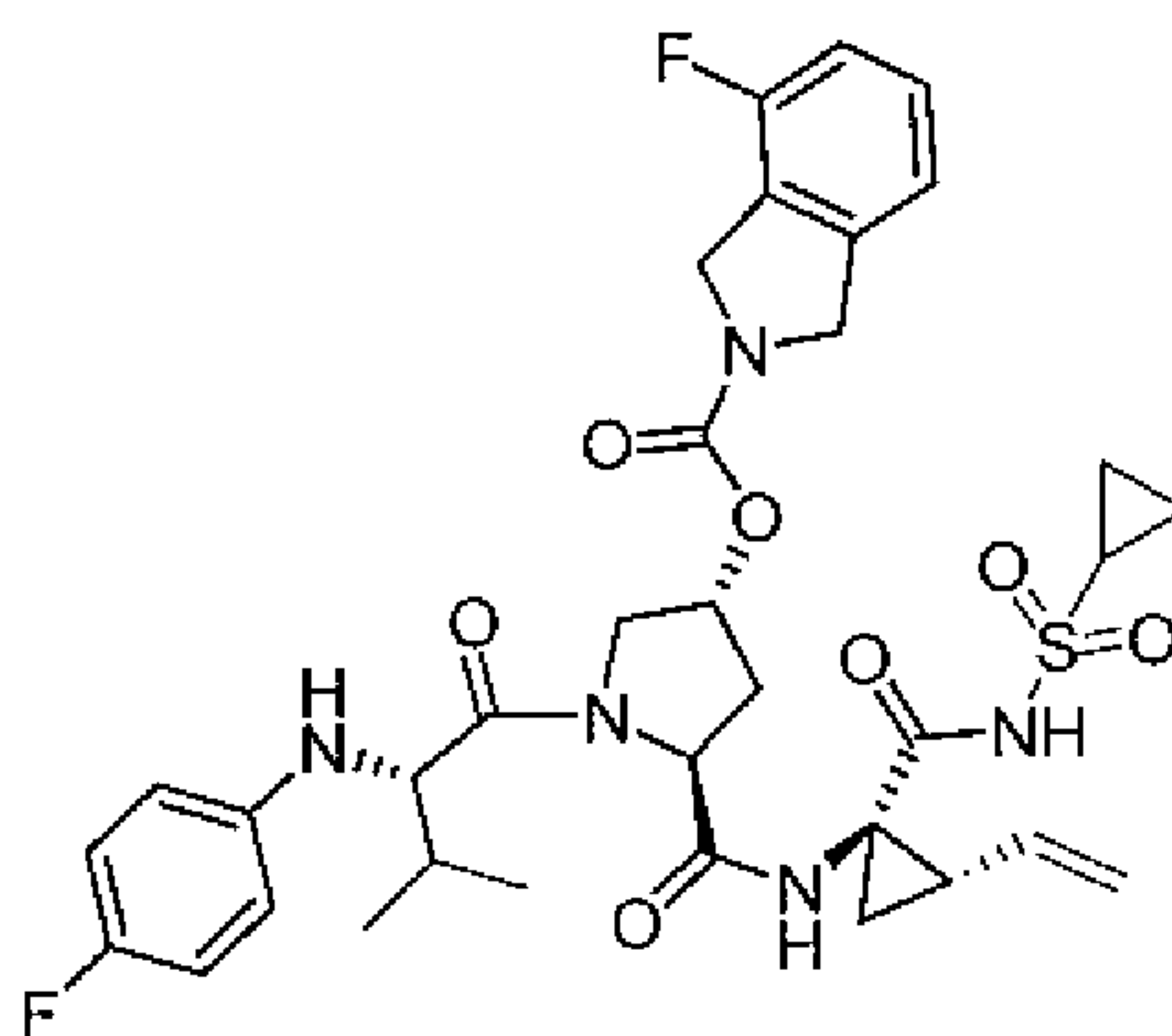
Compound 33
