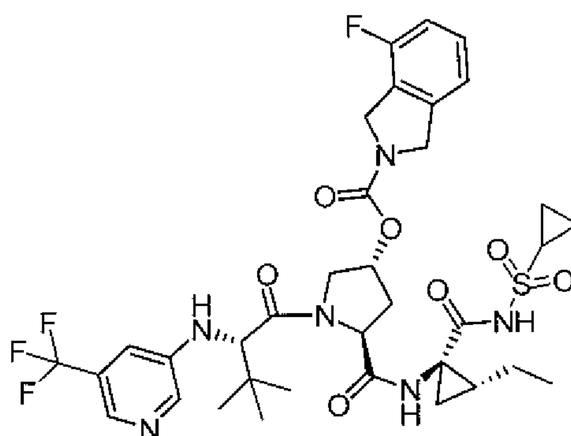
Compound 57
