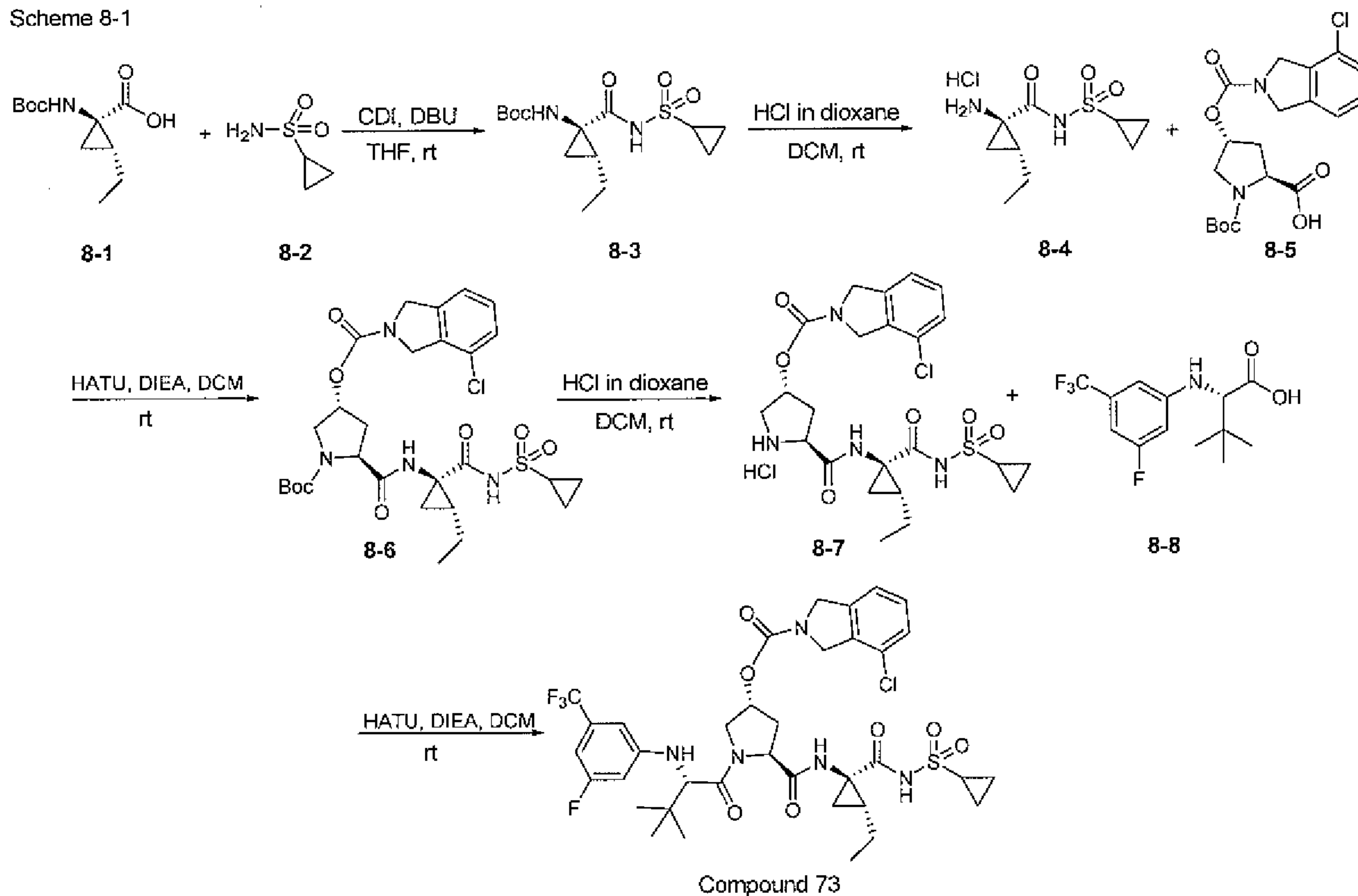
Scheme 8-1
