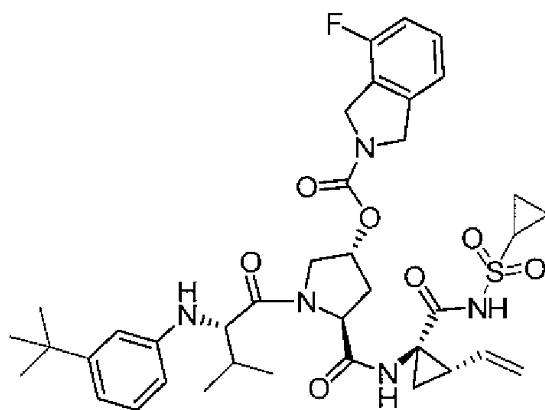
Compound 40
