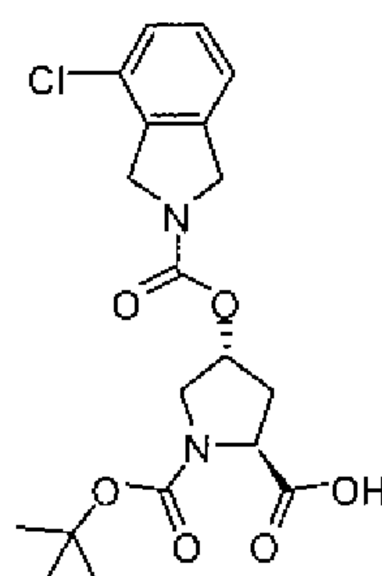
Compound 26
