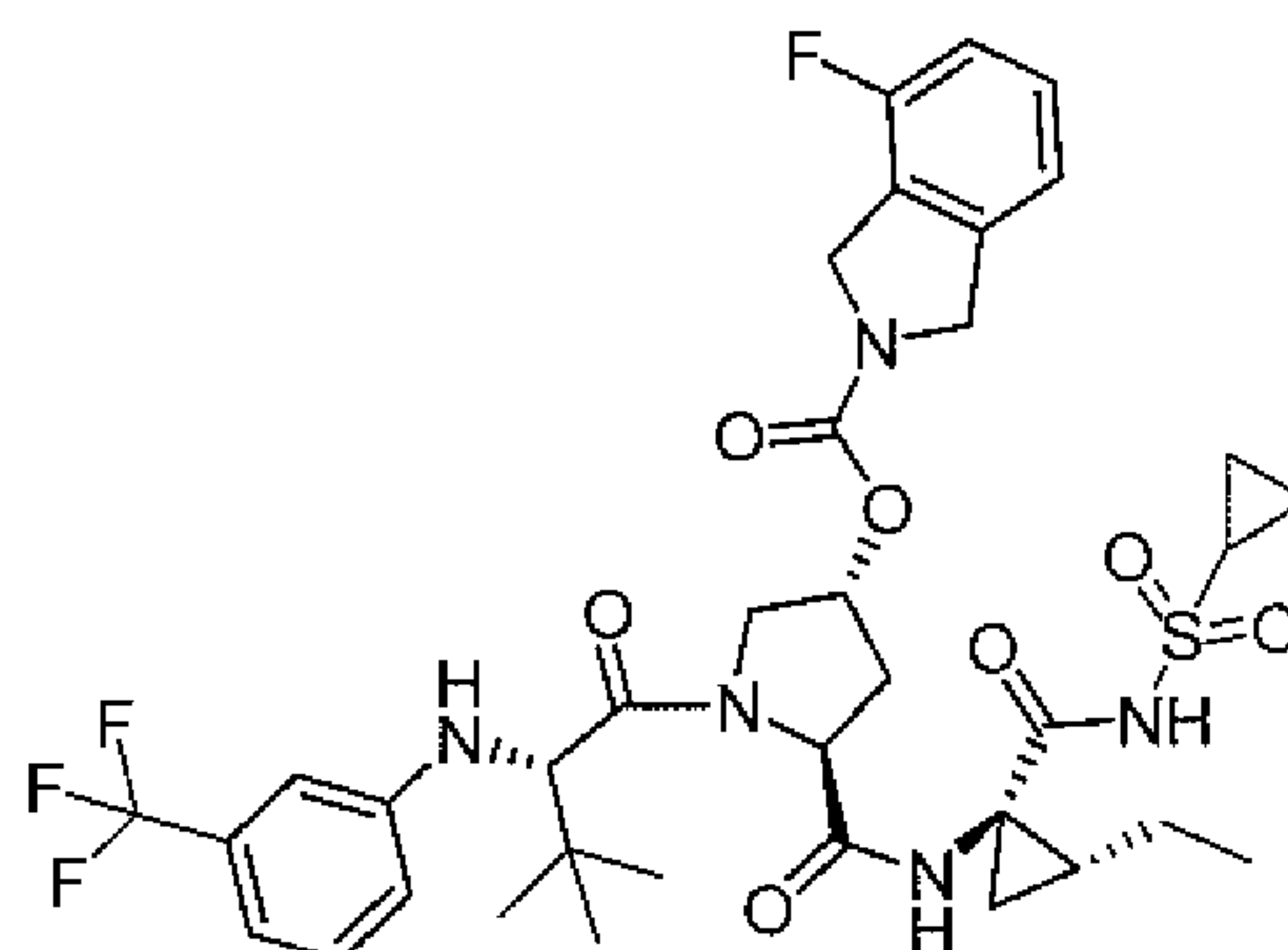
Compound 56
