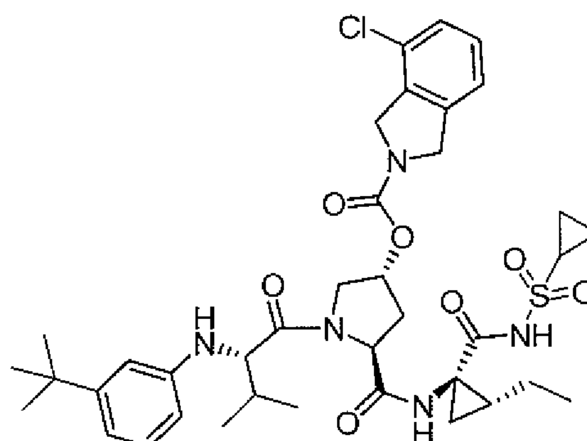
Compound 46
