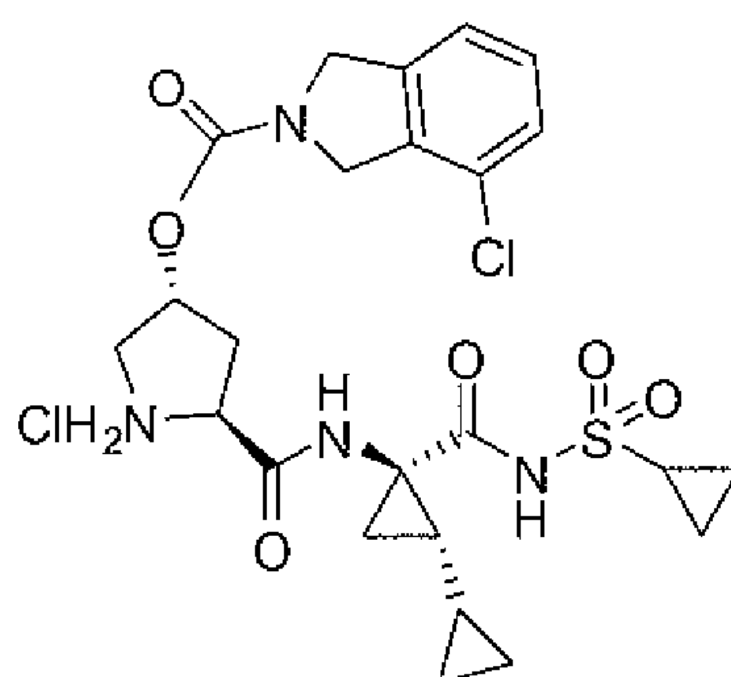
Compound 27
