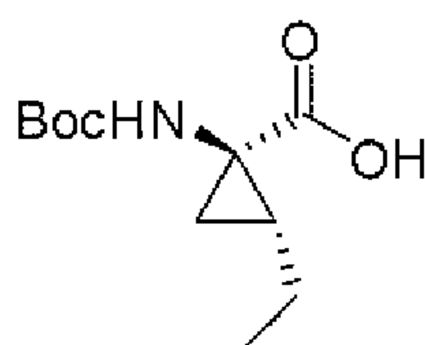
Compound 23
