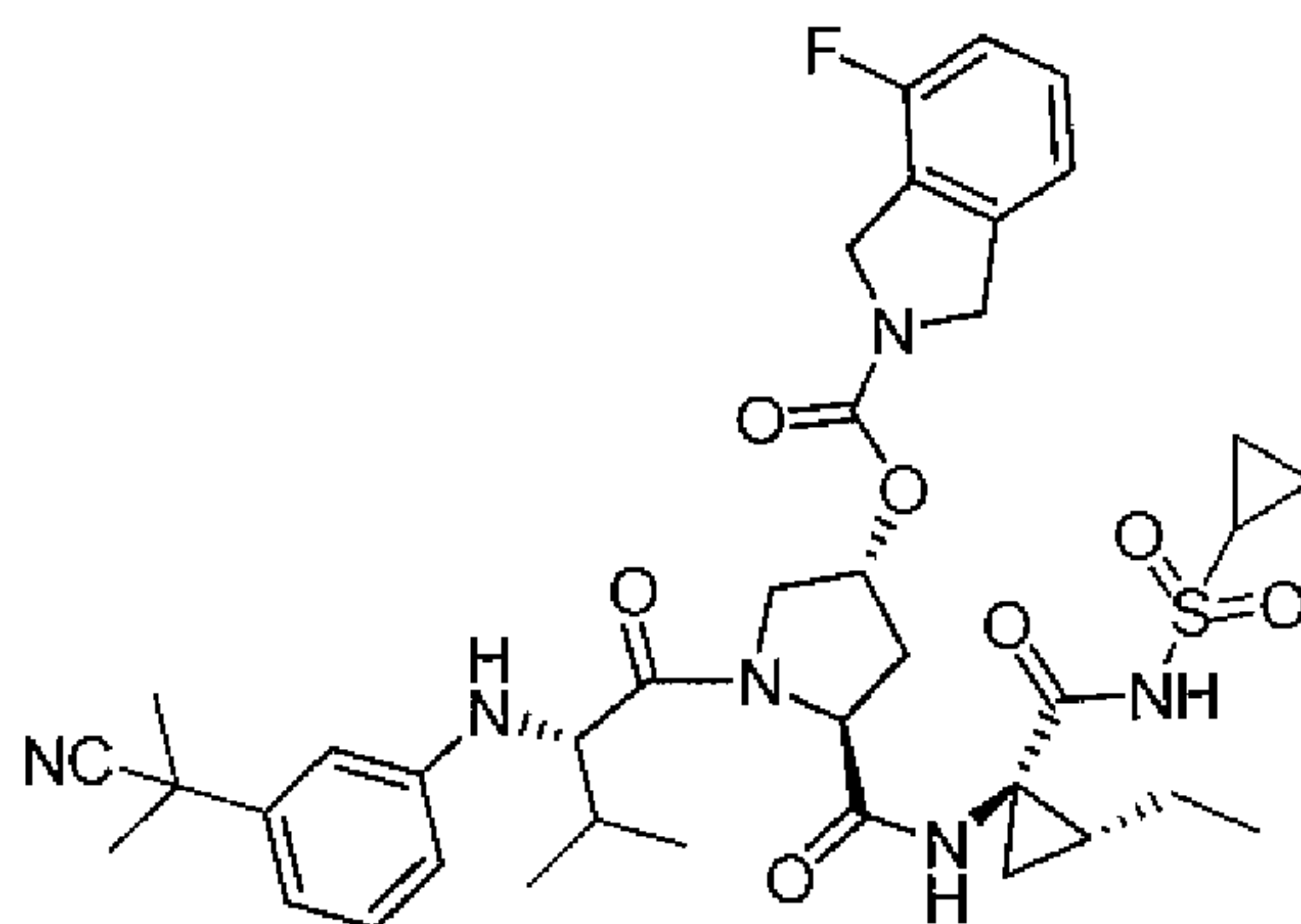
Compound 53
