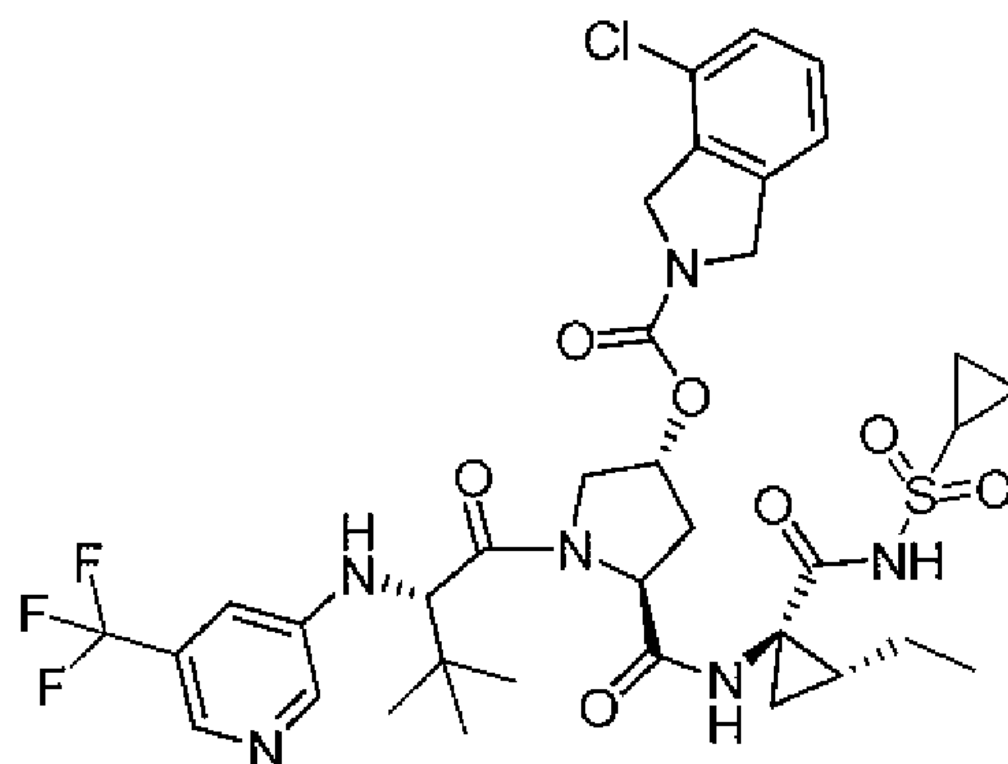
Compound 58
