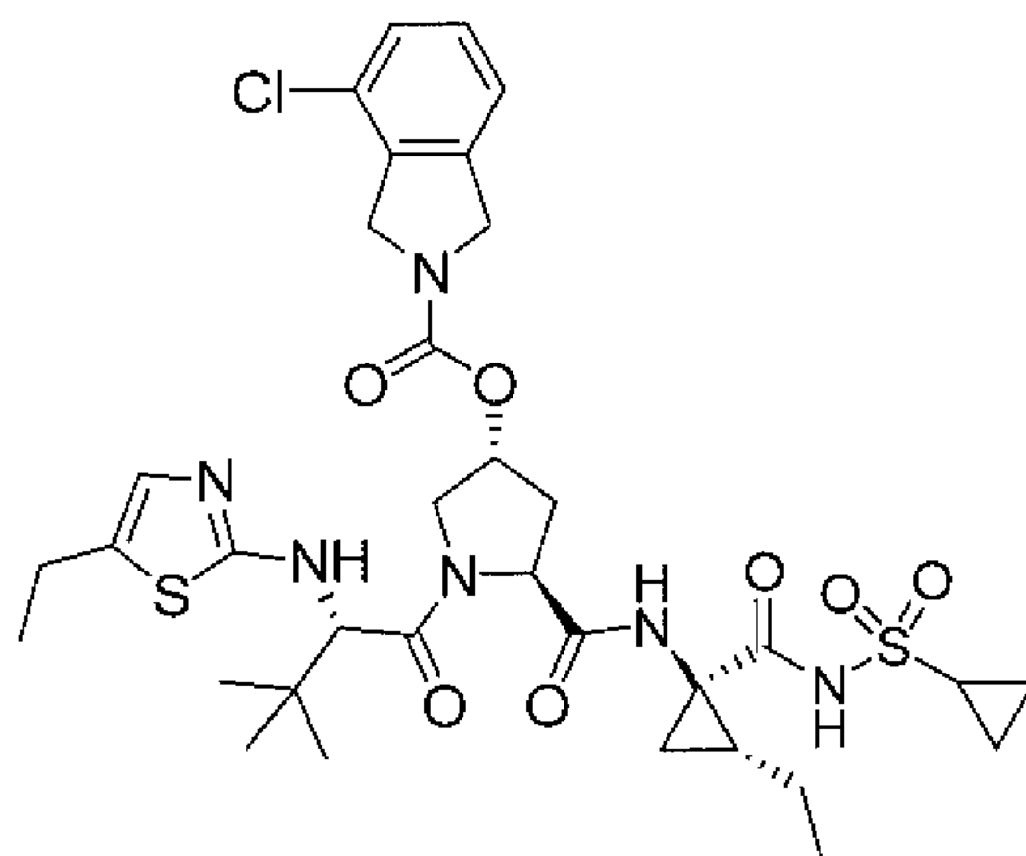
Compound 66
