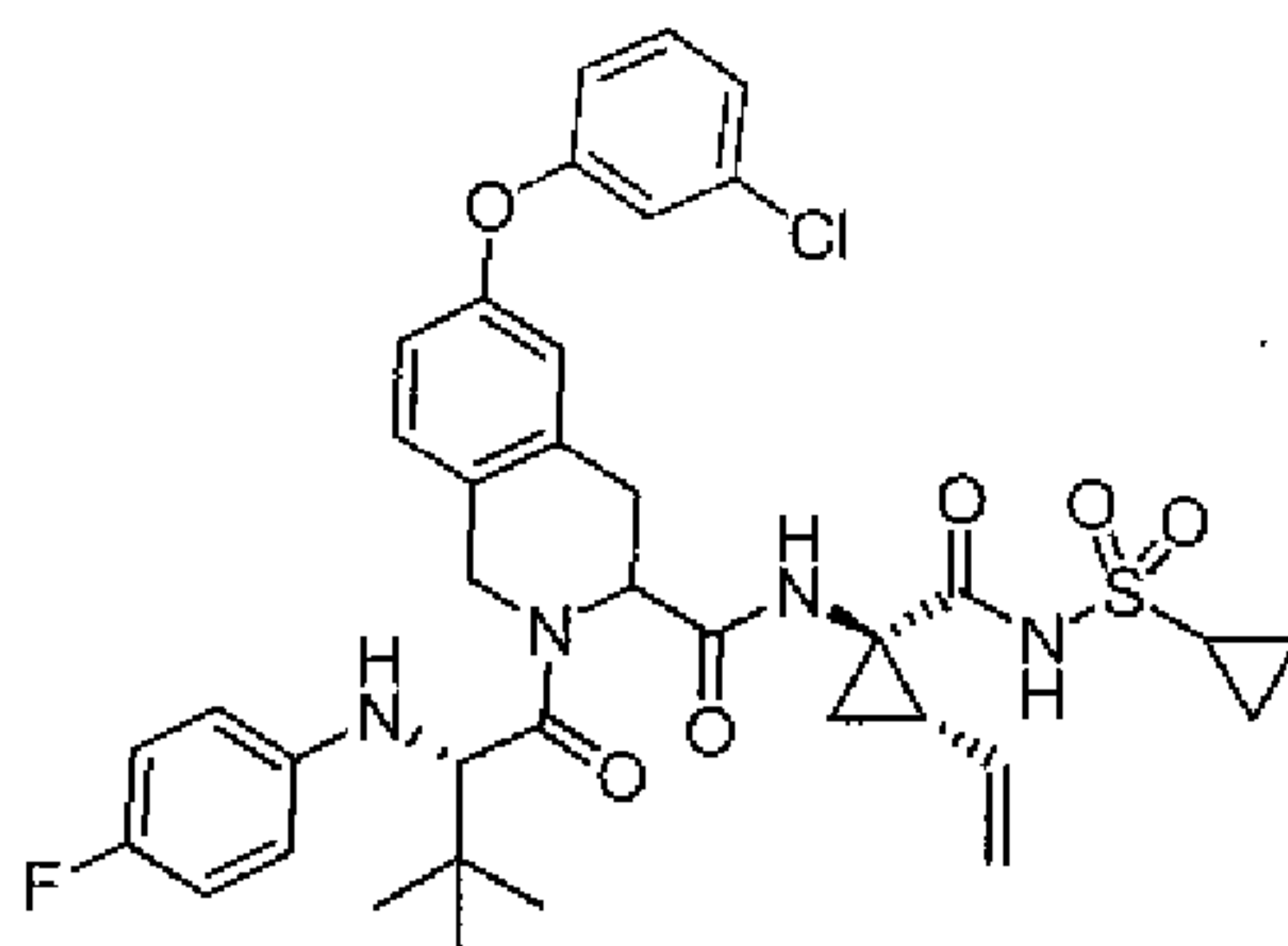
Compound 10
