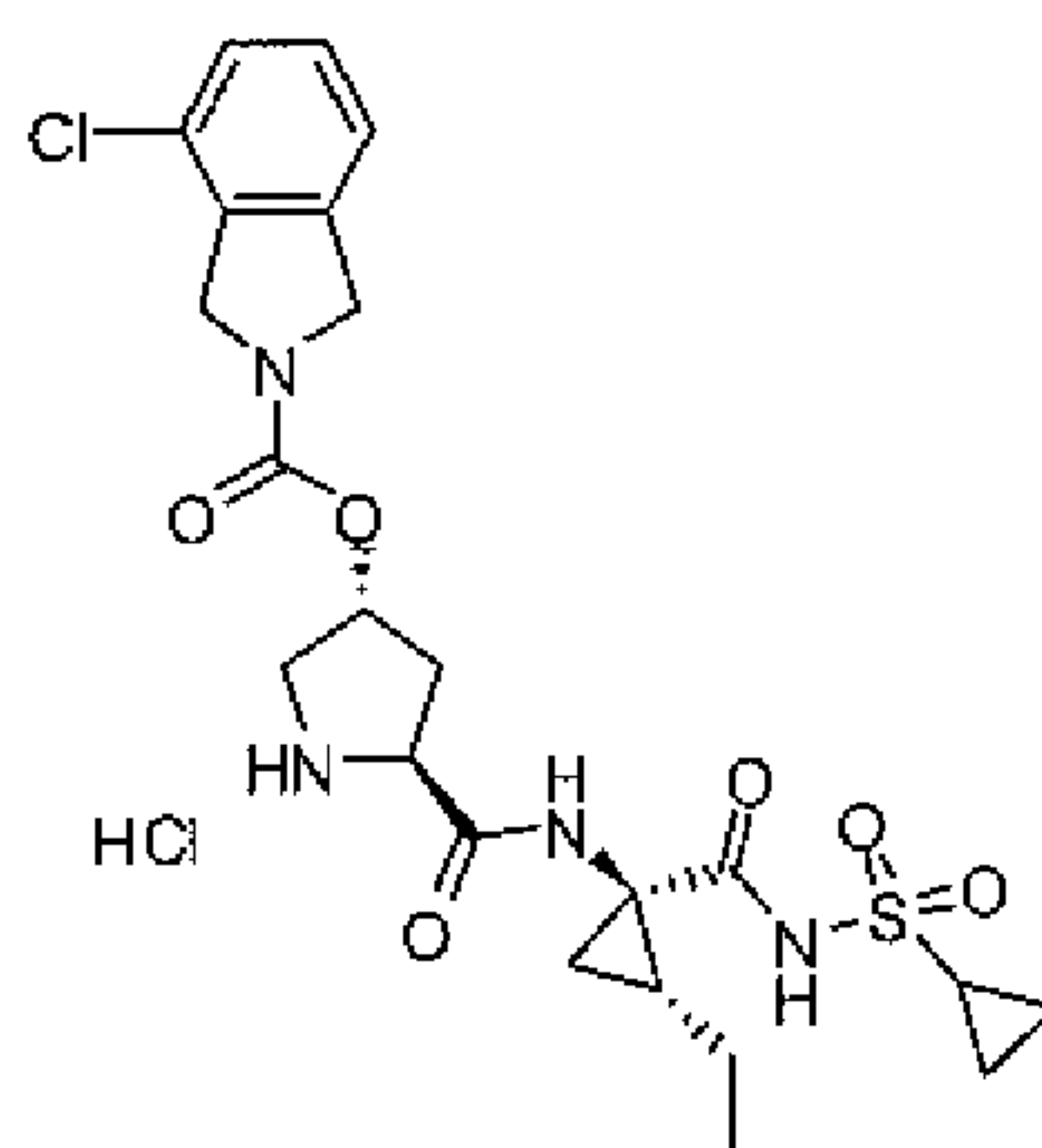
Compound 28
