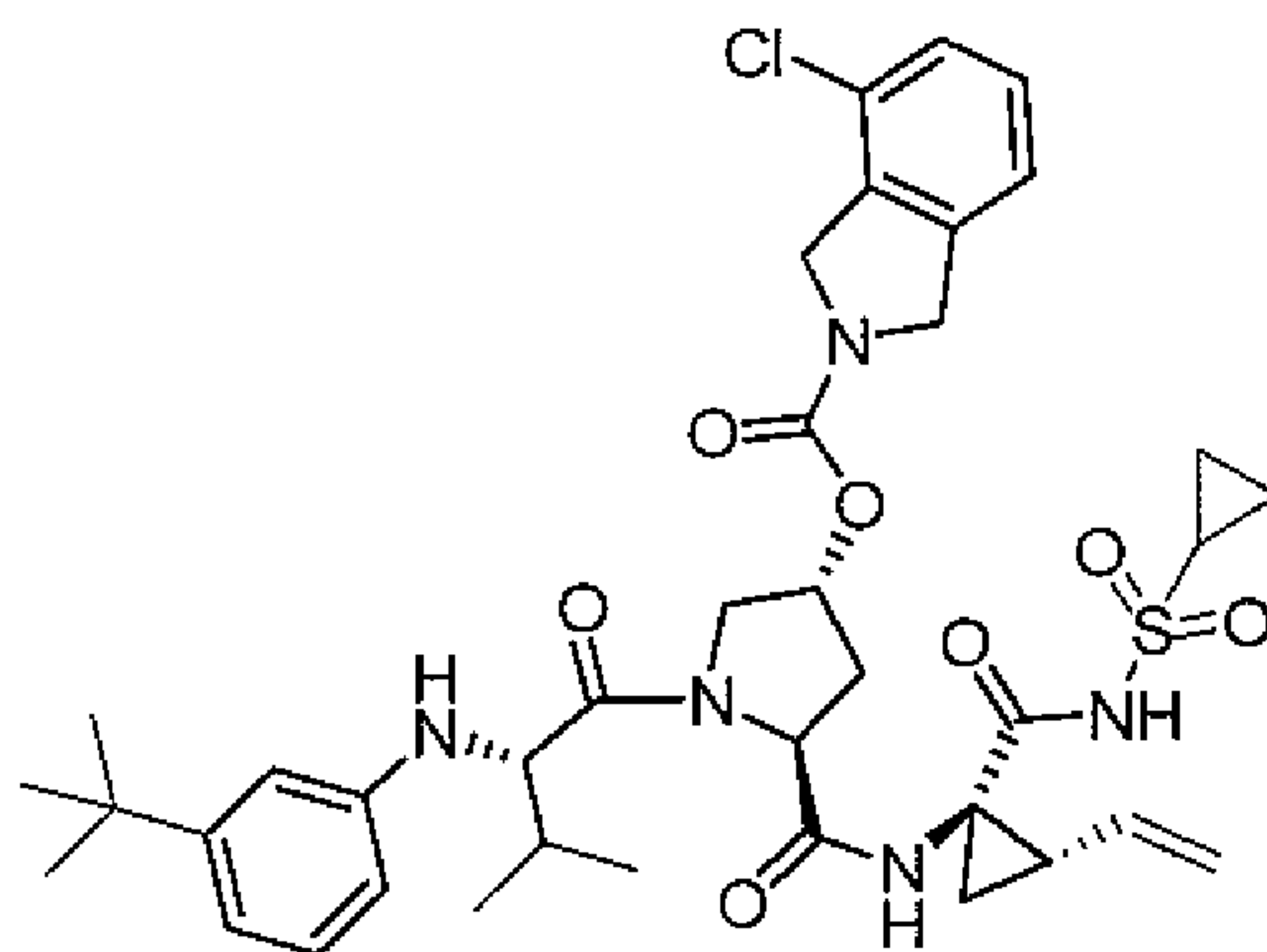
Compound 41
