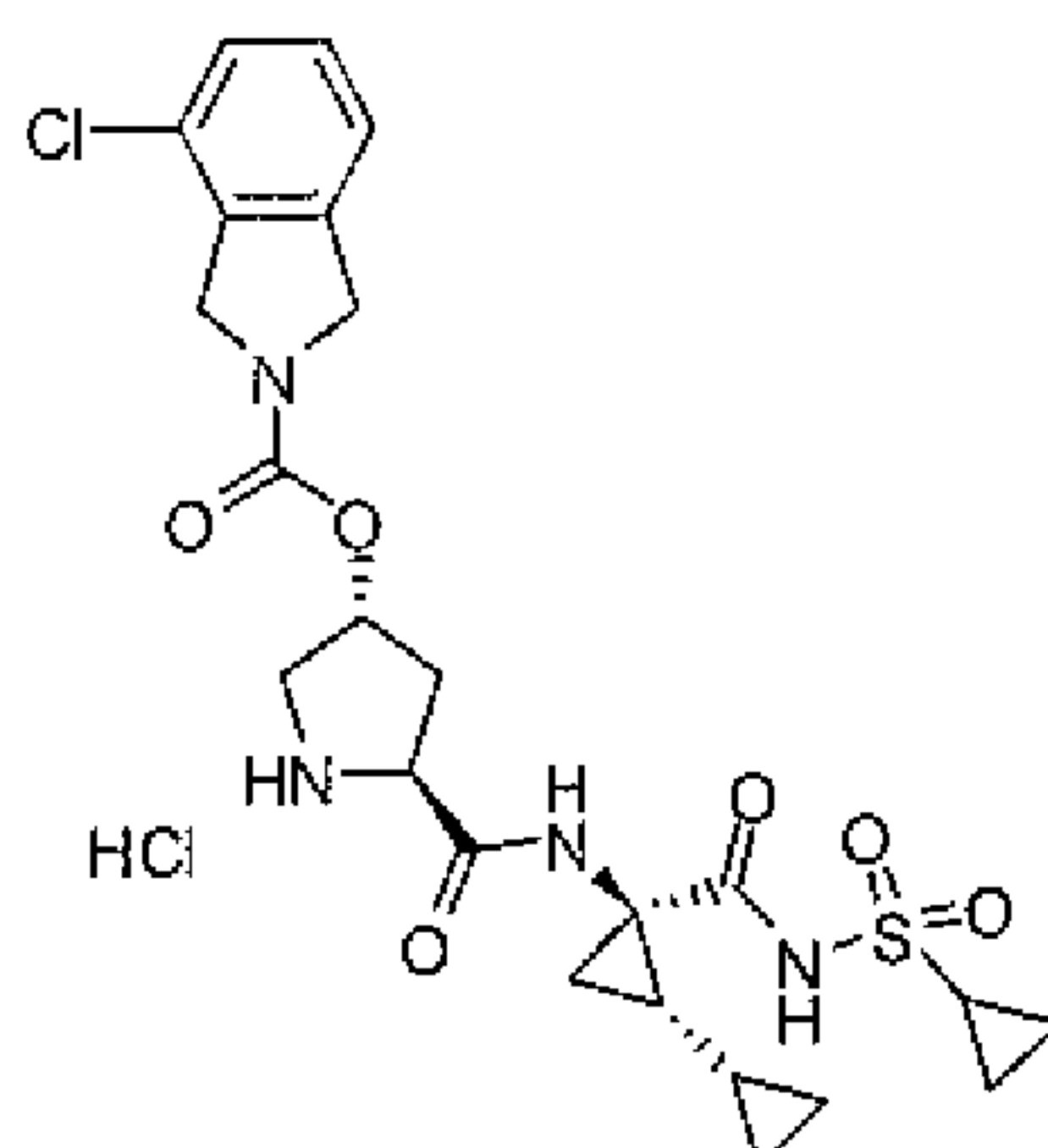
Compound 24
