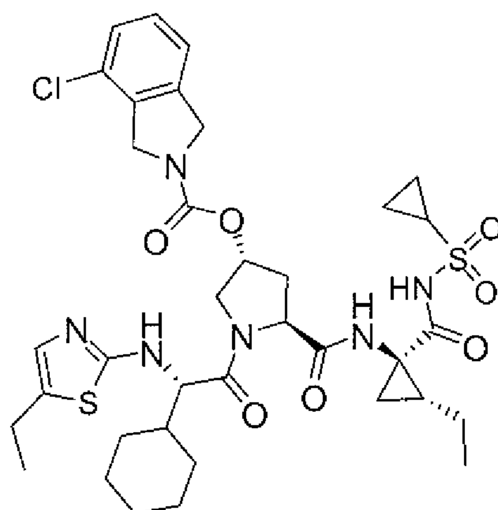
Compound 64
