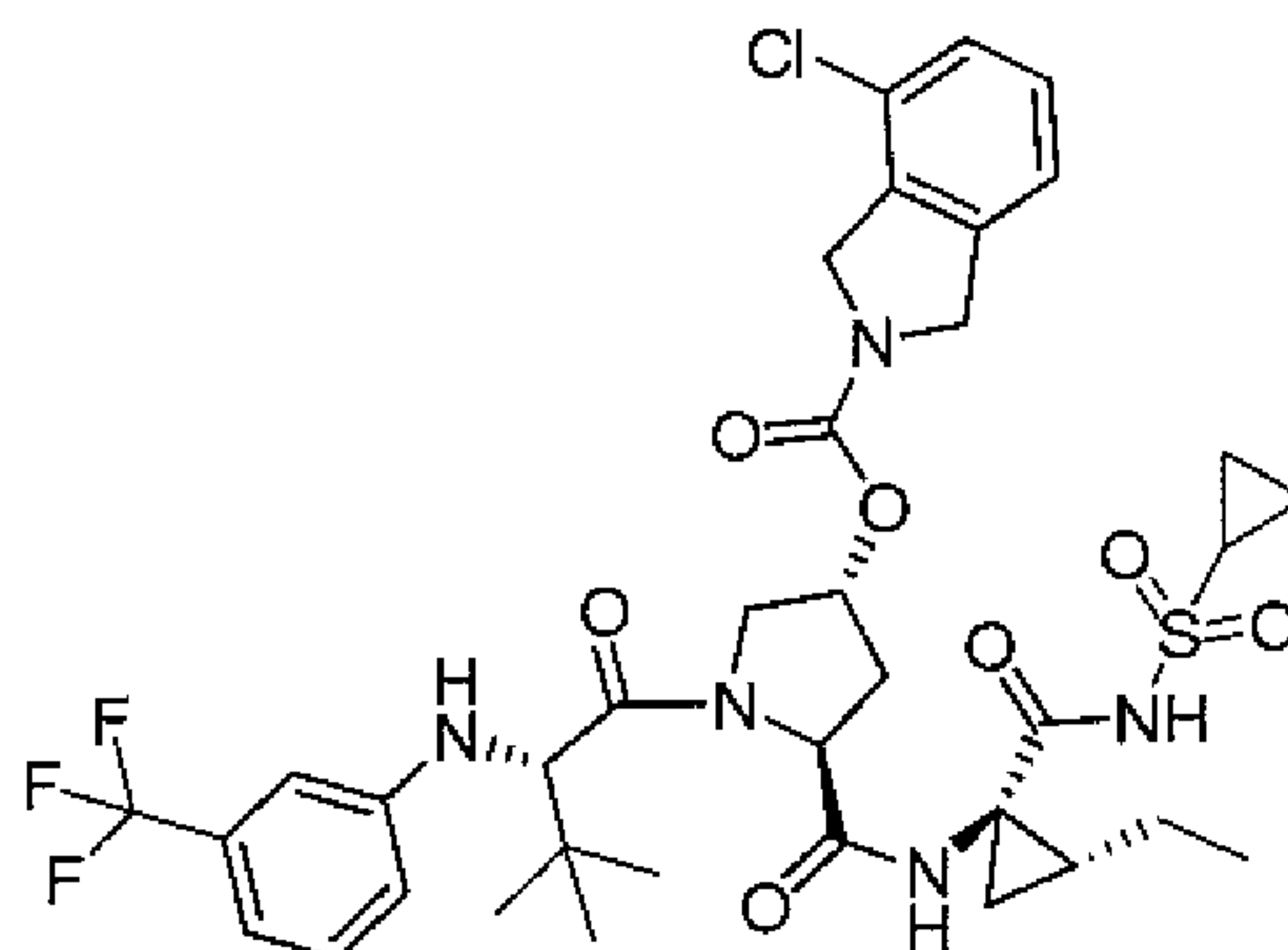
Compound 55
