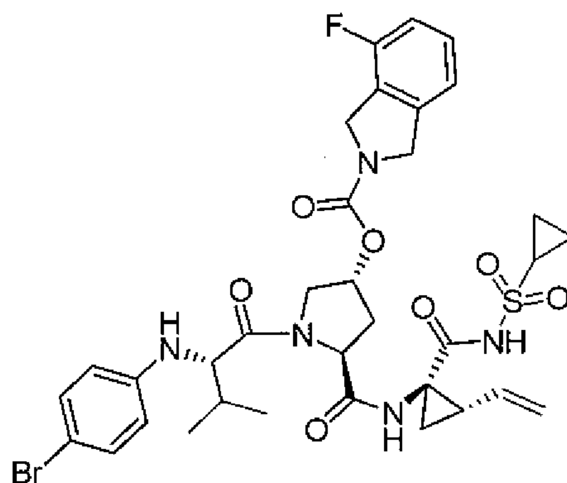
Compound 36
