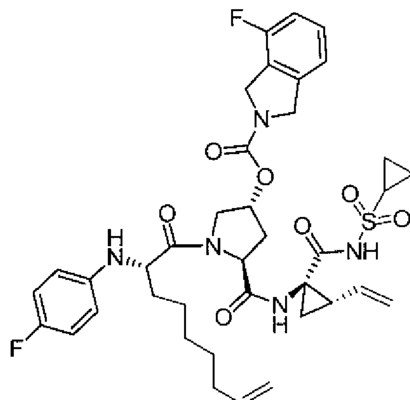
Compound 35
