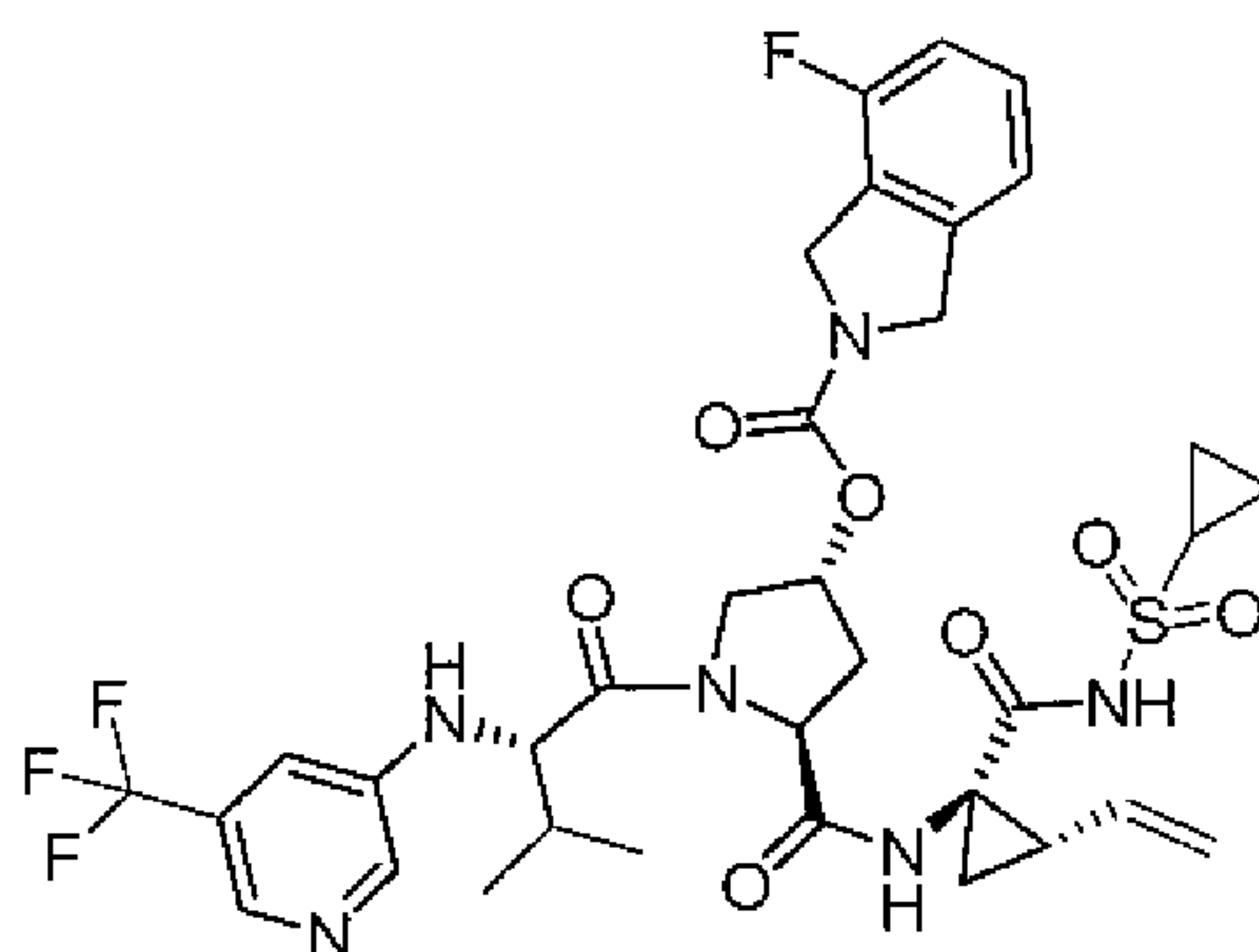
Compound 44
