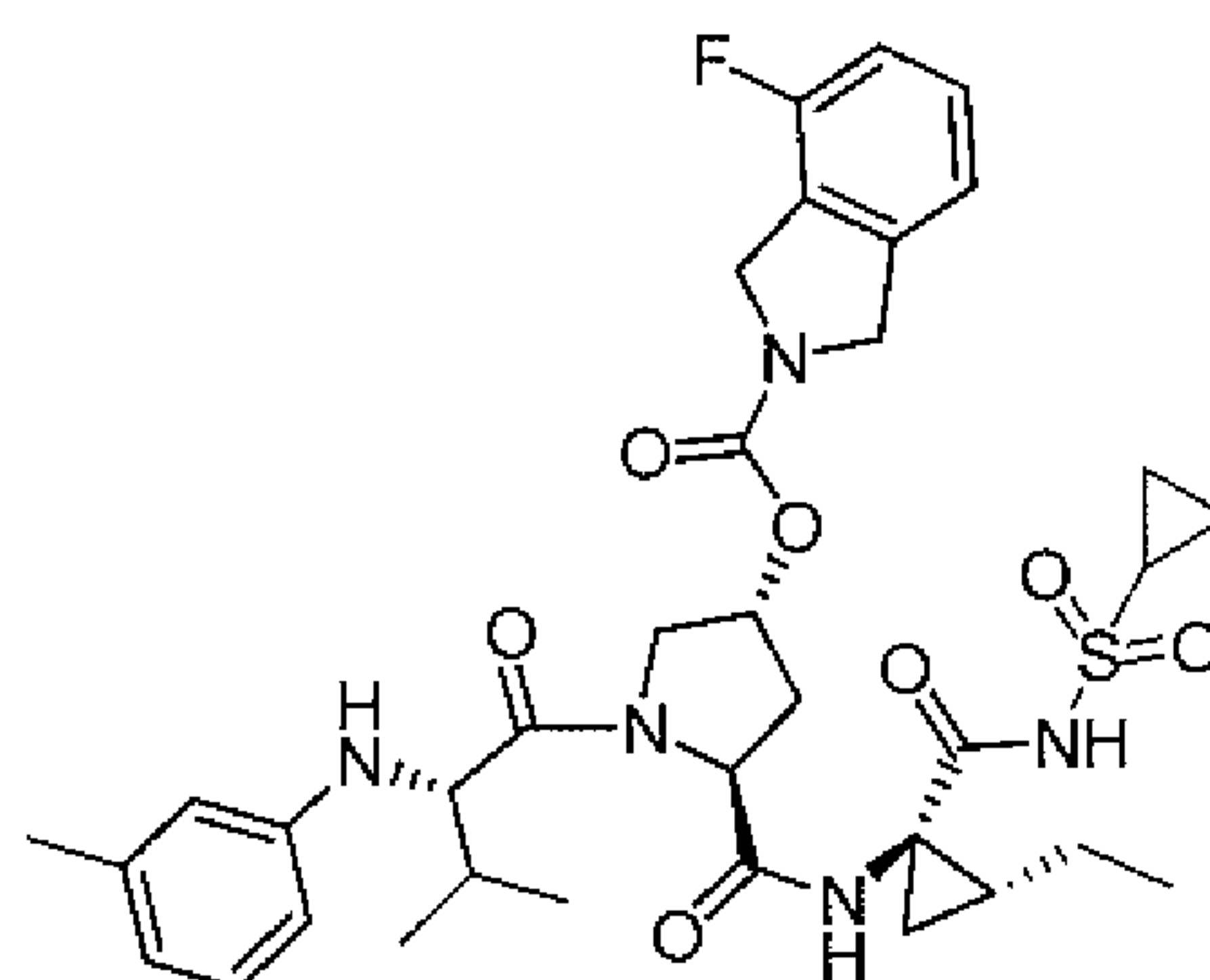
Compound 49
