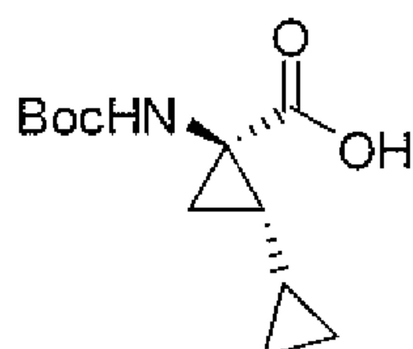
Compound 22
