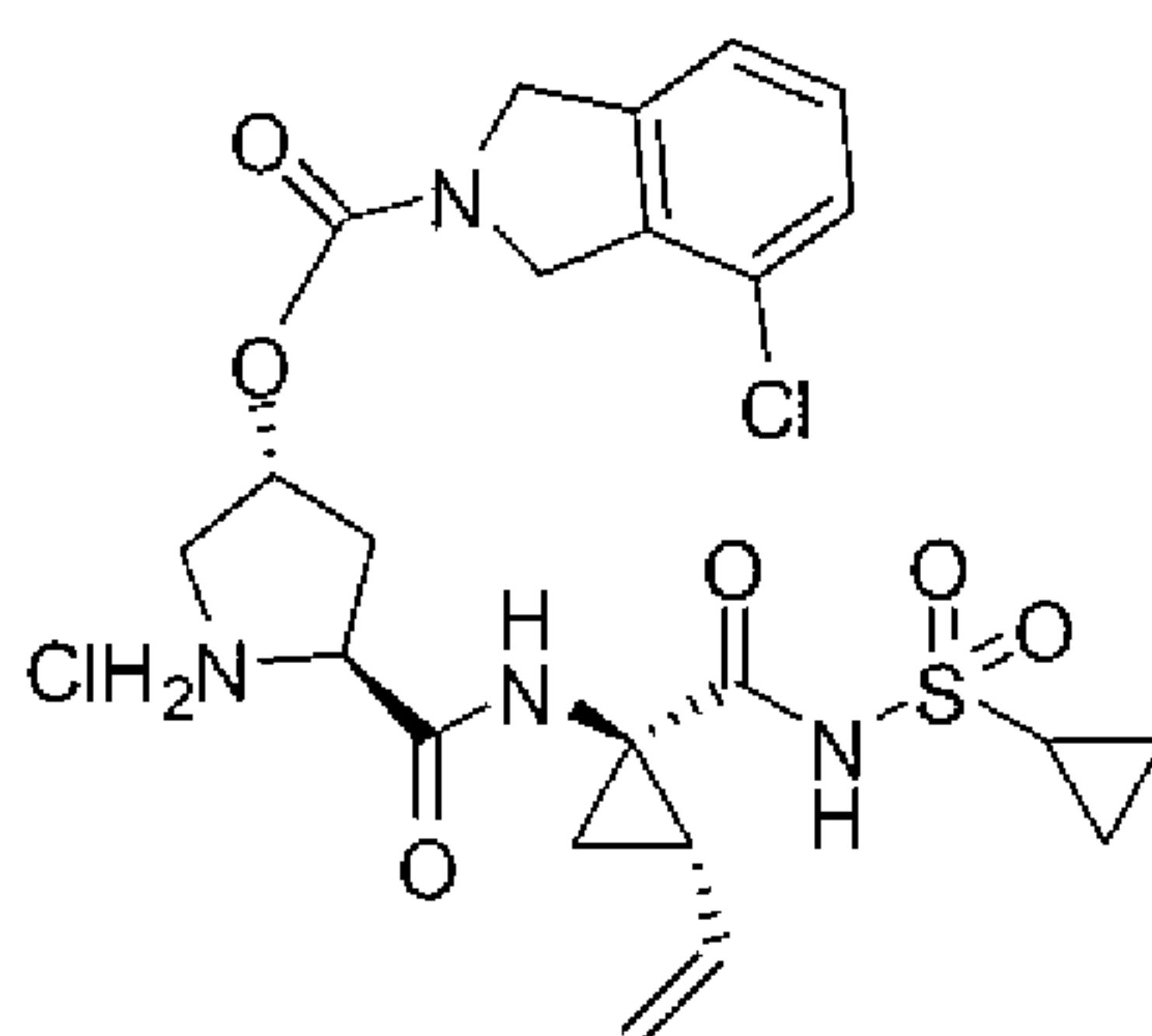
Compound 31
