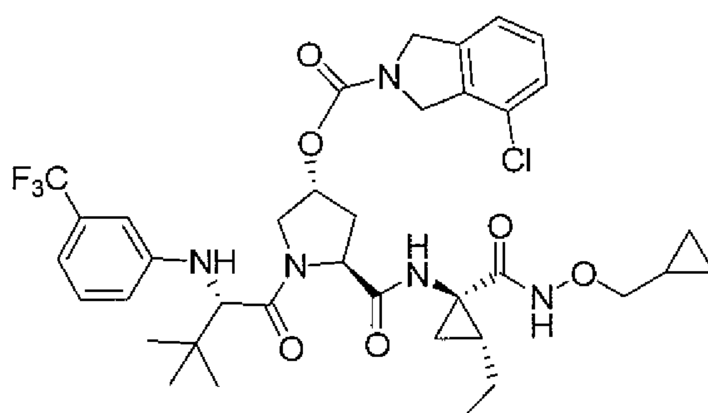
Compound 72
