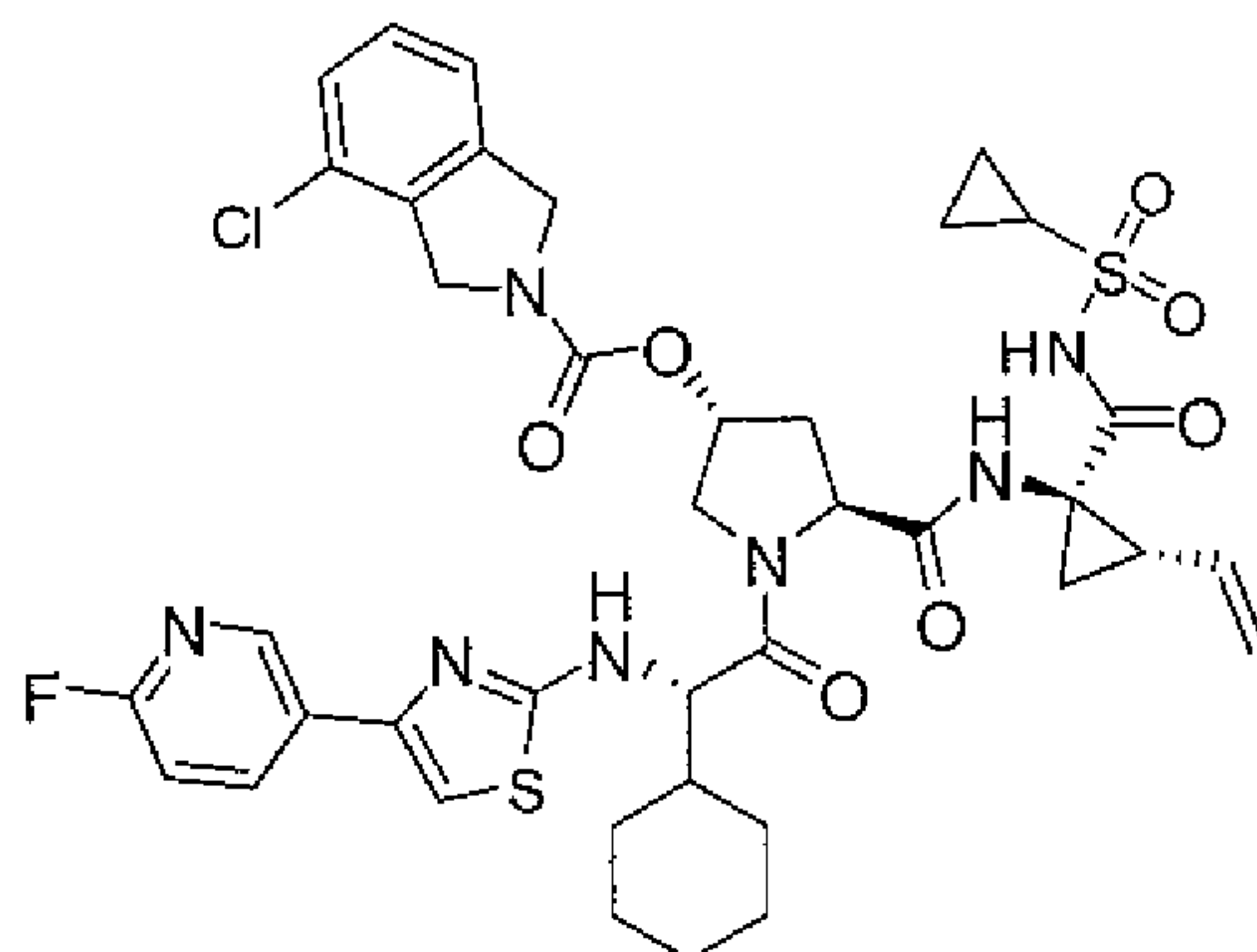
Compound 61
