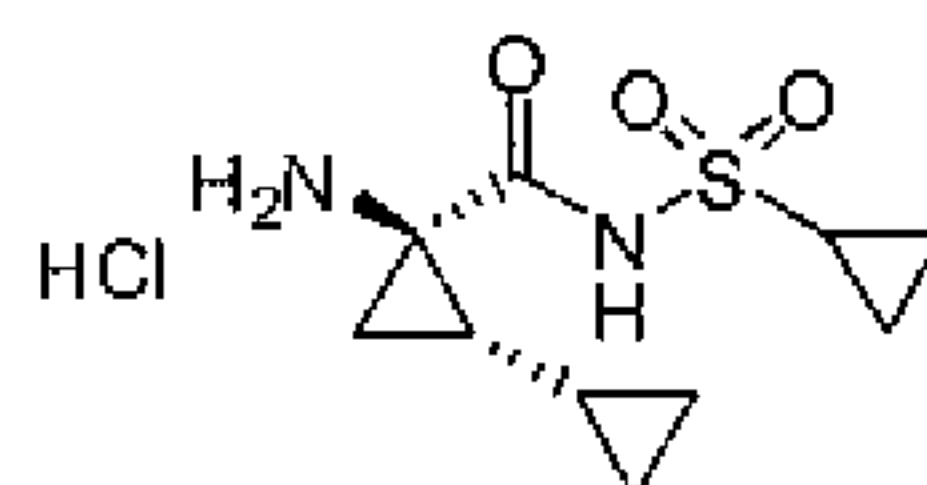
Compound 25
