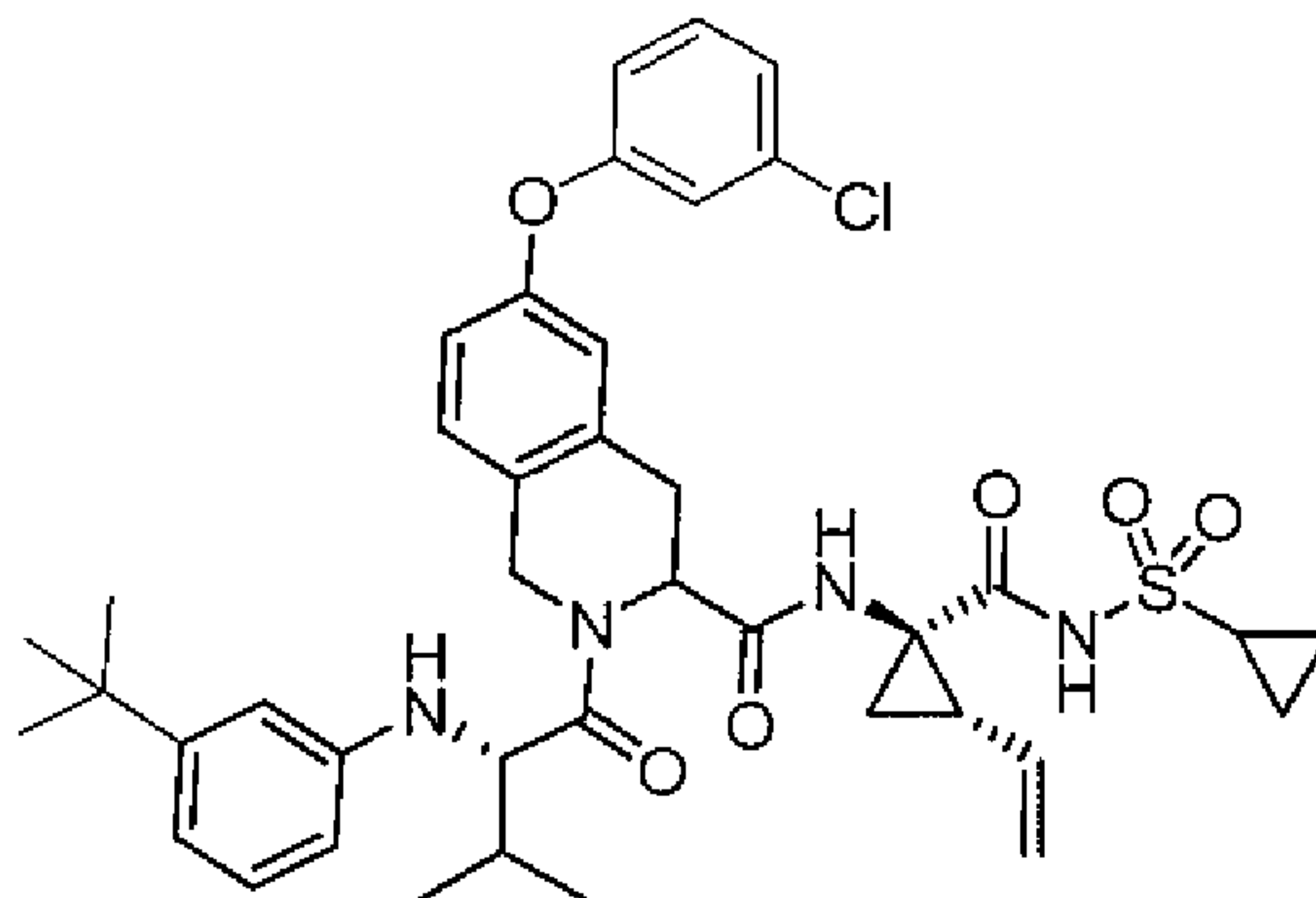
Compound 13
