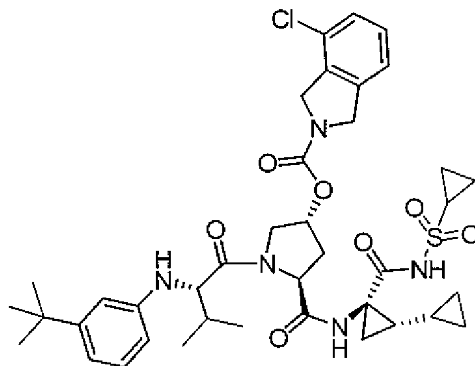
Compound 59
