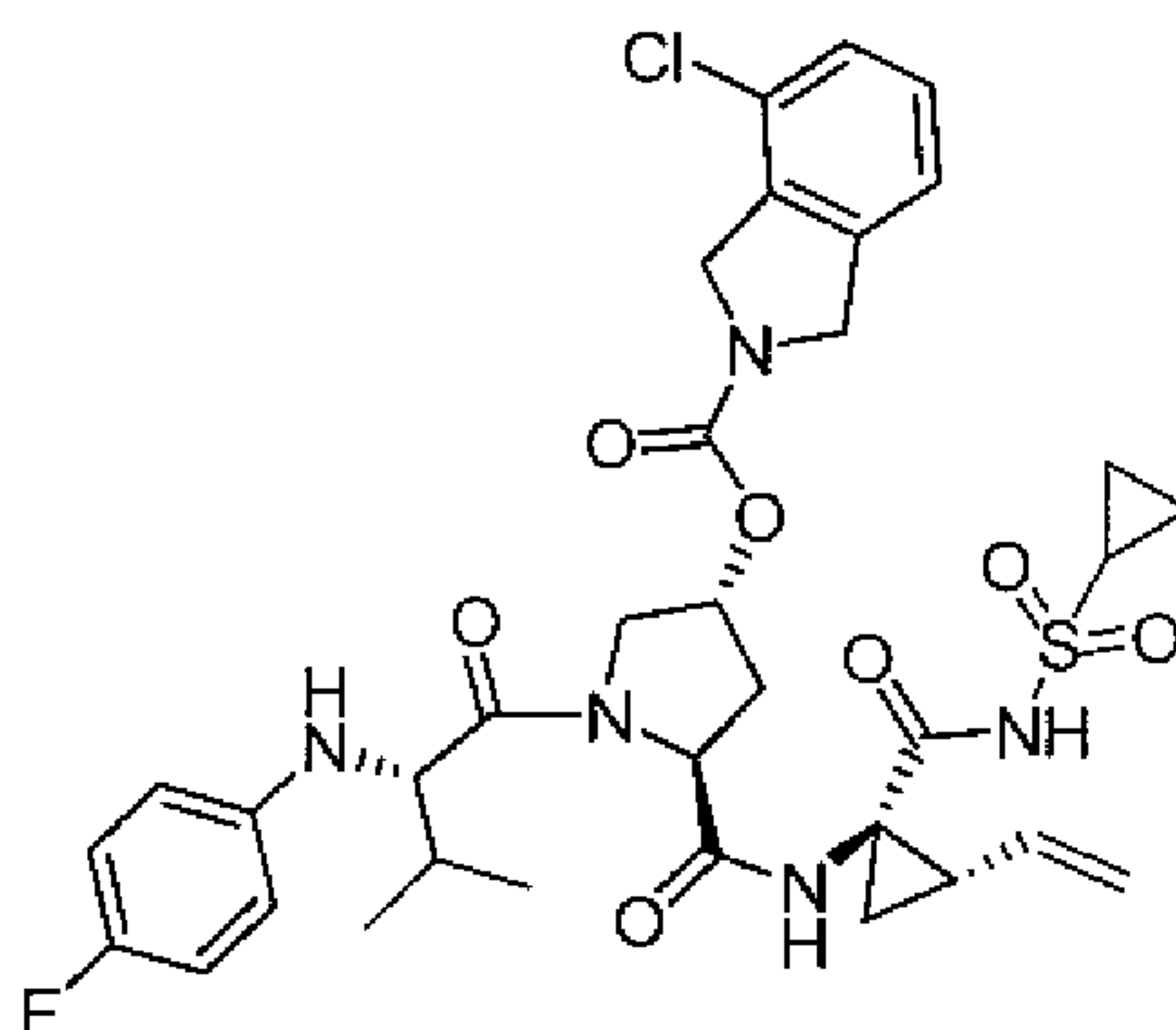
Compound 34
