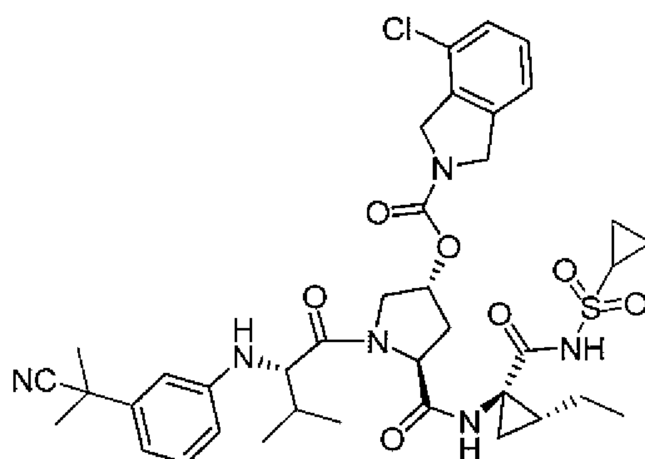
Compound 54
