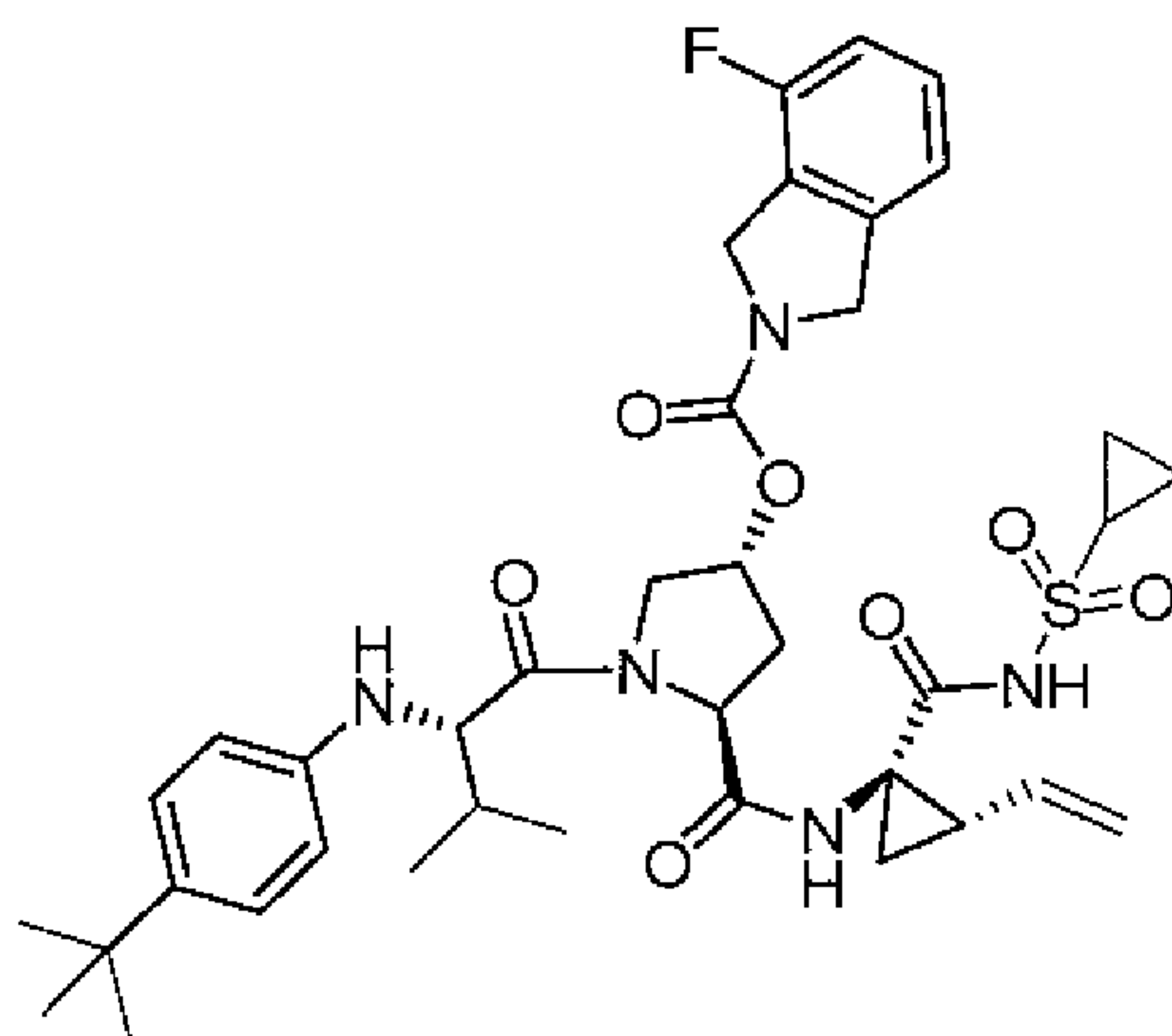
Compound 38
