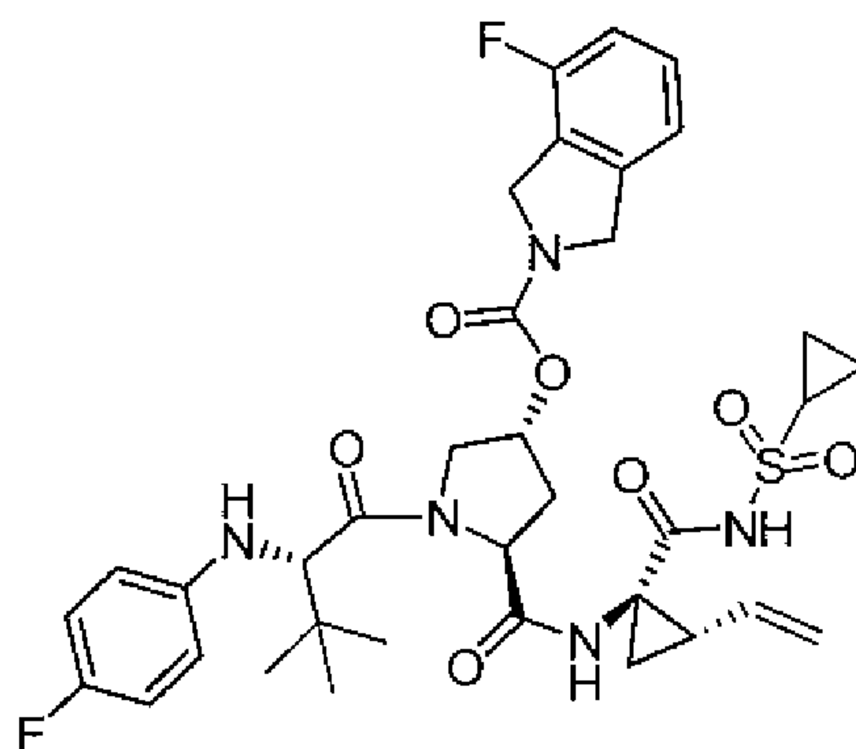
Compound 37
