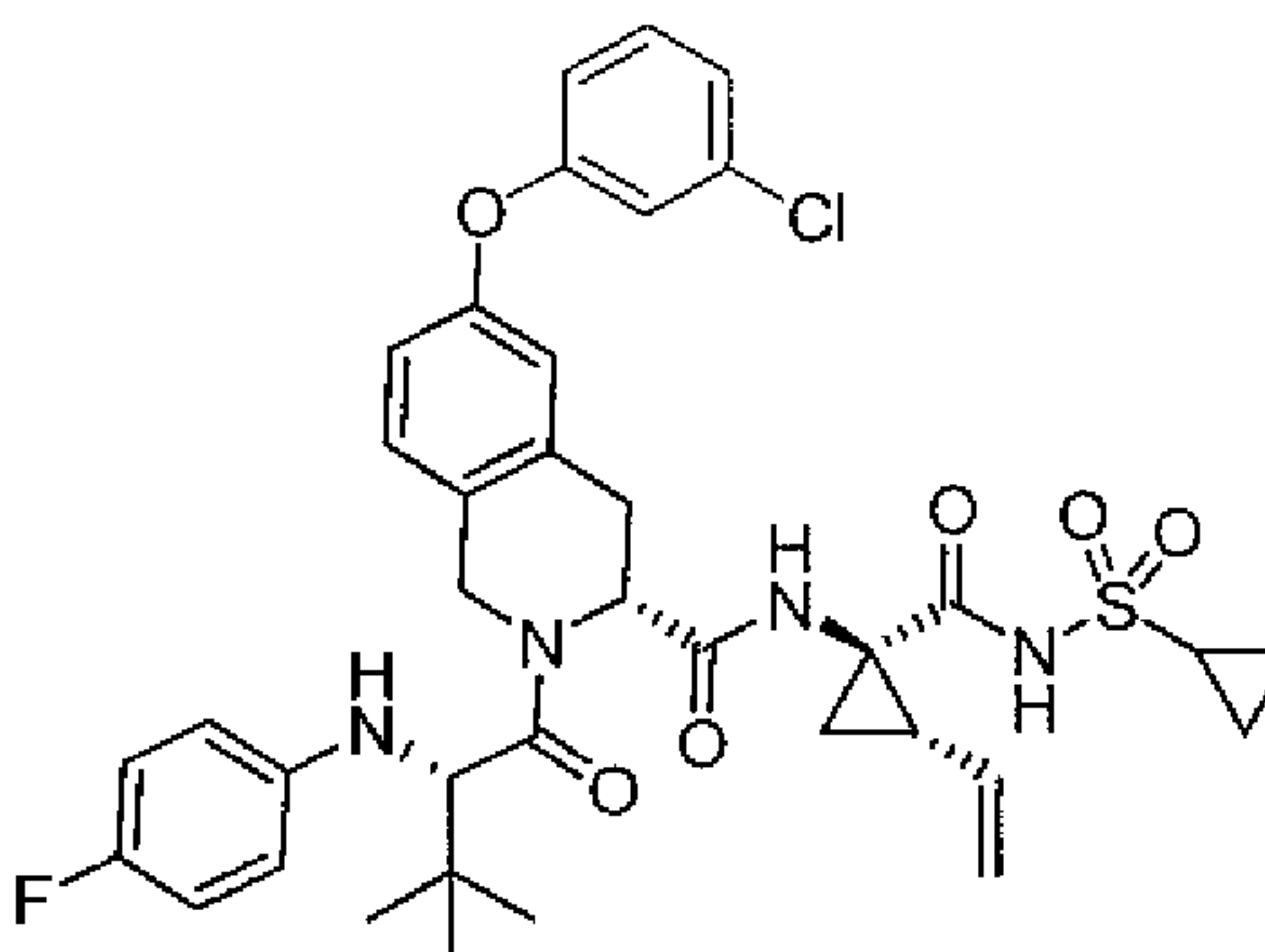
Compound 12
