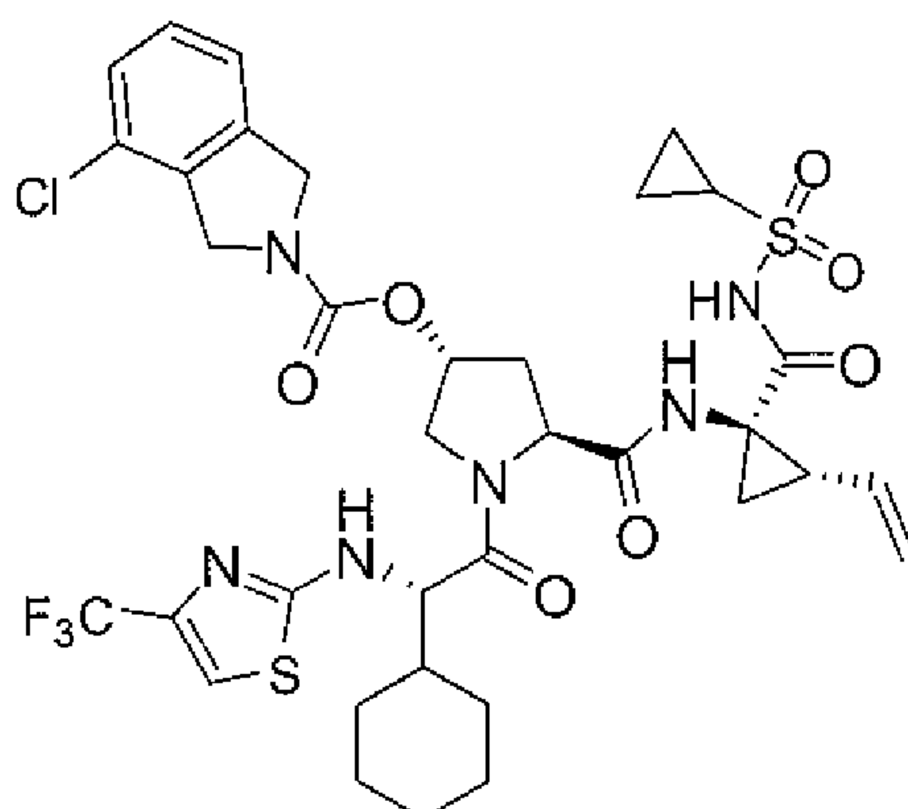
Compound 63
