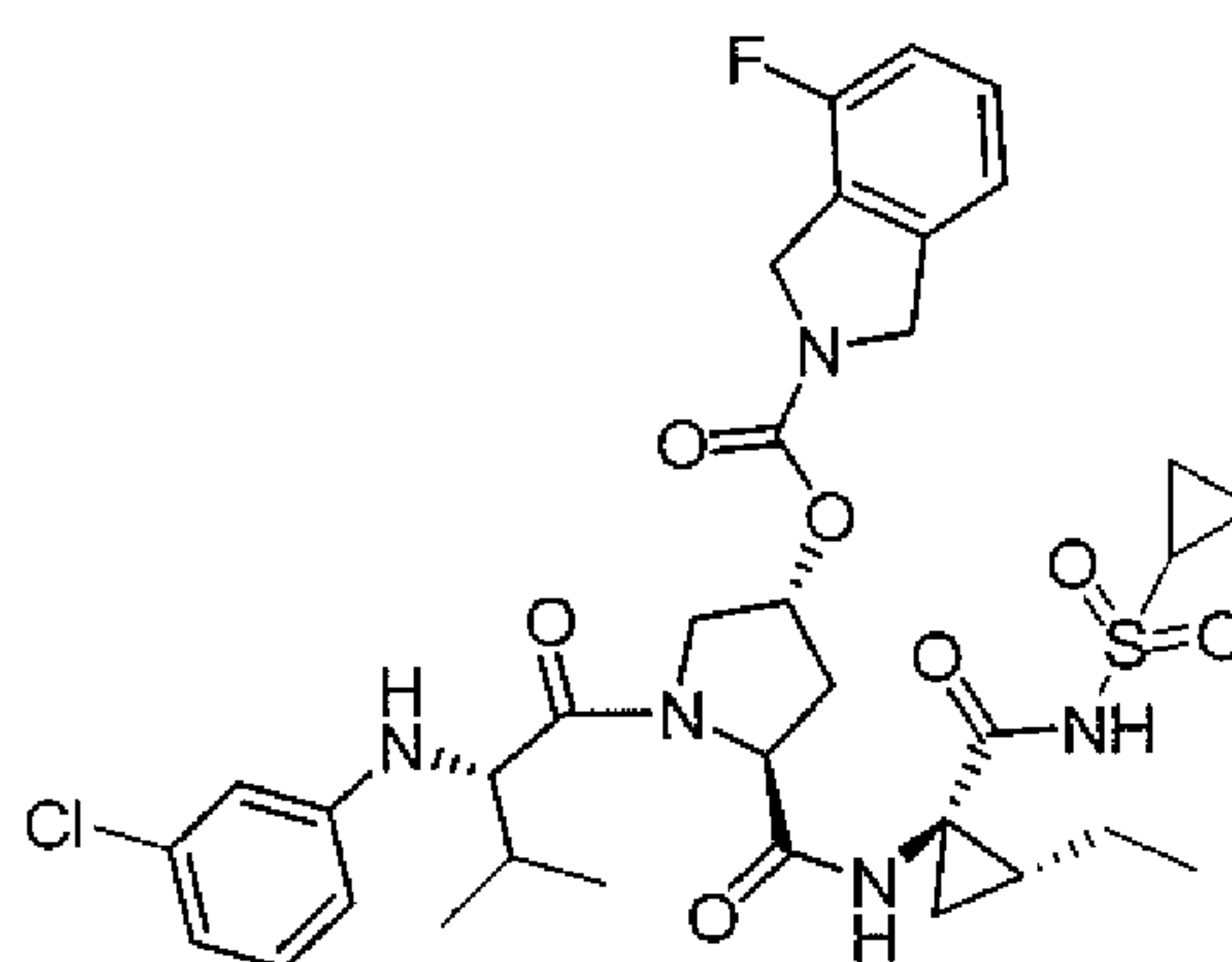
Compound 50
