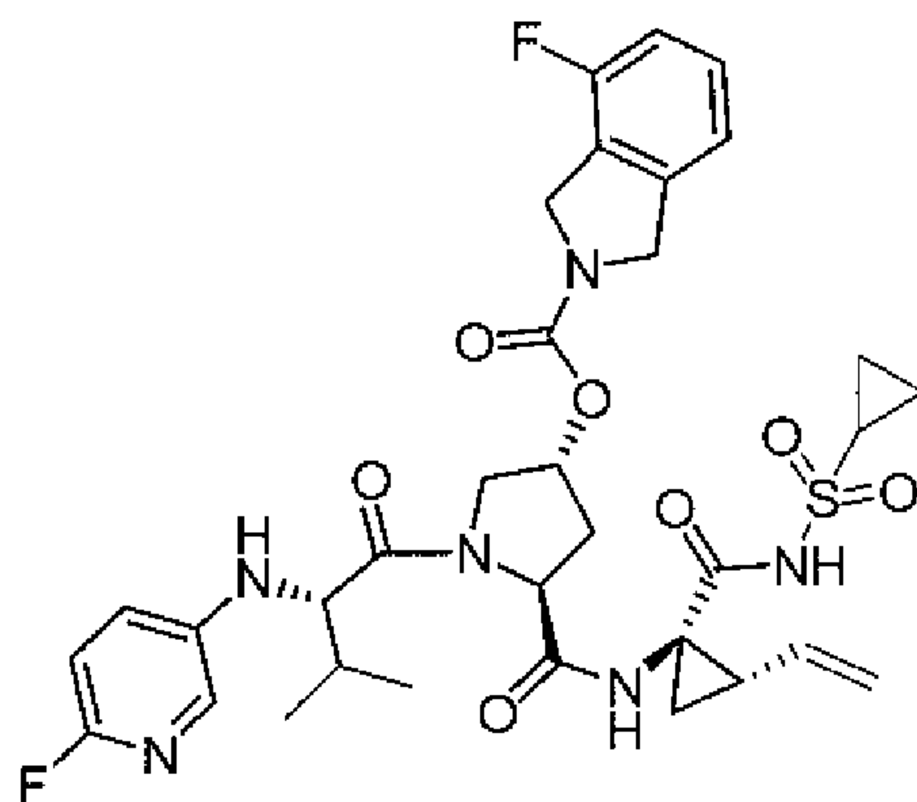
Compound 39
