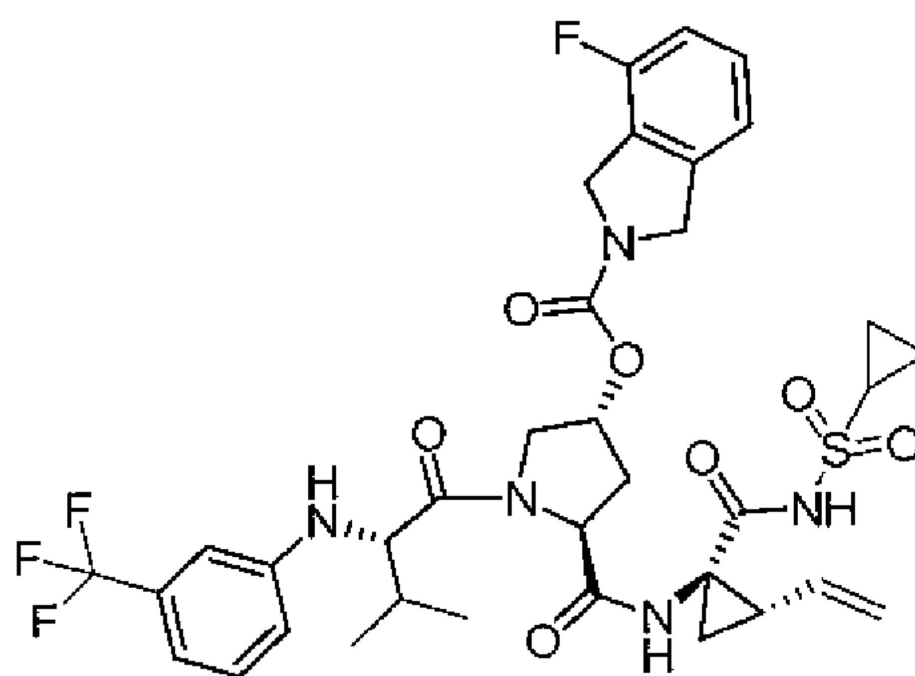
Compound 42
