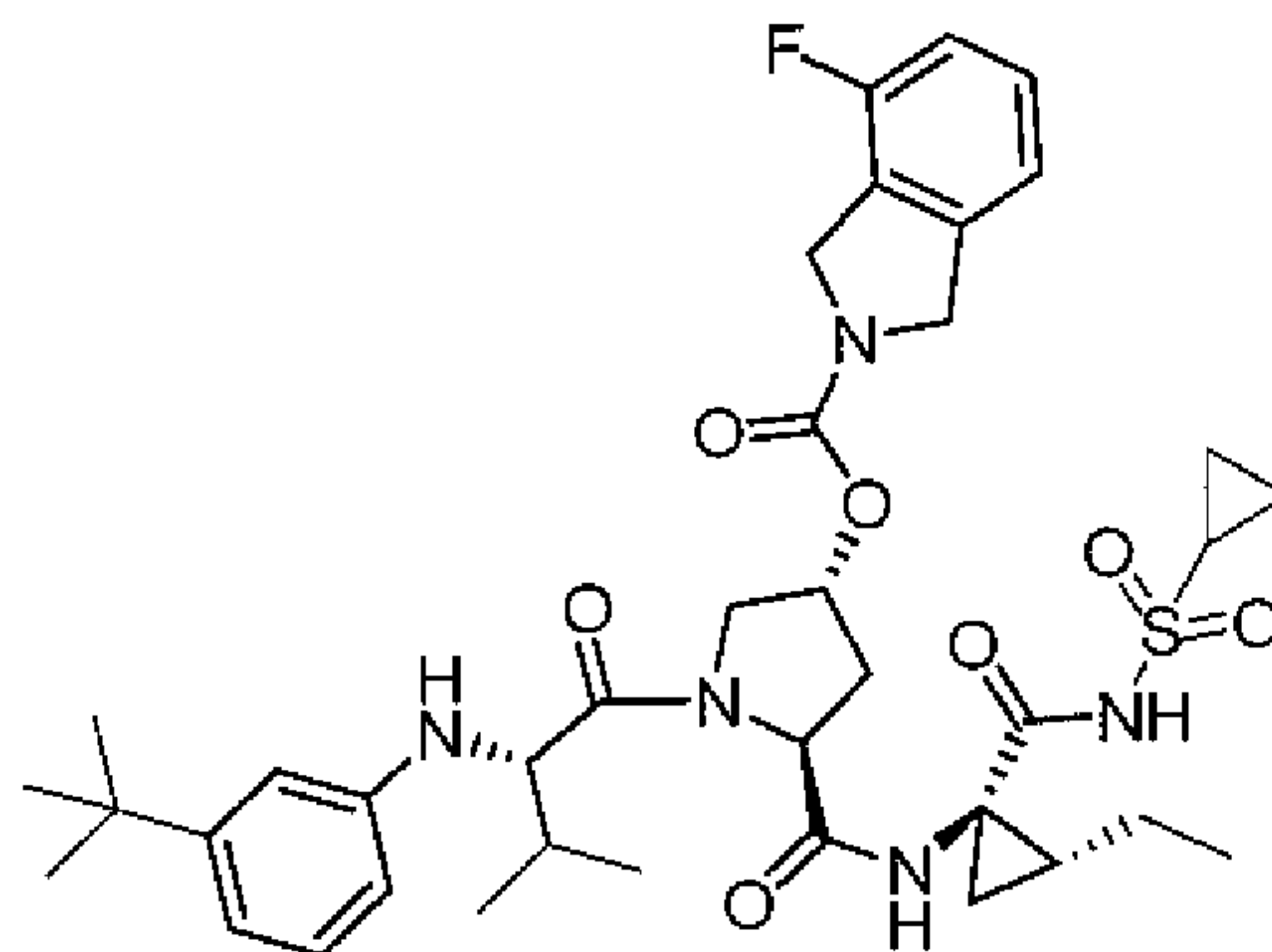
Compound 45
