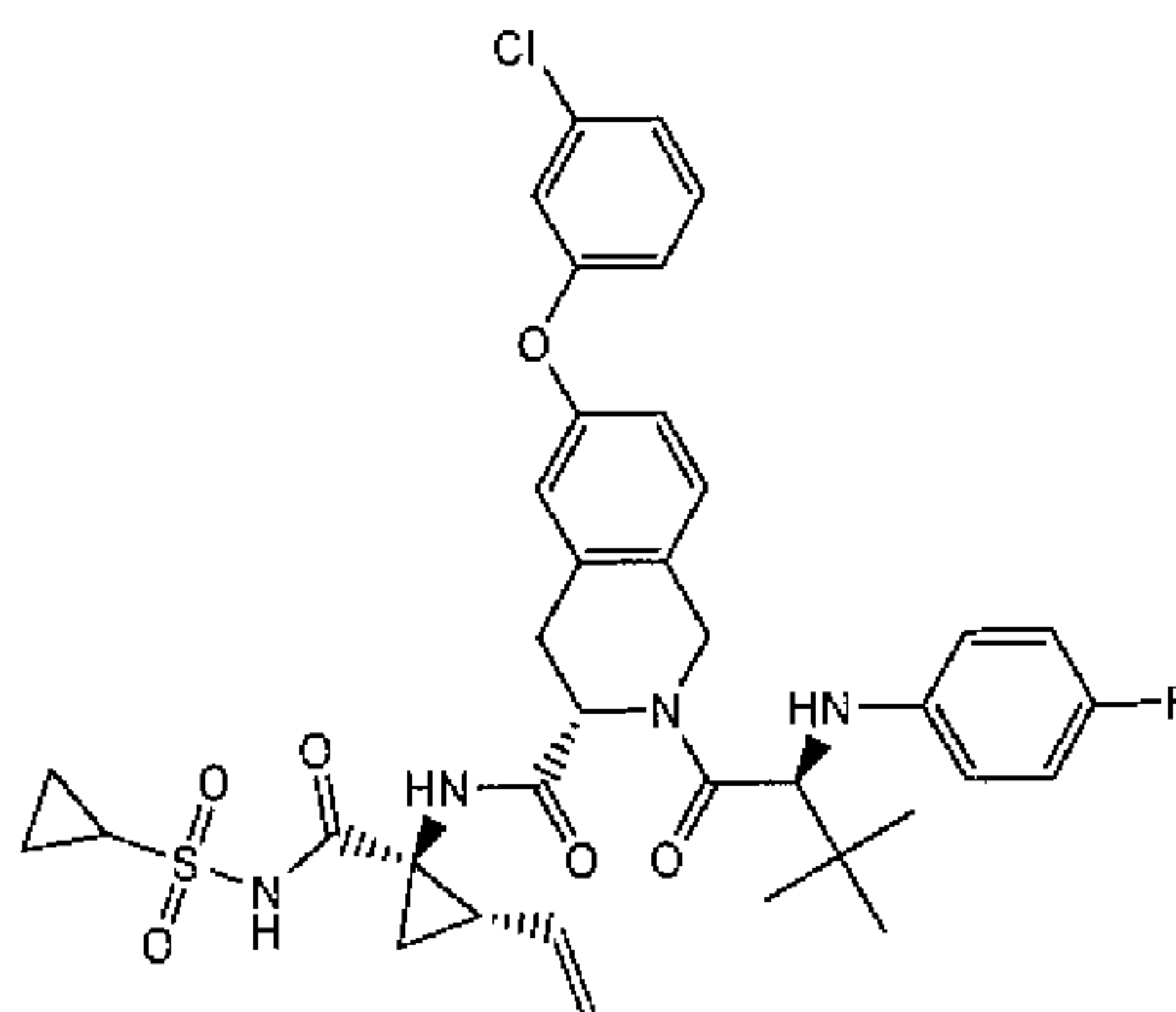
Compound 14
