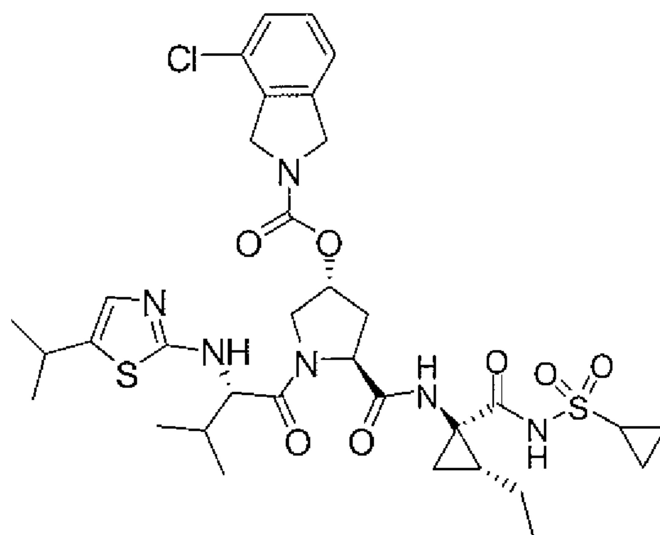
Compound 67
