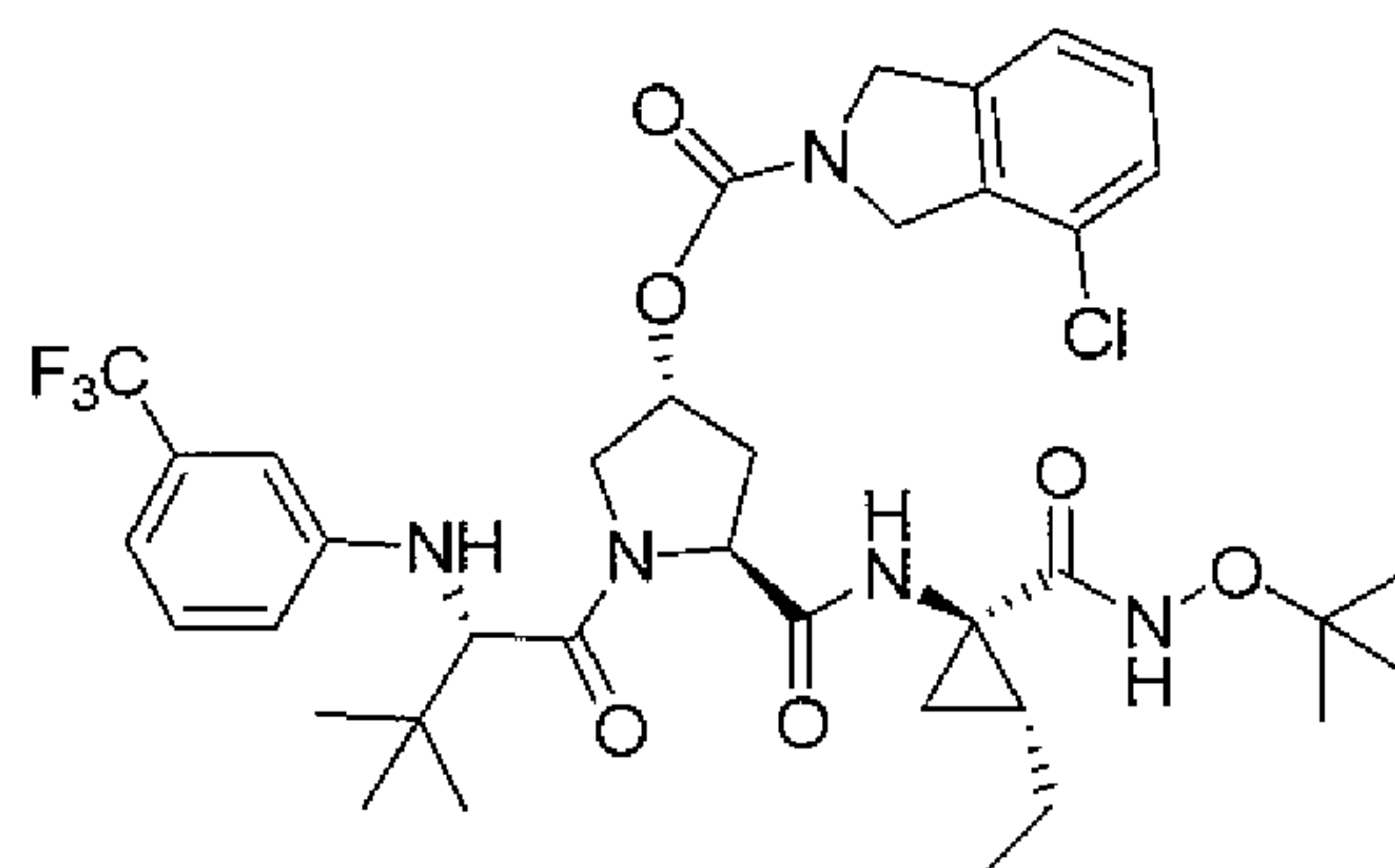
Compound 71
