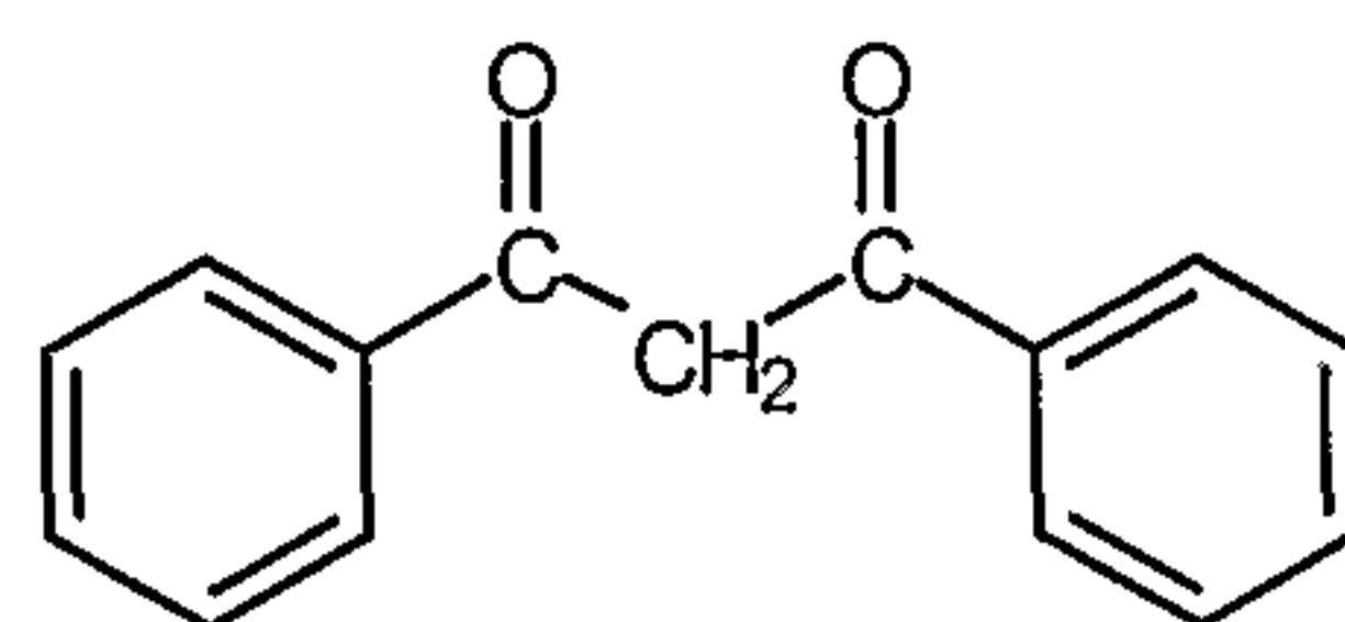
Dibenzoylmethane
