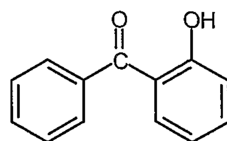
2-Hydroxybenzophenone
