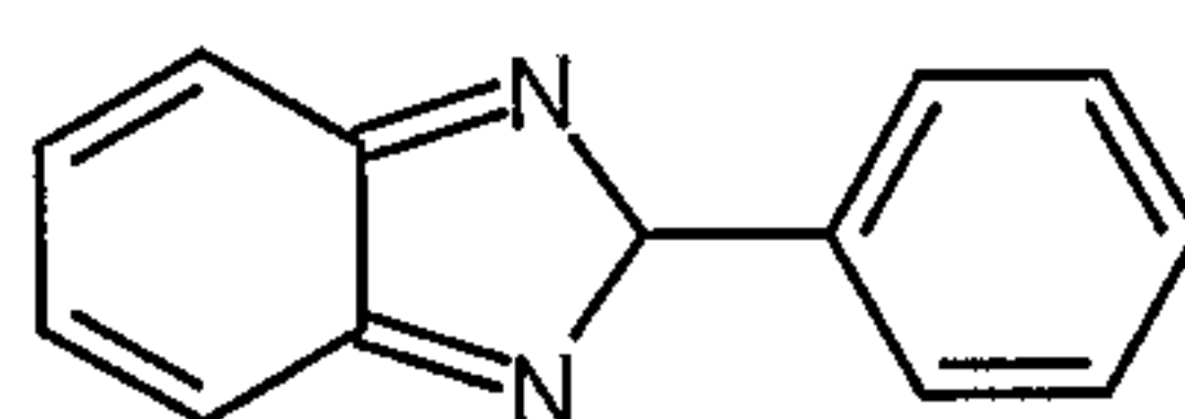
Phenylbenzimidazole
