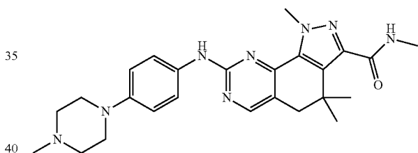
Milciclib Chemical Structure Molecular Weight: 460.57
