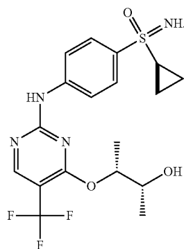
BAY 1000394 Chemical Structure Molecular Weight: 430.44
