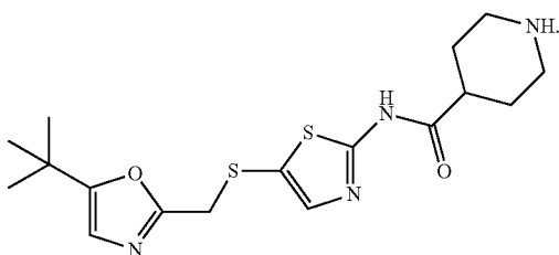
SNS032 Chemical Structure Molecular Weight: 380.53
