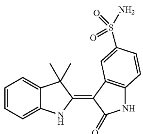
ZK-304709 Chemical Structure Molecular Weight: 355.41
