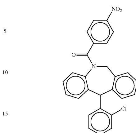
NC381 Chemical Structure Molecular Weight: 454
