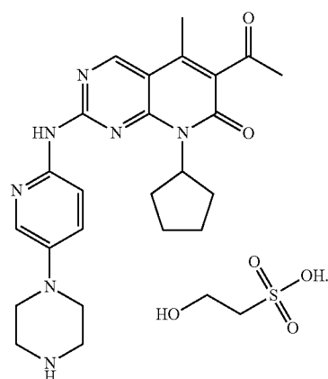
PD0332991/palbociclib Chemical Structure Molecular Weight: 573.66
