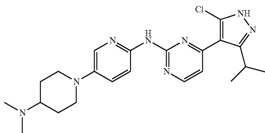
C_{22}H_{29}ClN_8 Mol. Wt.: 440.97
