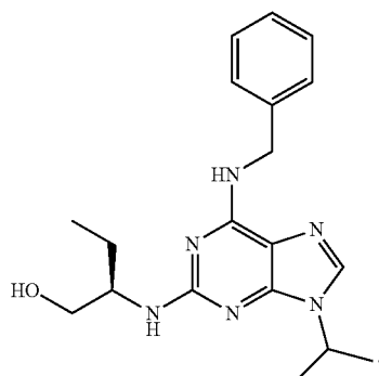
Seliciclib Chemical Structure Molecular Weight: 354.45
