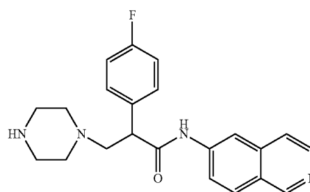
2-(4-fluorophenyl)-N-(isoquinolin-6-yl)-3-(piperazin-1-yl)propanamide
