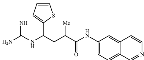
4-guanidino-N-(isoquinolin-6-yl)-2-methyl-4-(thiopen-2-yl)butanamide
