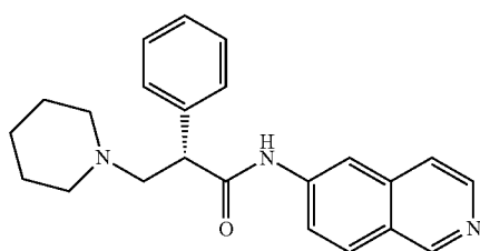
(S)-N-(isoquinolin-6-yl)-2-phenyl-3-(piperidin-1-yl)propanamide
