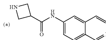
N-(isoquinolin-6- yl)-azetidine-3-carboxamide
