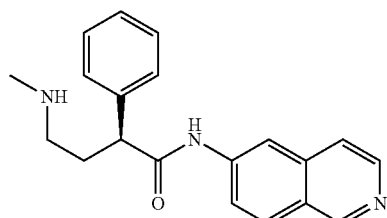
(S)-N-(isoquinolin-6-yl)-4-(methylamino)-2-phenylbutanamide
