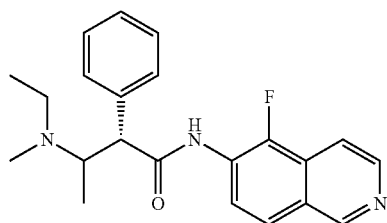
(2S)-3-(ethyl(methyl)amino)-N-(5-fluoroisoquinolin-6-yl)-2-phenylbutanamide
