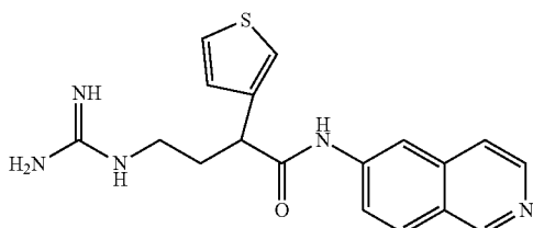
4-guanidino-N-(isoquinolin-6-yl)-2-(thiopen-3-yl)butanamide
