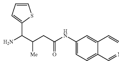
4-amino-N-(isoquinolin-6-yl)-3-methyl-4-(thiopen-2-yl)butanamide
