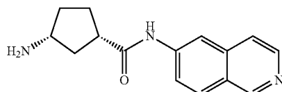
(1S,3R)-3-amino-N-(isoquinolin-6-yl)cyclopentanecarboxamide
