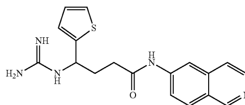
4-guanidino-N-(isoquinolin-6-yl)-4-(thiopen-2-yl)butanamide
