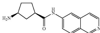
(1R,3S)-3-amino-N-(isoquinolin-6-yl)cyclopentanecarboxamide
