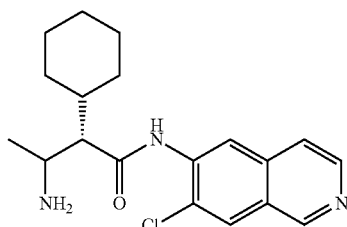
(2S)-3-amino-N-(7-chloroisoquinolin-6-yl)-2-cyclohexylbutanamide
