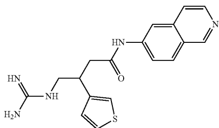
4-guanidino-N-(isoquinolin-6-yl)-3-(thiopen-3-yl)butanamide
