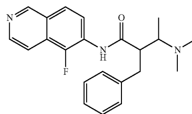
2-benzyl-3-(dimethylamino)-N-(5-fluoroisoquinolin-6-yl)butanamide
