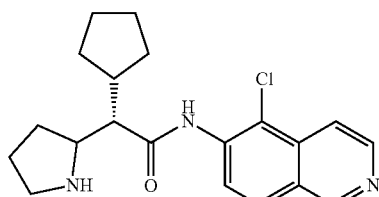
(2S)-N-(5-chloroisoquinolin-6-yl)-2-cyclopentyl-2-(pyrrolidin-2-yl)acetamide
