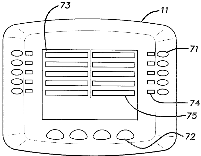
USER INTERFACE UNIT FOR MICRO-PROCESSOR CONTROLLED TIME DOMAIN SWITCHING SYSTEM FOR CONTROL OF POOL AND SPA LIGHTING FIXTURES AND AUXILIARY EQUIPMENT
