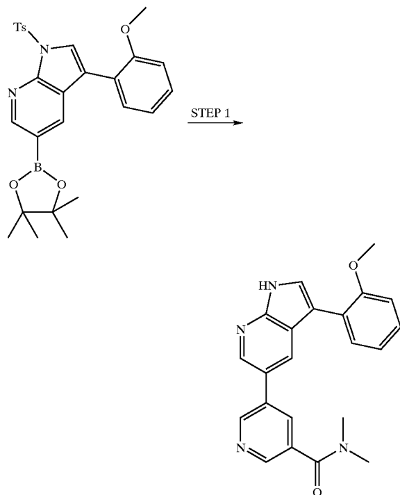
Step 1: Synthesis of 5-[3-(2-Methoxy-phenyl)-1H-pyrrolo[2,3-b]pyridin-5-yl]-N,N-dimethyl-nicotinamide.
