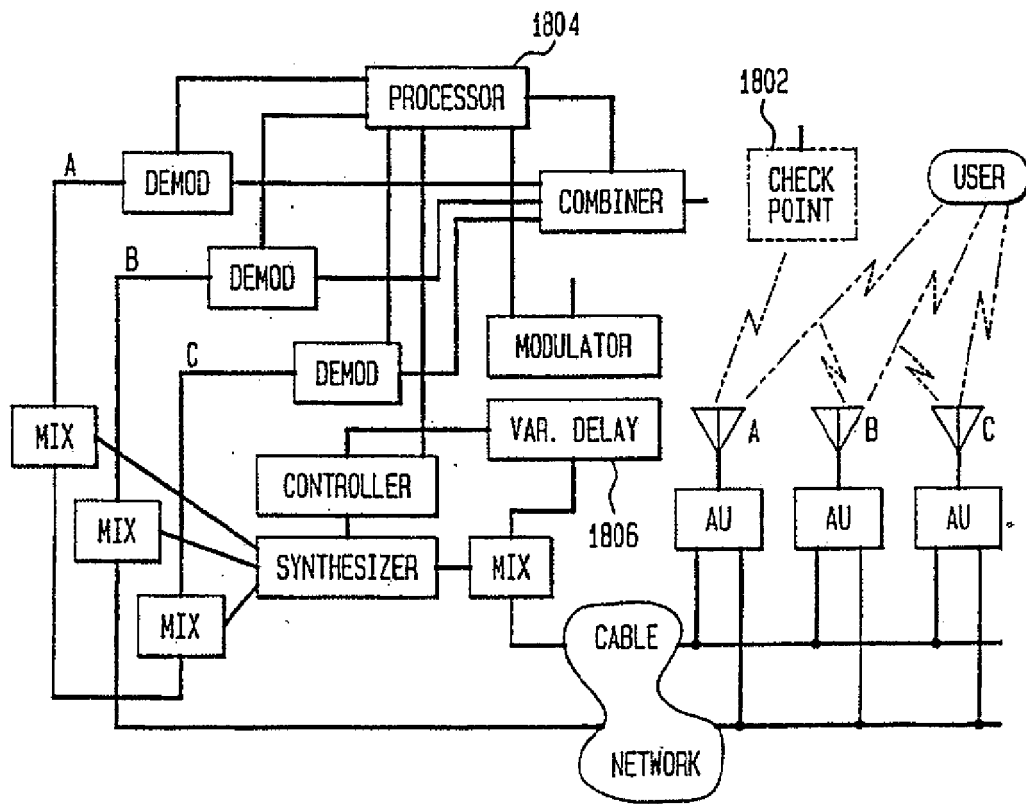
FIG. 18 TIME CALIBRATION FOR DISTRIBUTED ANTENNA IMPLEMENTATION
