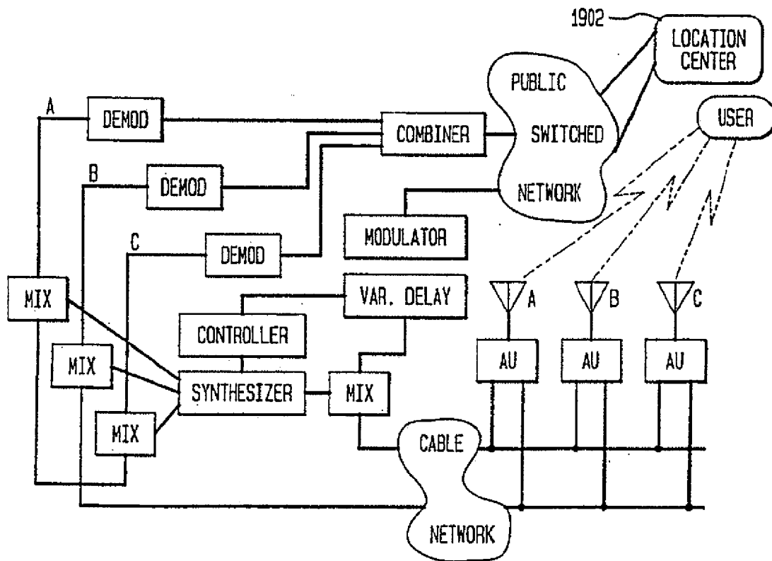
FIG. 19 LOCATION CENTER EXTERNAL TO COMMUNICAITON SYSTEM
