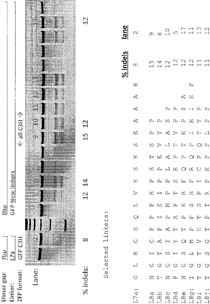
Figure 7: Linkers Selected for 8bp Dimer Gap
