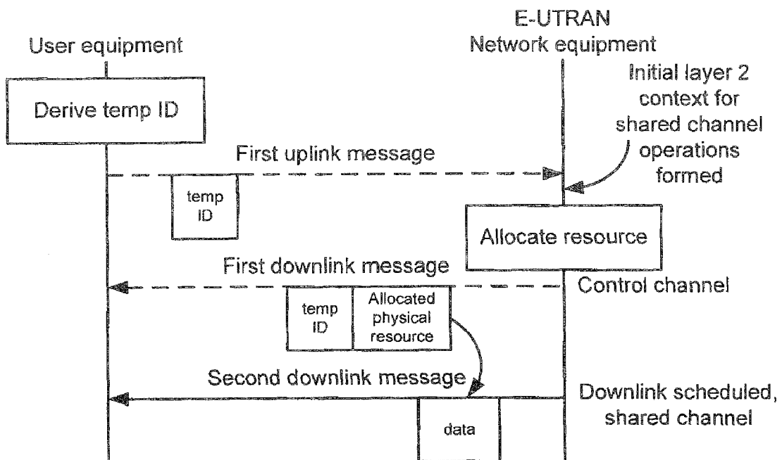
FIGURE 5B
