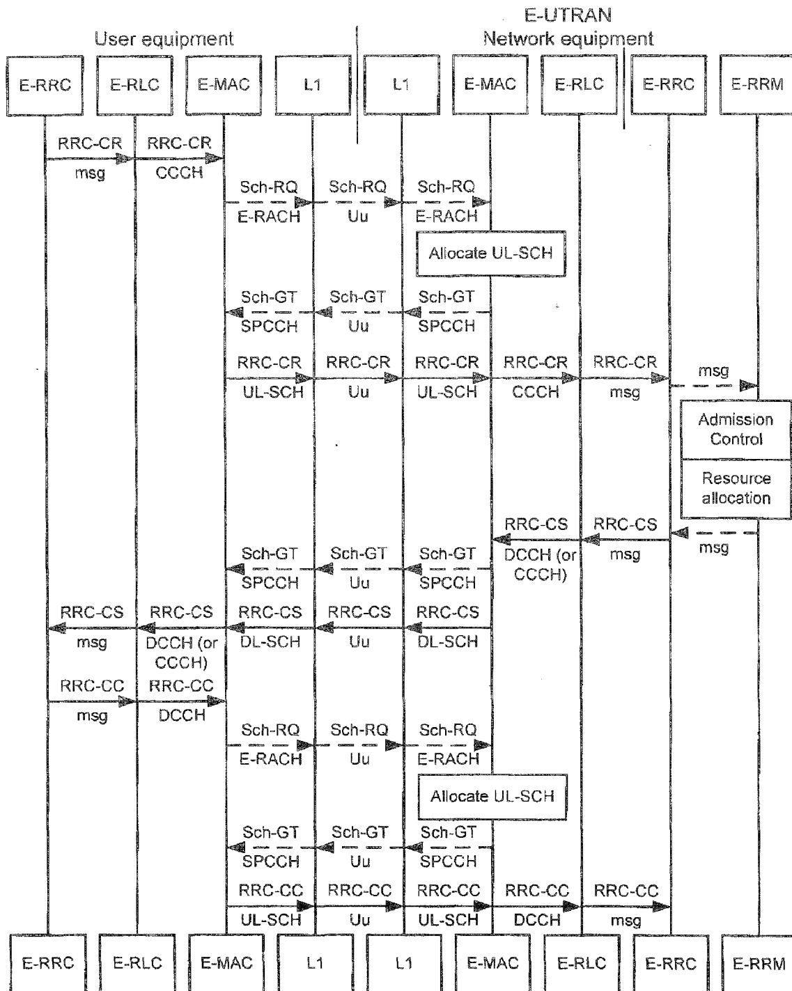
FIGURE 8B
