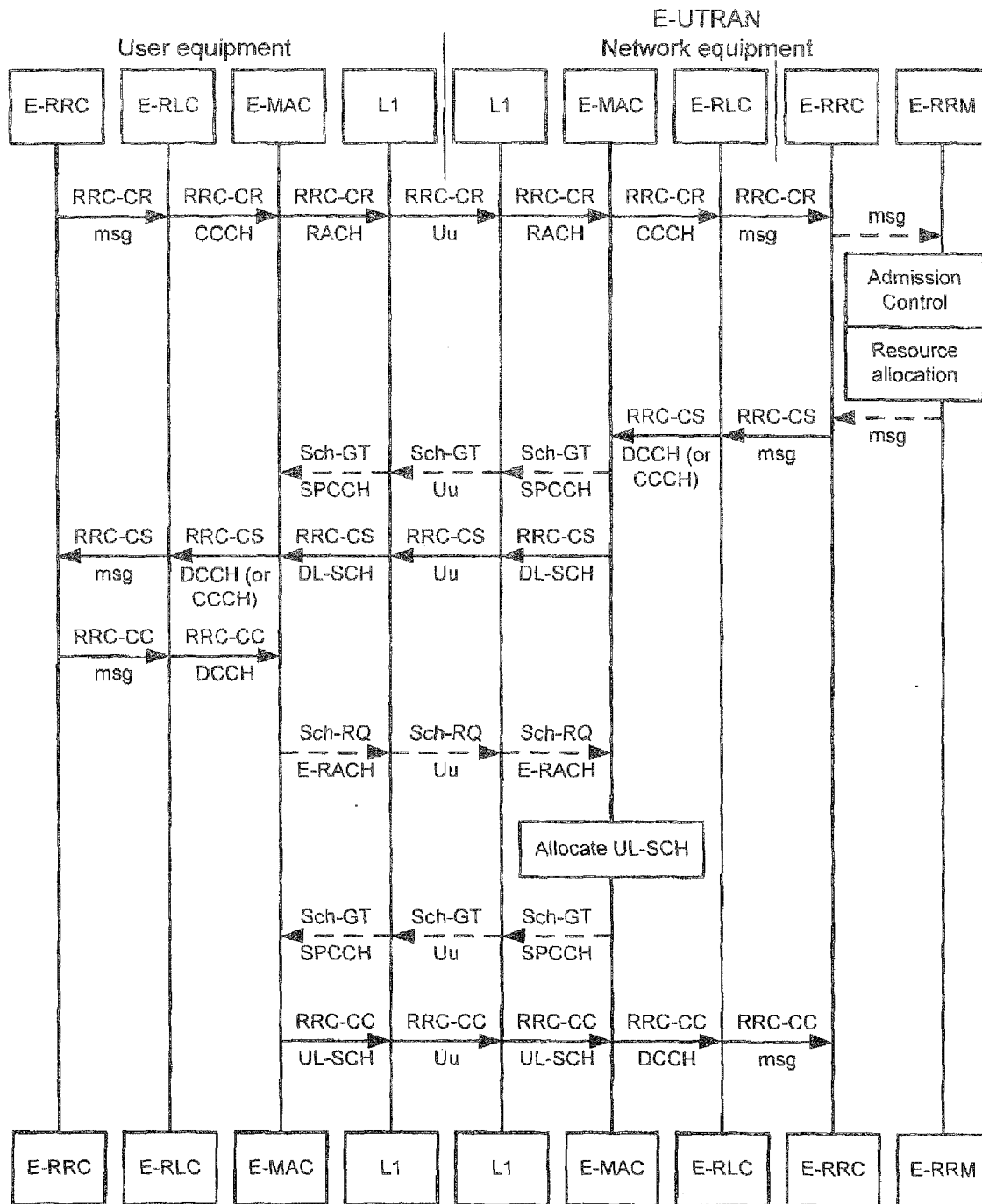
FIGURE 7B
