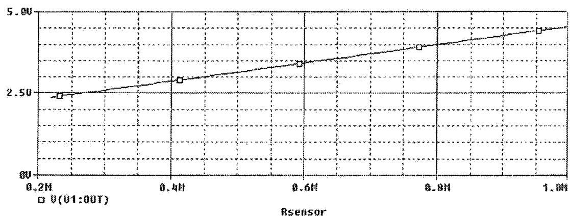
Figure 14: V_{out} vs. R_{sensor}
