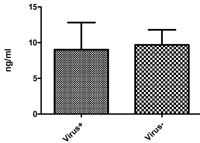
Fig. 19. Virus infection and S100A12 change. P=0.7019 , n=3 (V+), n=19 (V-)
