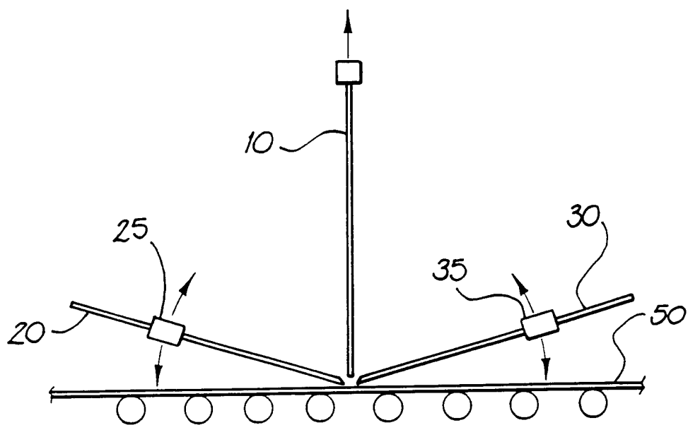
FIG. 2C PRIOR ART
