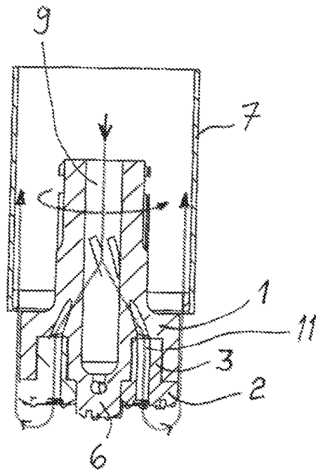
Fig. 9 SECTION B
