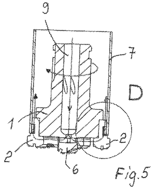
SECTION A
