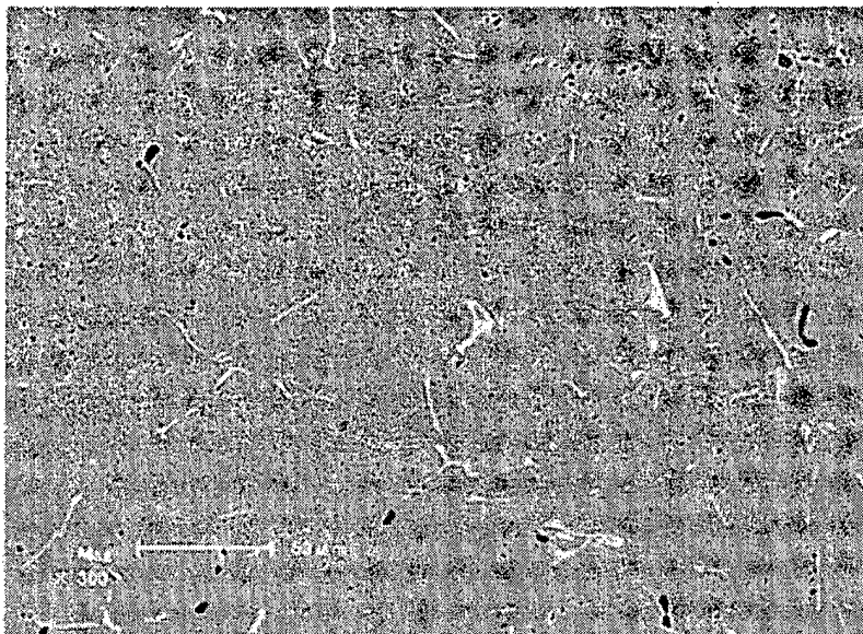
Fig. 3A Billet after homogenization treatment
