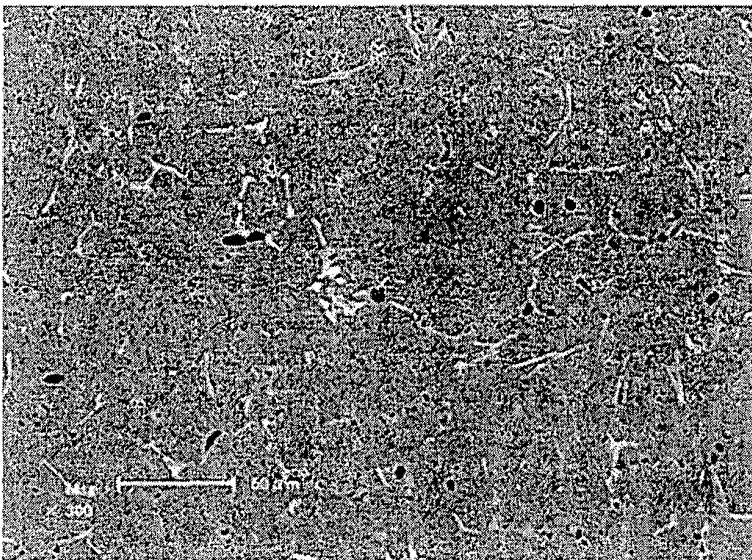
Fig. 4A Billet after homogenization treatment
