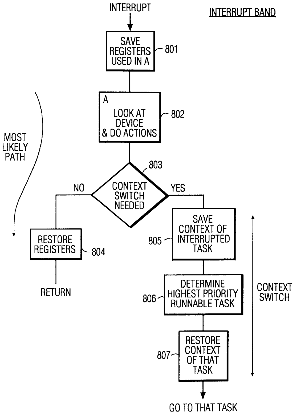
FIG. 8 PRIOR ART
