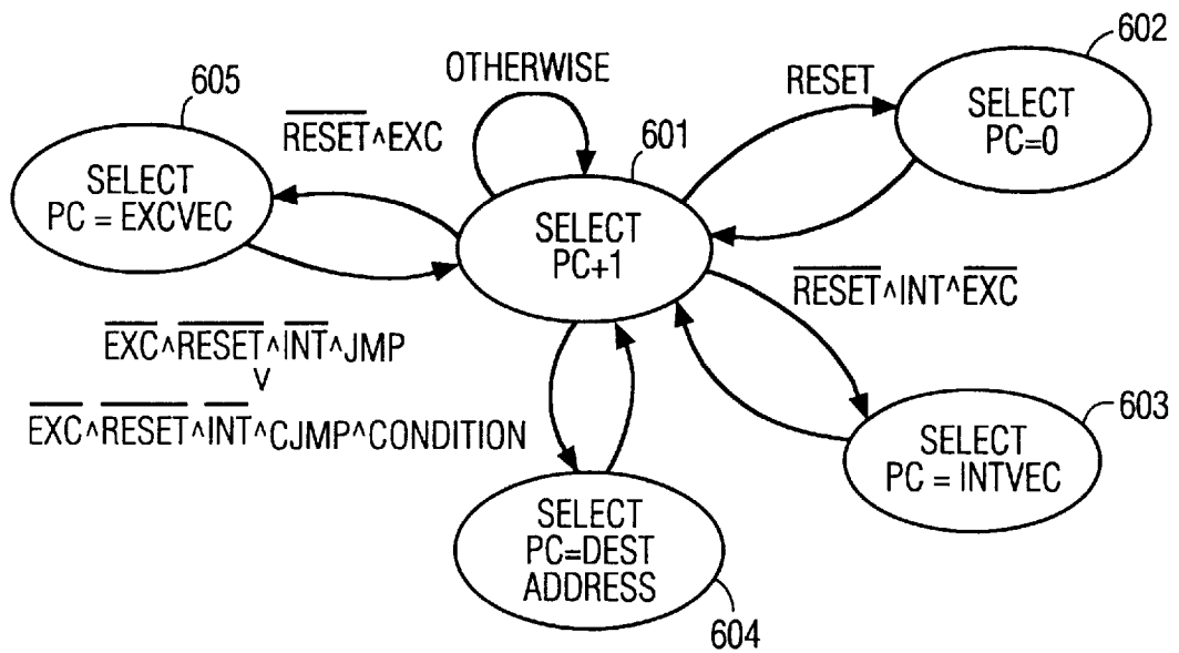
FIG. 6 PRIOR ART
