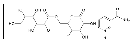
(VIII) Niacinamide Gluconyl Ascorbate or, Gluconyl Niacinamidonium Ascorbate
