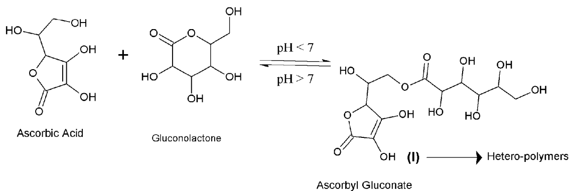
Fig. 2. Process Example of Ascorbyl Esters from Ascorbic Acid & A Natural Sugar Lactone (Gluconolactone)
