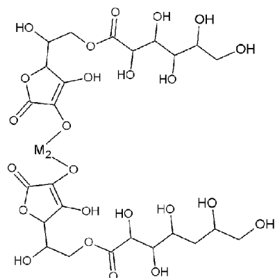
(V) Bis-(Ascorbyl Gluconate) M_2 Salt
