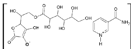
(VII) Niacinamide Ascorbyl Gluconate or, Ascorbyl Niacinamidonium Gluconate
