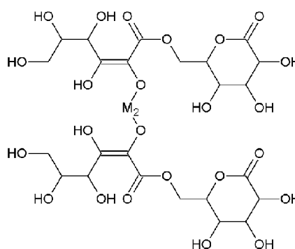
(VI) Bis-(Gluconyl Ascorbate) M_2 Salt
