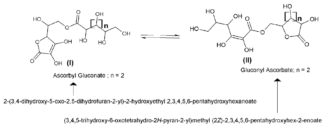
Fig. 3. Isomerism of Ascorbyl Esters
