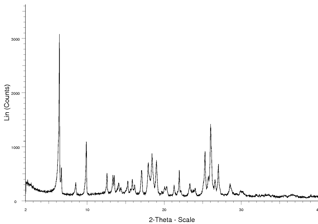
Figure 8 Example 1 esylate salt PXRD
