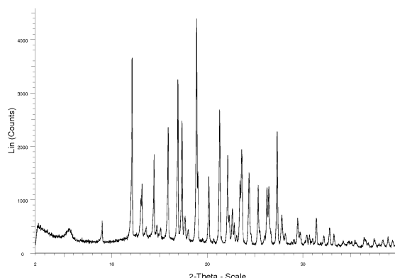
Fig 1 Free molecule (no salt) Example 1 PXRD
