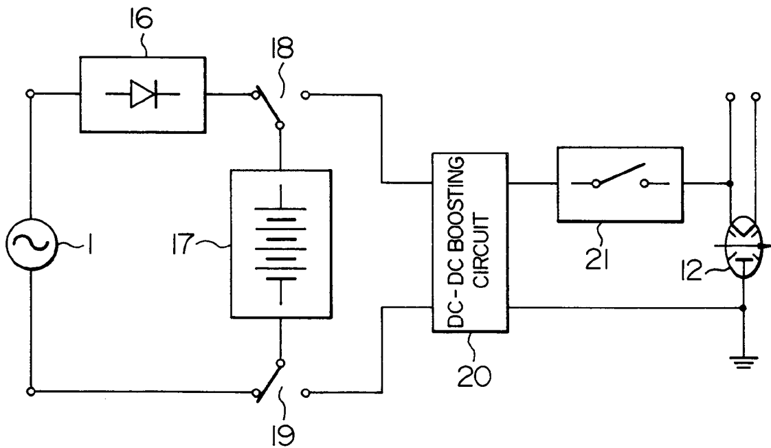
FIG. 14 PRIOR ART
