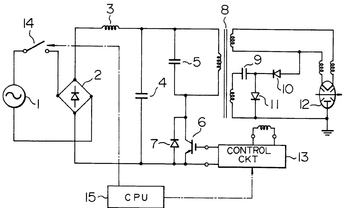
FIG. 12 PRIOR ART
